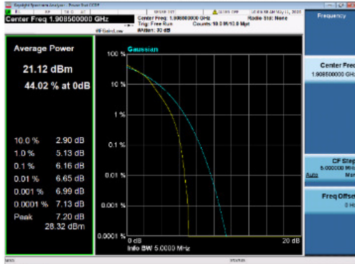
Peak-Average Ratio LTE_2_LTE_HCH_1908.5MHz_NTNV
