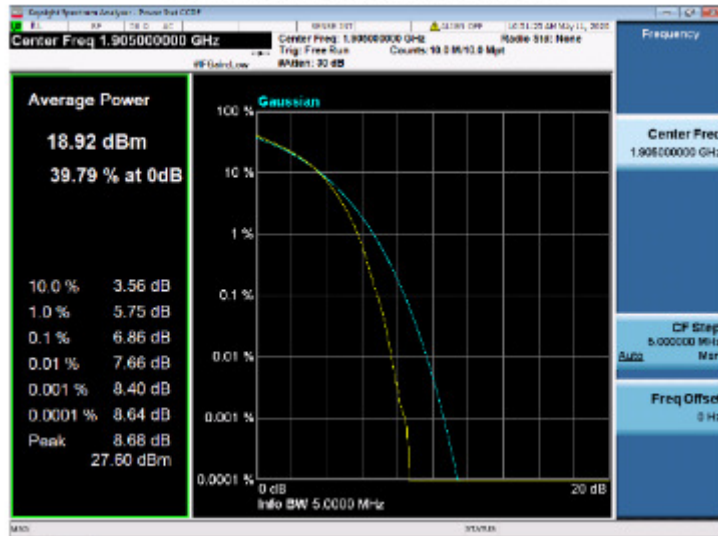
Peak-Average Ratio LTE_2_LTE_HCH_1905.0MHz_NTNV
