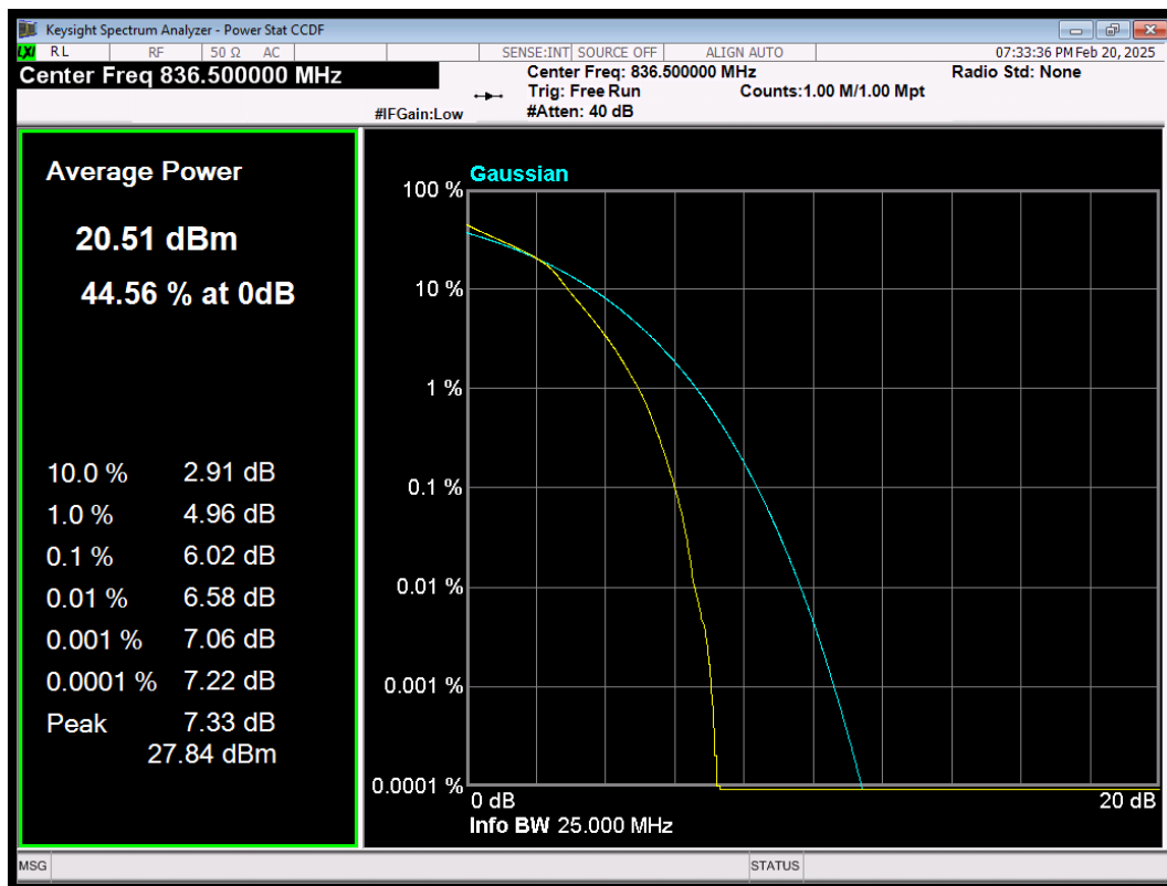
LTE Band5 QAM16 BW=5MHz Channel=20525 RB Size=25 Position=#0
