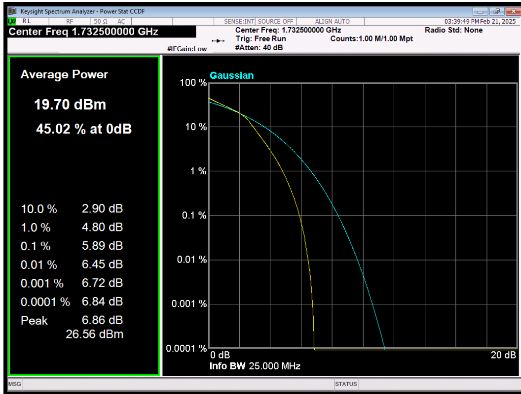
LTE Band4 QAM64 BW=3MHz Channel=20175 RB Size=15 Position=#0
