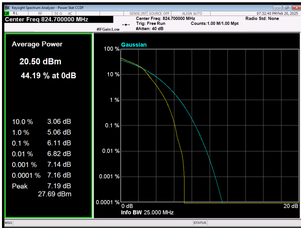
LTE Band5 QAM16 BW=1.4MHz Channel=20407 RB Size=6 Position=#0
