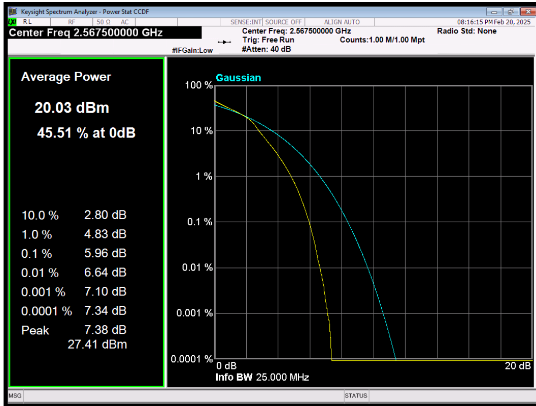
LTE Band7 QAM16 BW=5MHz Channel=21425 RB Size=25 Position=#0
