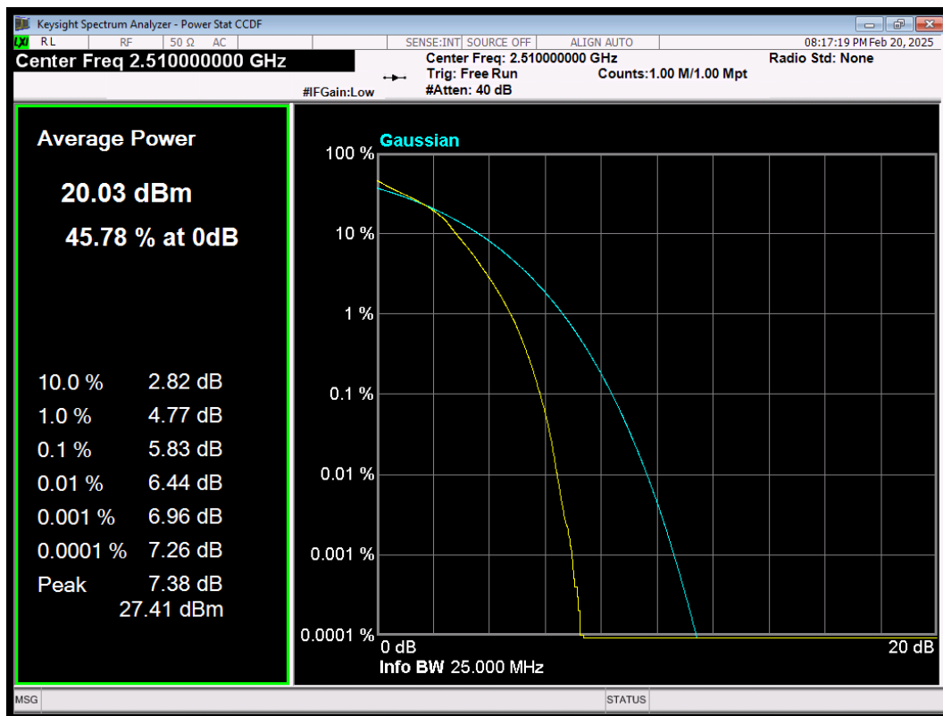
LTE Band7 QAM16 BW=20MHz Channel=20850 RB Size=100 Position=#0
