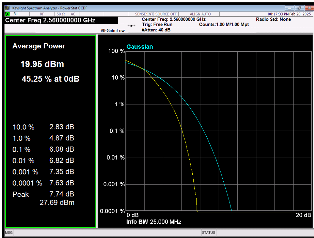
LTE Band7 QAM16 BW=20MHz Channel=21350 RB Size=100 Position=#0
