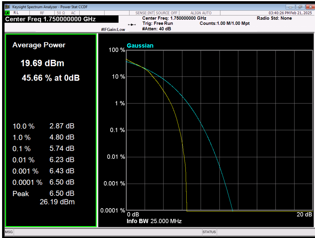
LTE Band4 QAM64 BW=10MHz Channel=20350 RB Size=50 Position=#0
