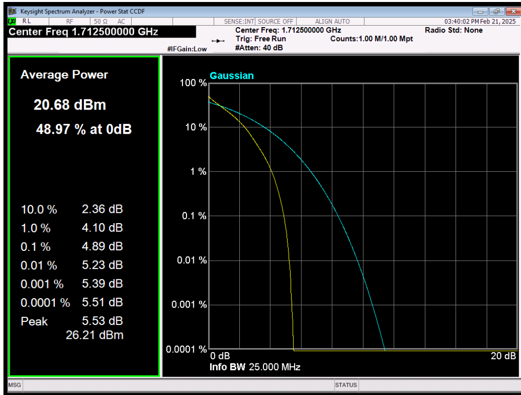
LTE Band4 QAM64 BW=5MHz Channel=19975 RB Size=25 Position=#0
