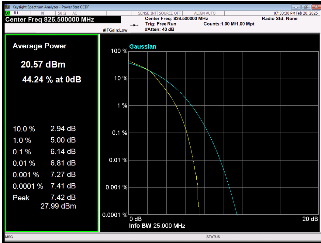
LTE Band5 QAM16 BW=5MHz Channel=20425 RB Size=25 Position=#0
