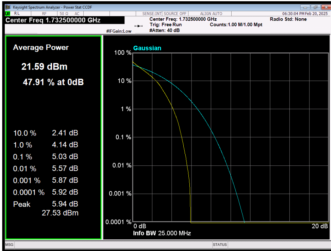
LTE Band4 QPSK BW=3MHz Channel=20175 RB Size=15 Position=#0
