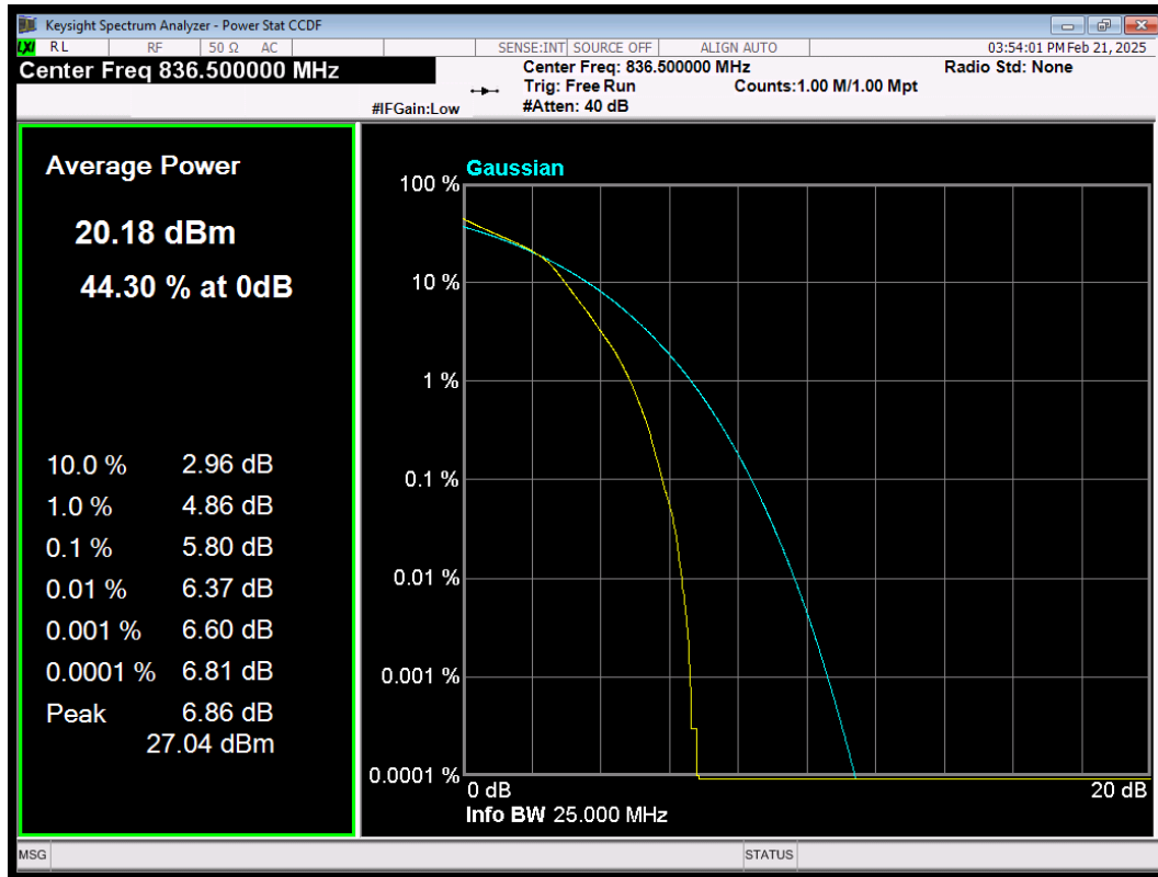
LTE Band5 QAM64 BW=3MHz Channel=20525 RB Size=15 Position=#0
