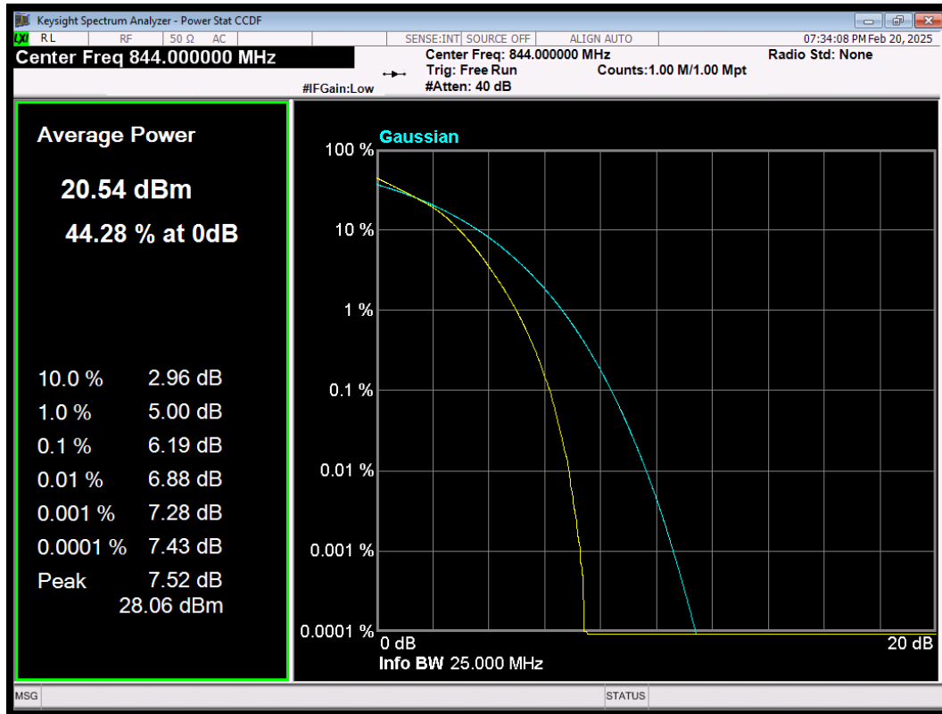
LTE Band5 QAM16 BW=10MHz Channel=20600 RB Size=50 Position=#0
