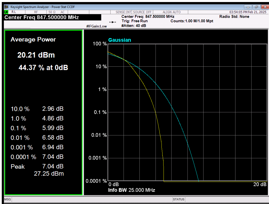
LTE Band5 QAM64 BW=3MHz Channel=20635 RB Size=15 Position=#0
