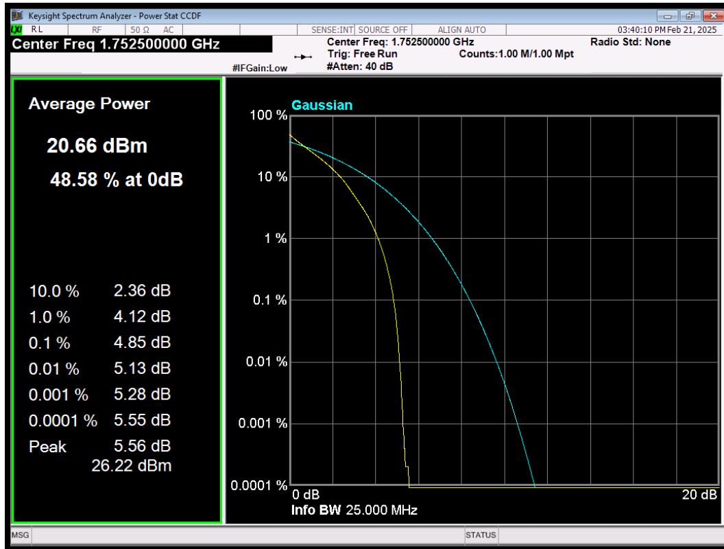
LTE Band4 QAM64 BW=5MHz Channel=20375 RB Size=25 Position=#0
