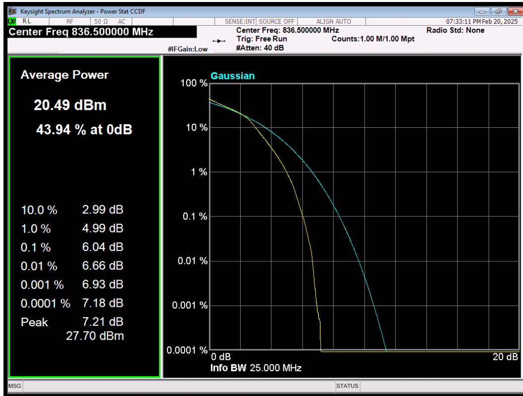
LTE Band5 QAM16 BW=3MHz Channel=20525 RB Size=15 Position=#0
