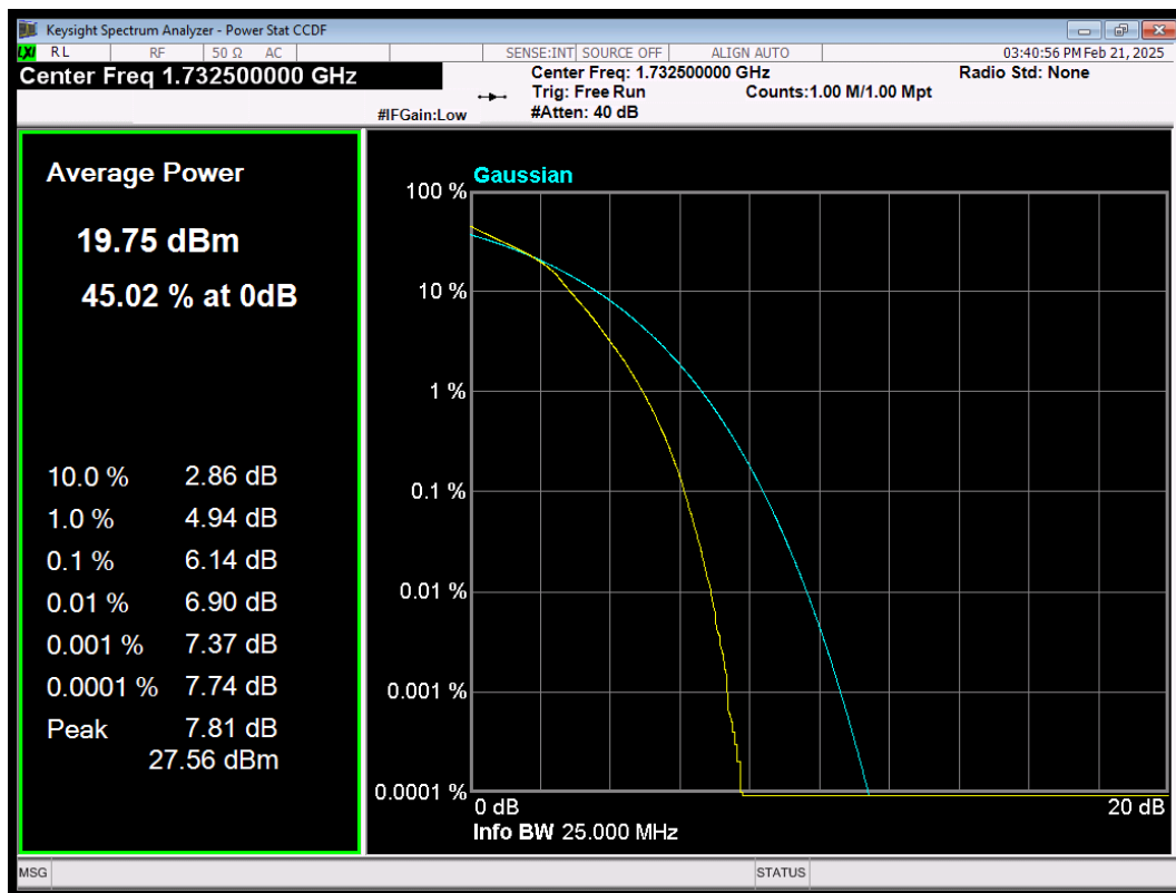
LTE Band4 QAM64 BW=20MHz Channel=20175 RB Size=100 Position=#0
