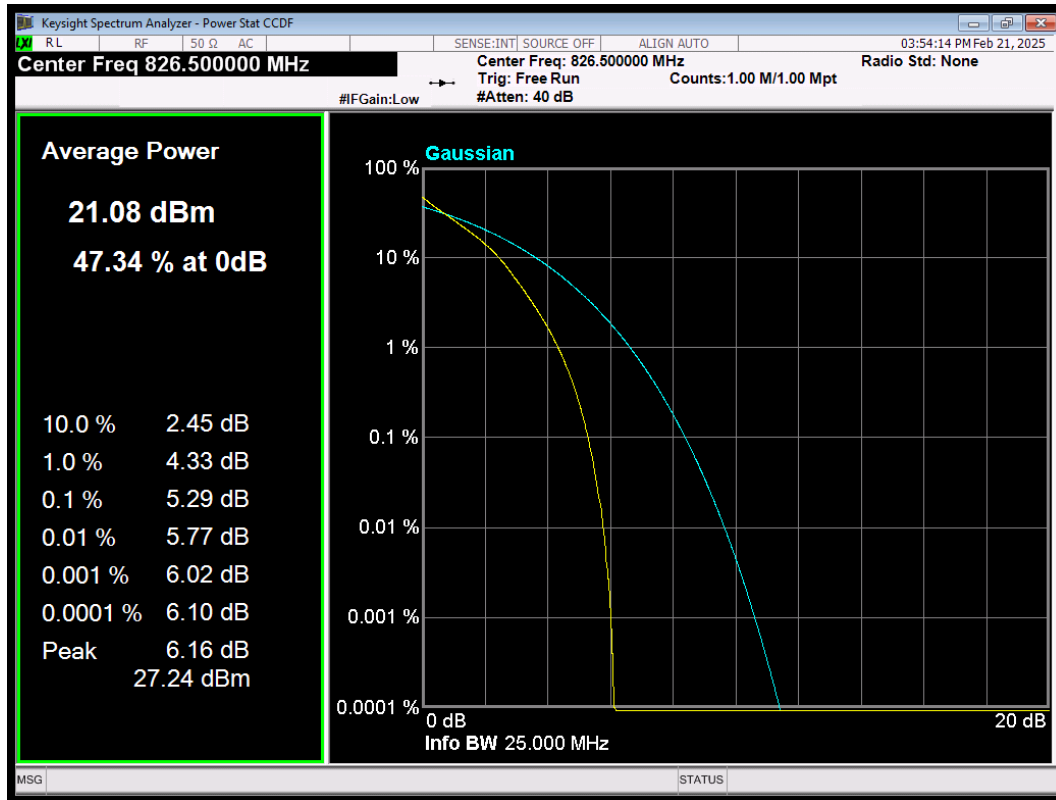
LTE Band5 QAM64 BW=5MHz Channel=20425 RB Size=25 Position=#0
