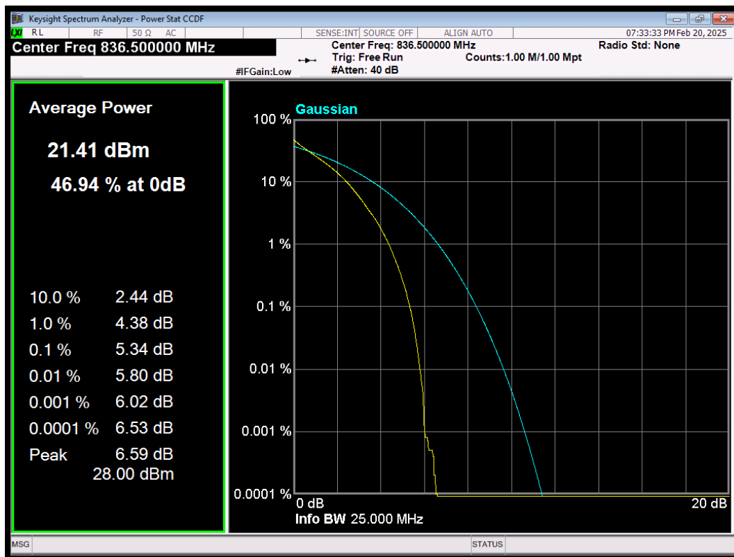
LTE Band5 QPSK BW=5MHz Channel=20525 RB Size=25 Position=#0
