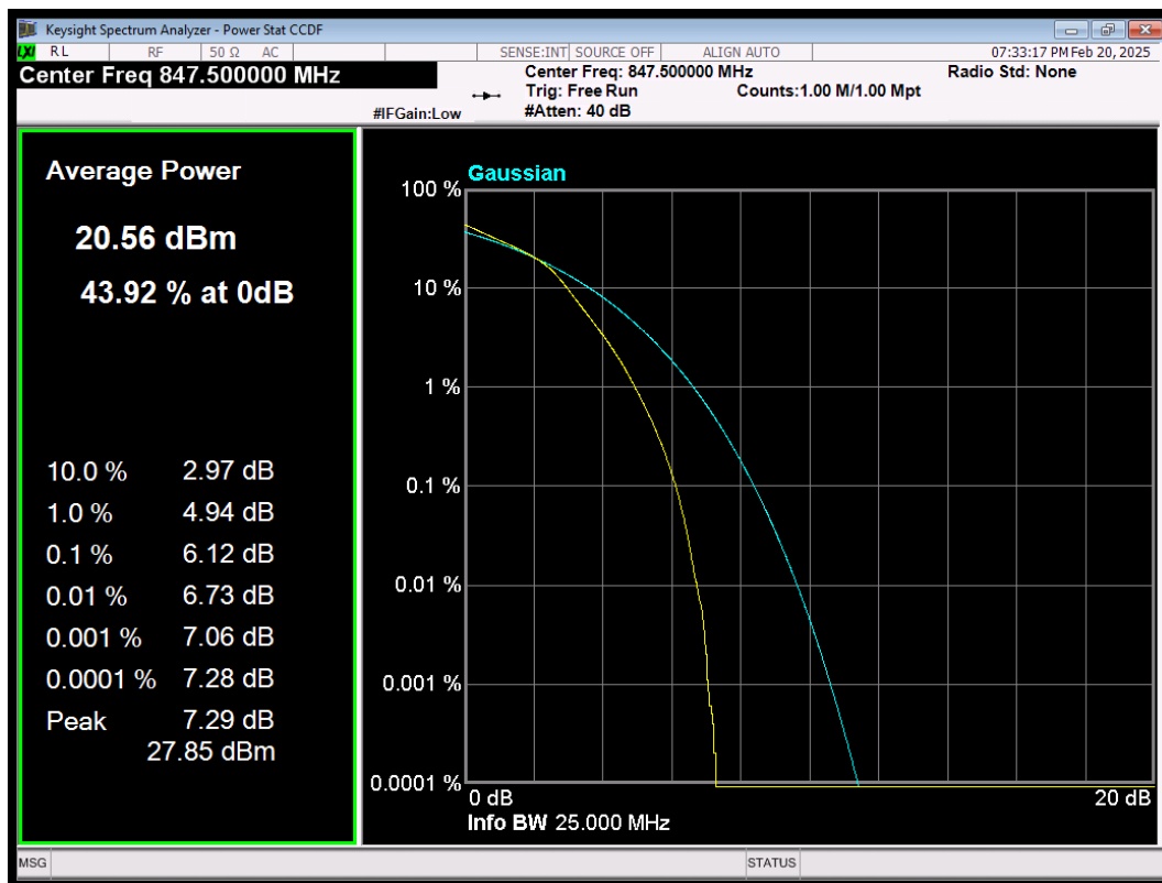
LTE Band5 QAM16 BW=3MHz Channel=20635 RB Size=15 Position=#0
