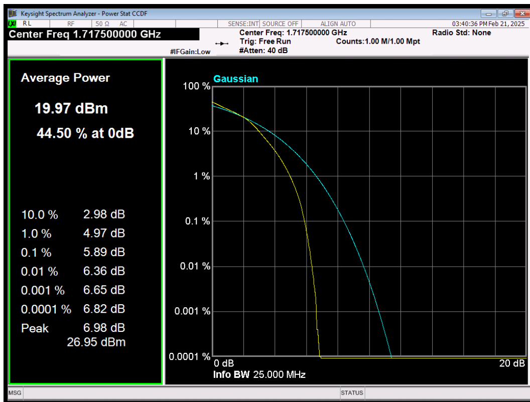
LTE Band4 QAM64 BW=15MHz Channel=20025 RB Size=75 Position=#0
