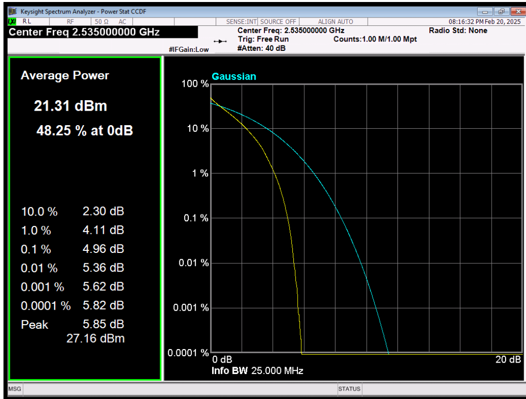
LTE Band7 QPSK BW=10MHz Channel=21100 RB Size=50 Position=#0
