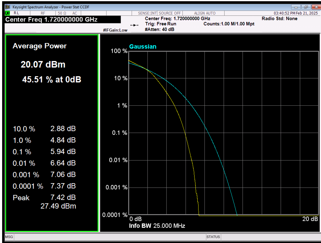
LTE Band4 QAM64 BW=20MHz Channel=20050 RB Size=100 Position=#0
