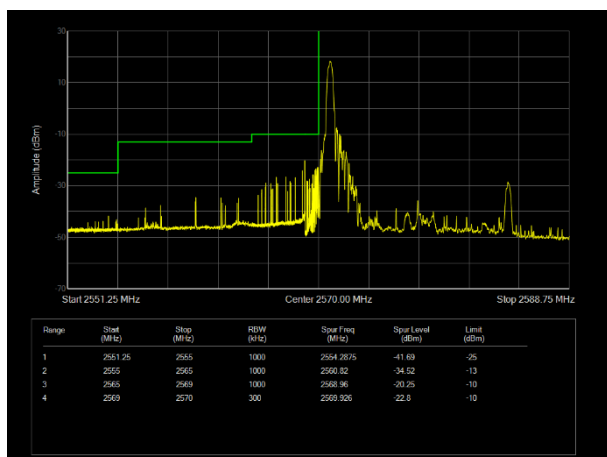
L\LTE Band38 QAM16 BW=15MHz Channel=37825 RB Size=1 Position=#0
