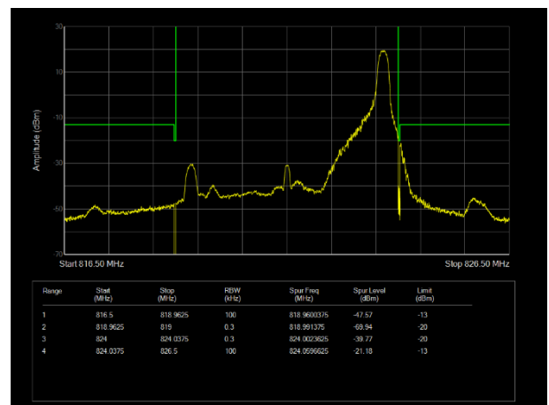
H\LTE Band26 (814-824) QAM64 BW=5MHz Channel=26765 RB Size=1 Position=#Max
