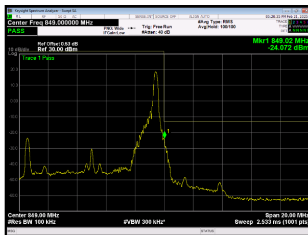
H\LTE Band26 (824-849) QAM64 BW=10MHz Channel=26990 RB Size=1 Position=#Max
