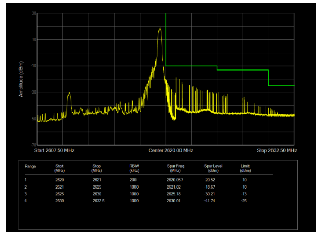
H\LTE Band38 QPSK BW=10MHz Channel=38200 RB Size=1 Position=#Max
