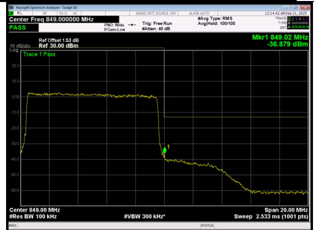
HLLTE Band26 (824-849) QAM16 BW=10MHz Channel=26990 RB Size=50 Position=#0
