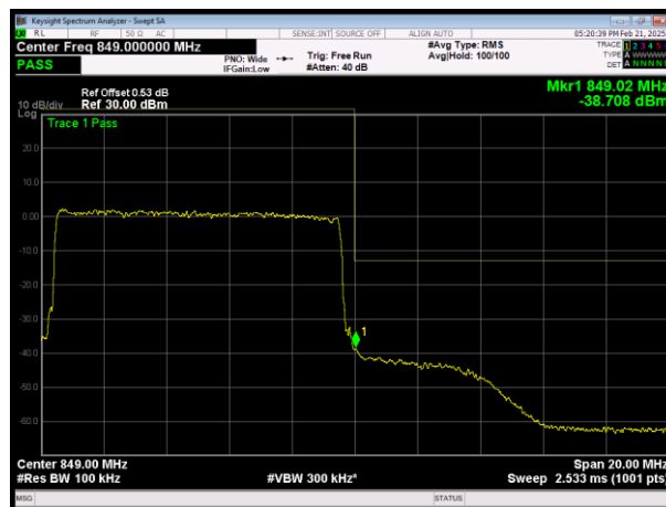
H\LTE Band26 (824-849) QAM64 BW=10MHz Channel=26990 RB Size=50 Position=#0
