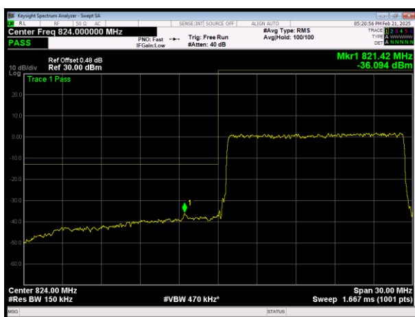
L1LTE Band26 (824-849) QAM64 BW=15MHz Channel=26865 RB Size=75 Position=#0
