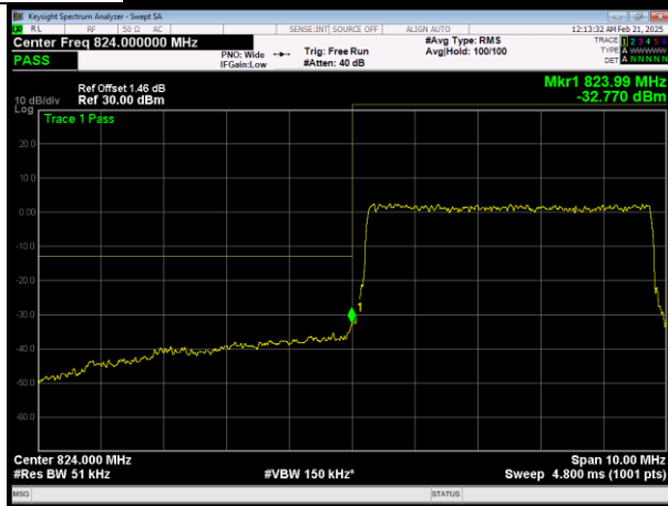
L\LTE Band26 (824-849) QAM16 BW=5MHz Channel=26815 RB Size=25 Position=#0
