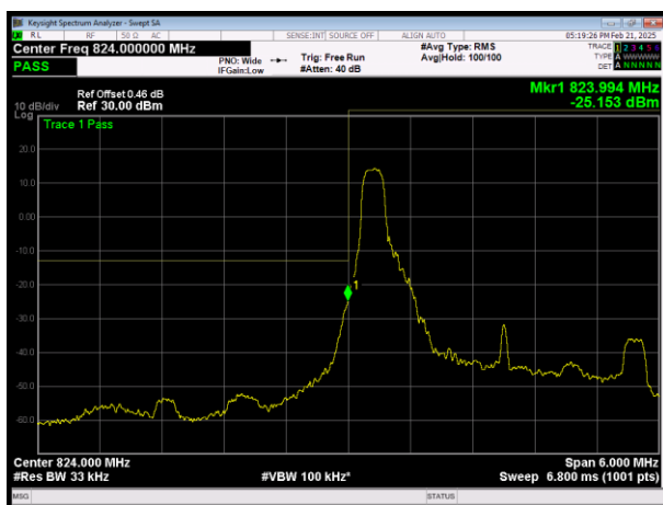
L1LTE Band26 (824-849) QAM64 BW=3MHz Channel=26805 RB Size=1 Position=#0
