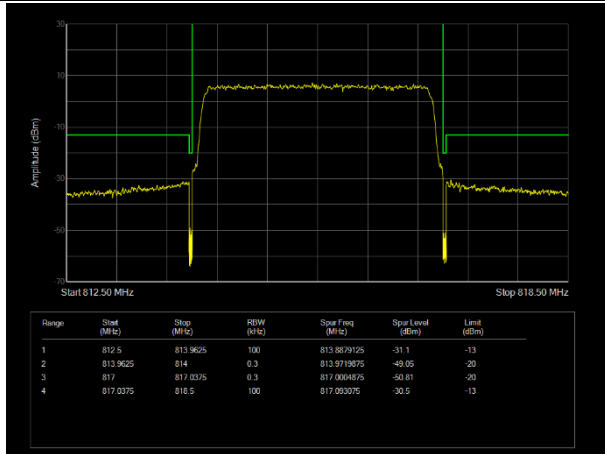
L\LTE Band26 (814-824) QAM64 BW=3MHz Channel=26705 RB Size=15 Position=#0
