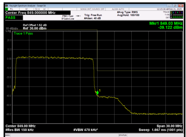
HLLTE Band26 (824-849) QAM16 BW=15MHz Channel=26965 RB Size=75 Position=#0
