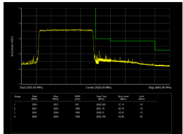
H\LTE Band38 QAM16 BW=20MHz Channel=38150 RB Size=100 Position=#0
