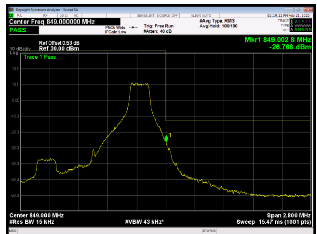
H\LTE Band26 (824-849) QAM64 BW=1.4MHz Channel=27033 RB Size=1 Position=#Max
