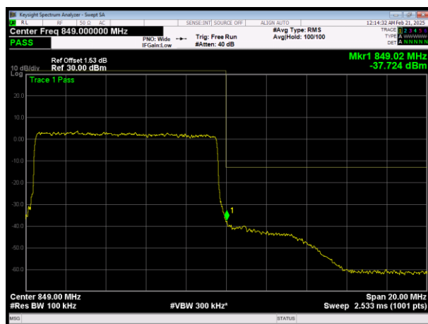
H\LTE Band26 (824-849) QPSK BW=10MHz Channel=26990 RB Size=50 Position=#0
