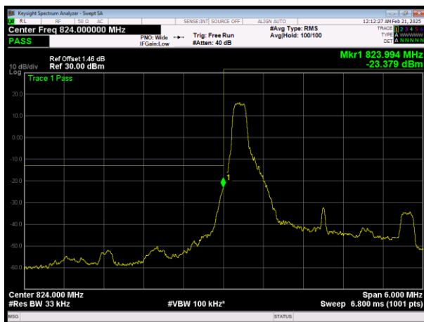
L/LTE Band26 (824-849) QPSK BW=3MHz Channel=26805 RB Size=1 Position=#0
