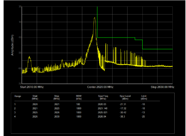
H\LTE Band38 QAM16 BW=5MHz Channel=38225 RB Size=1 Position=#Max
