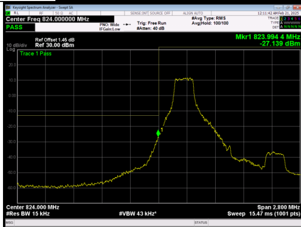
L\LTE Band26 (824-849) QAM16 BW=1.4MHz Channel=26797 RB Size=1 Position=#0
