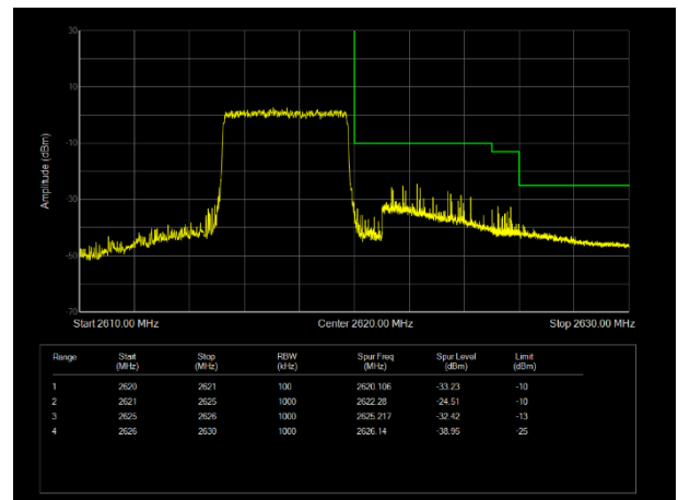
H\LTE Band38 QAM16 BW=5MHz Channel=38225 RB Size=25 Position=#0
