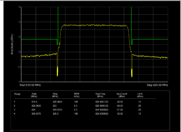
H\LTE Band26 (814-824) QAM64 BW=3MHz Channel=26775 RB Size=15 Position=#0
