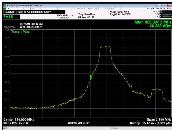
L\LTE Band26 (824-849) QAM64 BW=1.4MHz Channel=26797 RB Size=1 Position=#0
