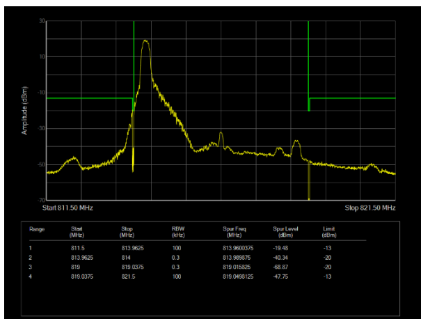
L\LTE Band26 (814-824) QAM64 BW=5MHz Channel=26715 RB Size=1 Position=#0
