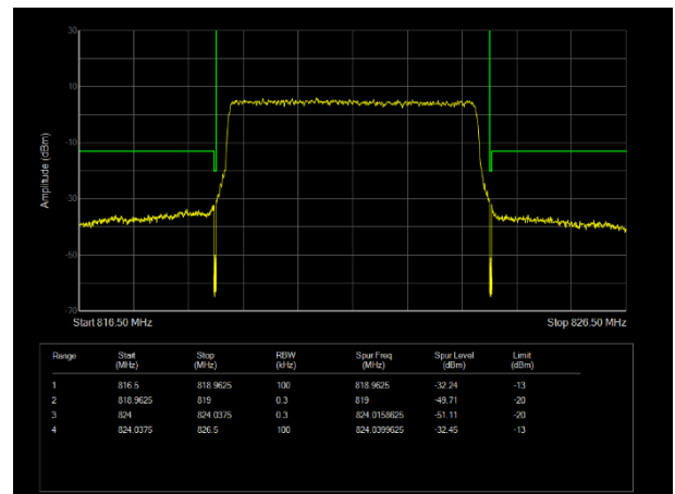
H\LTE Band26 (814-824) QAM64 BW=5MHz Channel=26765 RB Size=25 Position=#0
