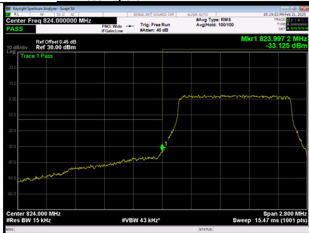
L\LTE Band26 (824-849) QAM64 BW=1.4MHz Channel=26797 RB Size=6 Position=#0
