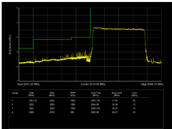
L\LTE Band38 QPSK BW=15MHz Channel=37825 RB Size=75 Position=#0
