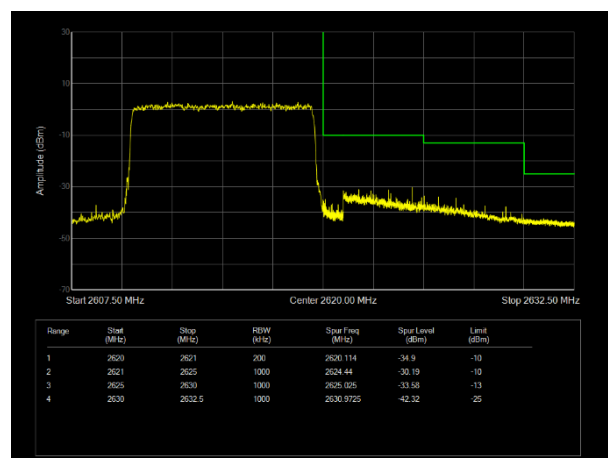
H\LTE Band38 QAM16 BW=10MHz Channel=38200 RB Size=50 Position=#0
