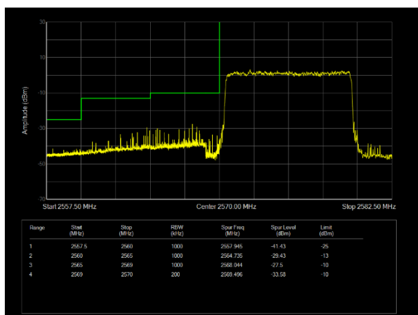
L\LTE Band38 QAM16 BW=10MHz Channel=37800 RB Size=50 Position=#0
