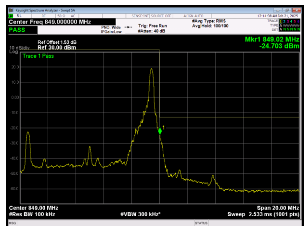
H\LTE Band26 (824-849) QAM16 BW=10MHz Channel=26990 RB Size=1 Position=#Max
