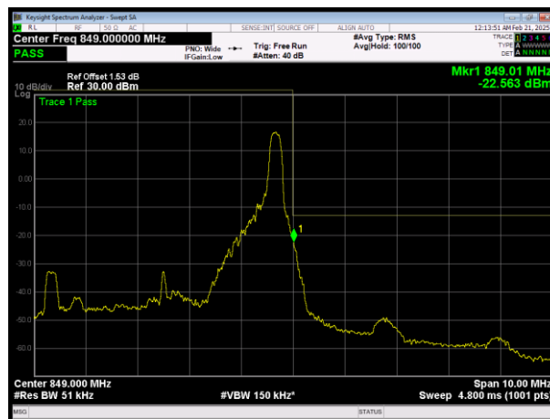
H\LTE Band26 (824-849) QAM16 BW=5MHz Channel=27015 RB Size=1 Position=#Max
