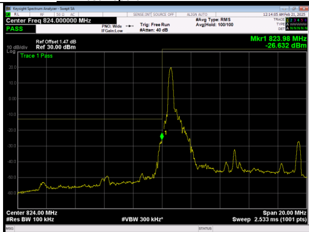
L\LTE Band26 (824-849) QPSK BW=10MHz Channel=26840 RB Size=1 Position=#0
