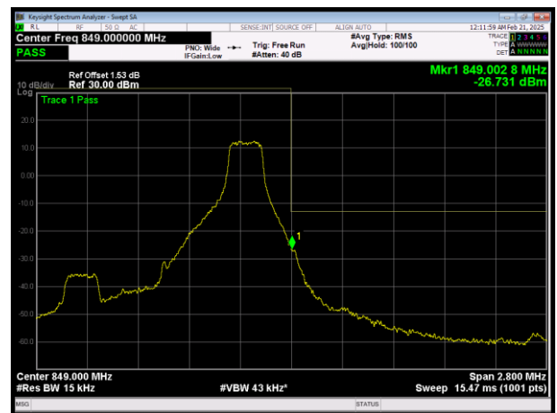
H\LTE Band26 (824-849) QPSK BW=1.4MHz Channel=27033 RB Size=1 Position=#Max
