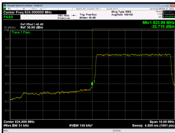
L\LTE Band26 (824-849) QPSK BW=5MHz Channel=26815 RB Size=25 Position=#0
