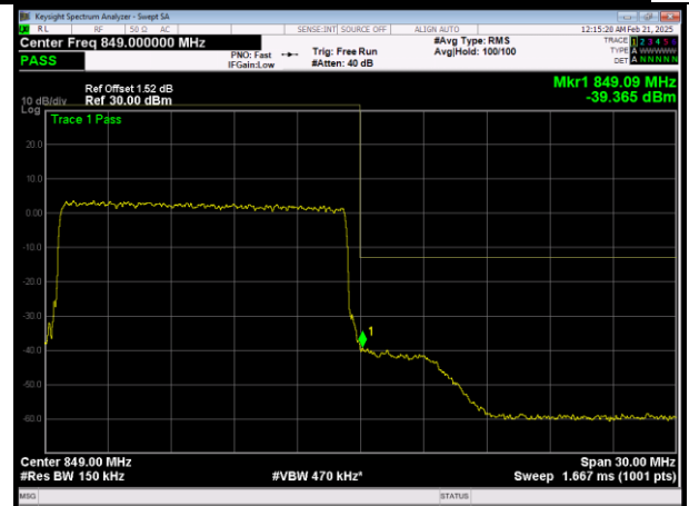
H/LTE Band26 (824-849) QPSK BW=15MHz Channel=26965 RB Size=75 Position=#0
