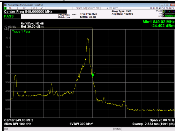
H\LTE Band26 (824-849) QPSK BW=10MHz Channel=26990 RB Size=1 Position=#Max
