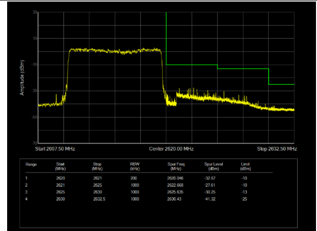
H\LTE Band38 QPSK BW=10MHz Channel=38200 RB Size=50 Position=#0
