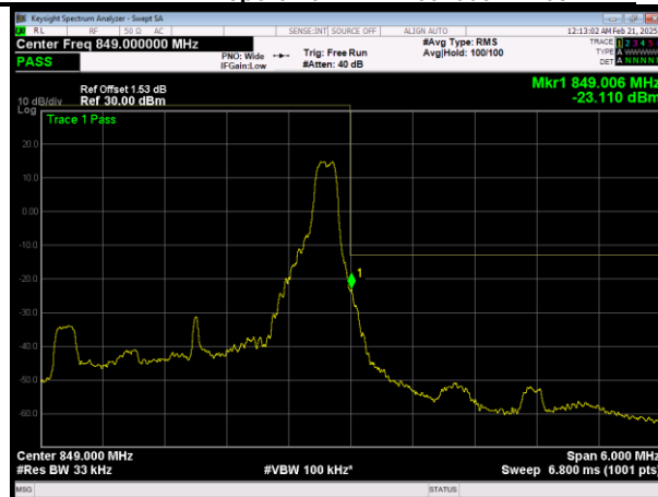
H\LTE Band26 (824-849) QAM16 BW=3MHz Channel=27025 RB Size=1 Position=#Max
