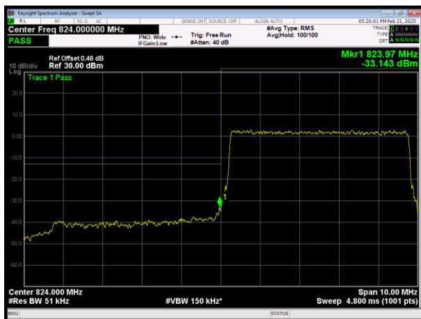
L\LTE Band26 (824-849) QAM64 BW=5MHz Channel=26815 RB Size=25 Position=#0
