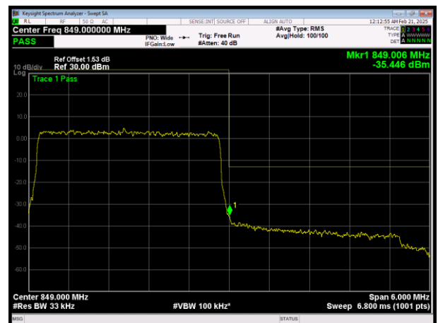
H/LTE Band26 (824-849) QPSK BW=3MHz Channel=27025 RB Size=15 Position=#0
