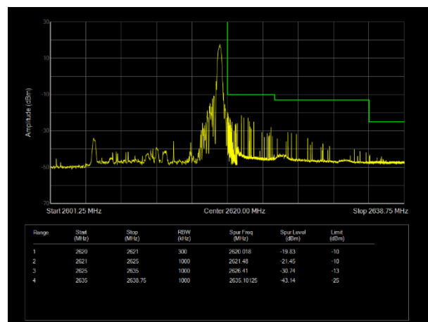
H\LTE Band38 QAM16 BW=15MHz Channel=38175 RB Size=1 Position=#Max
