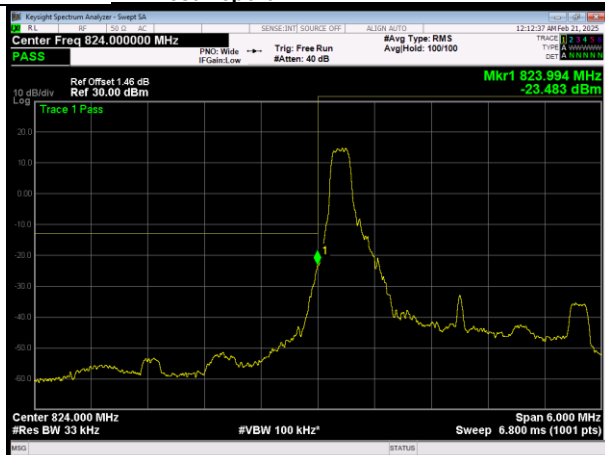
L\LTE Band26 (824-849) QAM16 BW=3MHz Channel=26805 RB Size=1 Position=#0
