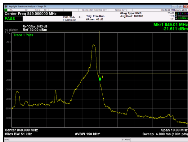
H\LTE Band26 (824-849) QAM64 BW=5MHz Channel=27015 RB Size=1 Position=#Max
