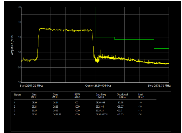
H\LTE Band38 QAM16 BW=15MHz Channel=38175 RB Size=75 Position=#0
