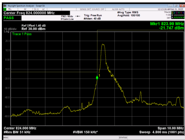
L\LTE Band26 (824-849) QAM16 BW=5MHz Channel=26815 RB Size=1 Position=#0
