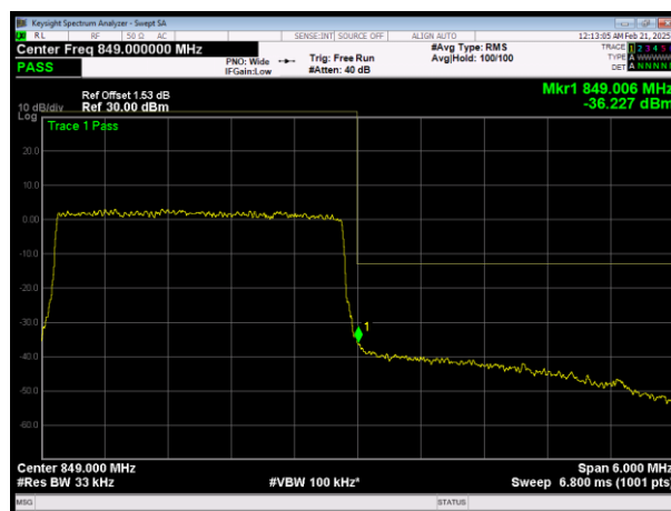
H\LTE Band26 (824-849) QAM16 BW=3MHz Channel=27025 RB Size=15 Position=#0
