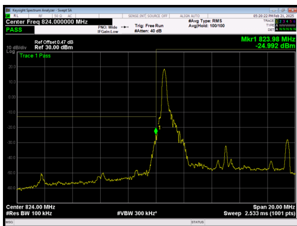
L\LTE Band26 (824-849) QAM64 BW=10MHz Channel=26840 RB Size=1 Position=#0
