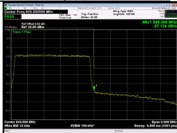
H\LTE Band26 (824-849) QAM64 BW=3MHz Channel=27025 RB Size=15 Position=#0
