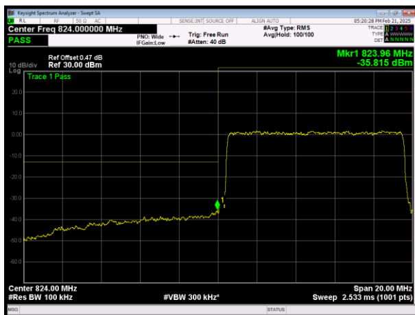
L\LTE Band26 (824-849) QAM64 BW=10MHz Channel=26840 RB Size=50 Position=#0
