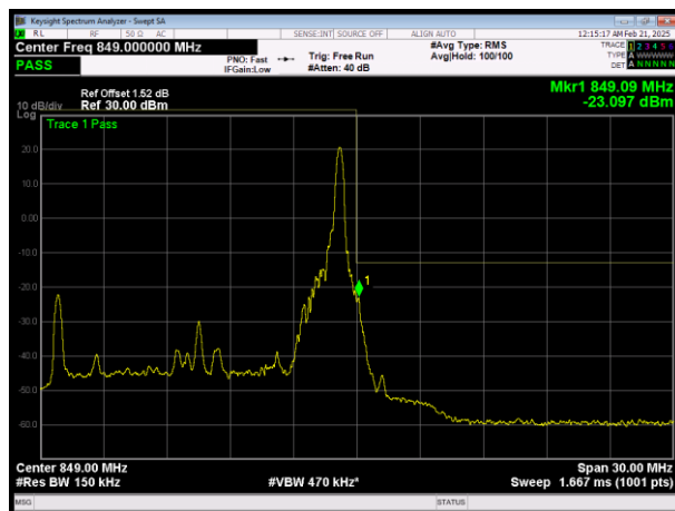
H\LTE Band26 (824-849) QPSK BW=15MHz Channel=26965 RB Size=1 Position=#Max
