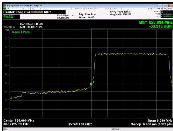
L/LTE Band26 (824-849) QPSK BW=3MHz Channel=26805 RB Size=15 Position=#0
