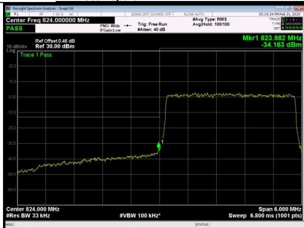
L\LTE Band26 (824-849) QAM64 BW=3MHz Channel=26805 RB Size=15 Position=#0
