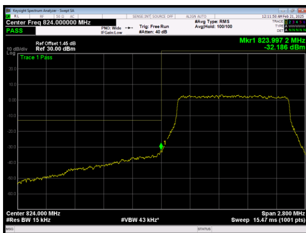
L\LTE Band26 (824-849) QAM16 BW=1.4MHz Channel=26797 RB Size=6 Position=#0
