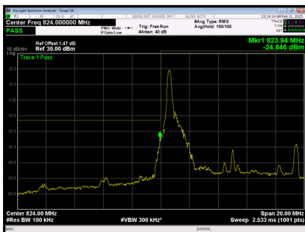
L\LTE Band26 (824-849) QAM16 BW=10MHz Channel=26840 RB Size=1 Position=#0
