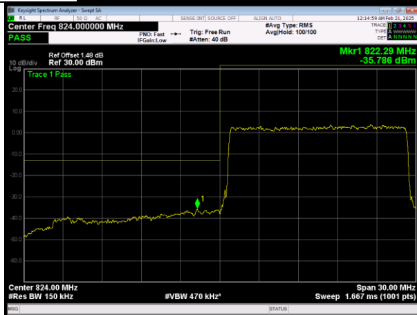
L/LTE Band26 (824-849) QPSK BW=15MHz Channel=26865 RB Size=75 Position=#0
