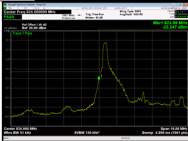
L\LTE Band26 (824-849) QPSK BW=5MHz Channel=26815 RB Size=1 Position=#0
