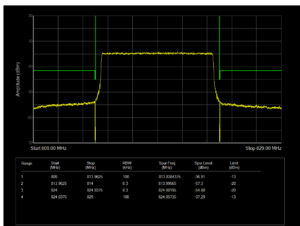
L/LTE Band26 (814-824) QAM64 BW=10MHz Channel=26740 RB Size=50 Position=#0
