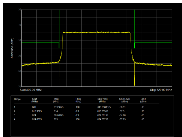
H/LTE Band26 (814-824) QAM64 BW=10MHz Channel=26740 RB Size=50 Position=#0
