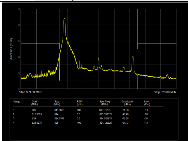
L/LTE Band26 (814-824) QAM64 BW=10MHz Channel=26740 RB Size=1 Position=#0
