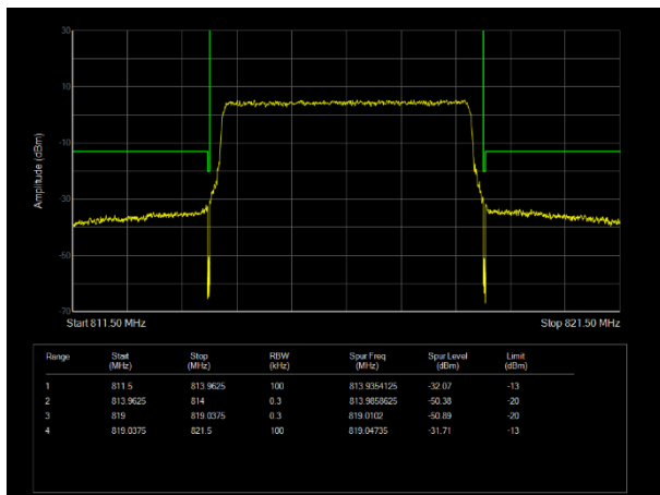
L\LTE Band26 (814-824) QAM64 BW=5MHz Channel=26715 RB Size=25 Position=#0
