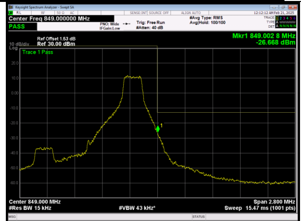
H\LTE Band26 (824-849) QAM16 BW=1.4MHz Channel=27033 RB Size=1 Position=#Max
