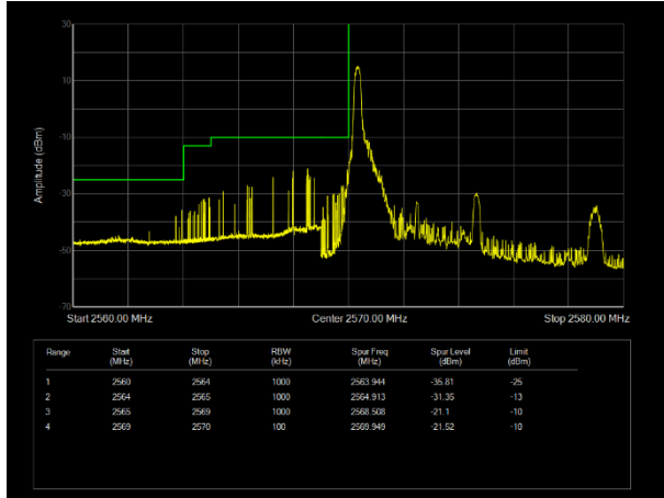
L\LTE Band38 QAM16 BW=5MHz Channel=37775 RB Size=1 Position=#0
