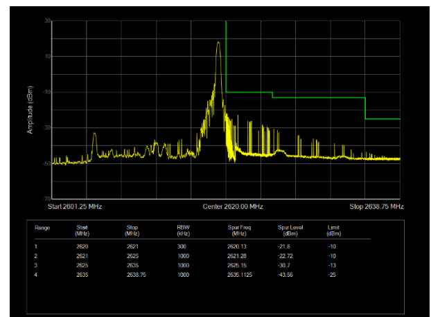
H\LTE Band38 QPSK BW=15MHz Channel=38175 RB Size=1 Position=#Max
