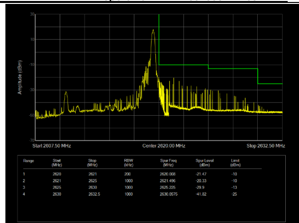
H\LTE Band38 QAM16 BW=10MHz Channel=38200 RB Size=1 Position=#Max
