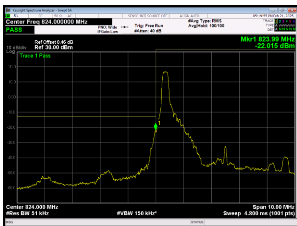
L\LTE Band26 (824-849) QAM64 BW=5MHz Channel=26815 RB Size=1 Position=#0
