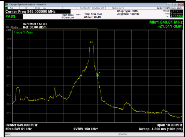
H\LTE Band26 (824-849) QPSK BW=5MHz Channel=27015 RB Size=1 Position=#Max
