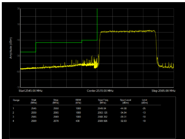
L\LTE Band38 QAM16 BW=20MHz Channel=37850 RB Size=100 Position=#0
