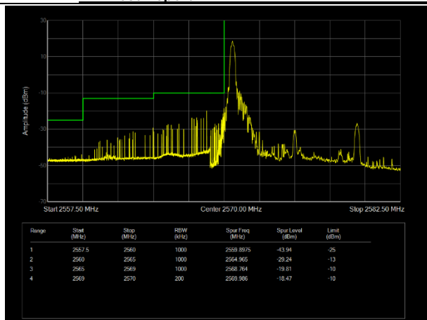
L\LTE Band38 QAM16 BW=10MHz Channel=37800 RB Size=1 Position=#0
