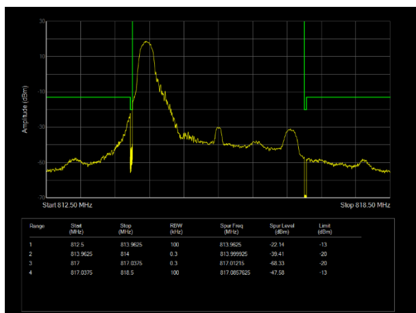
L/LTE Band26 (814-824) QAM64 BW=3MHz Channel=26705 RB Size=1 Position=#0
