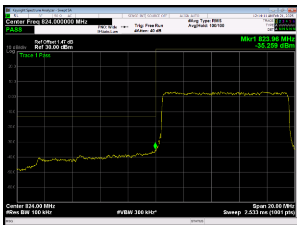
L\LTE Band26 (824-849) QPSK BW=10MHz Channel=26840 RB Size=50 Position=#0
