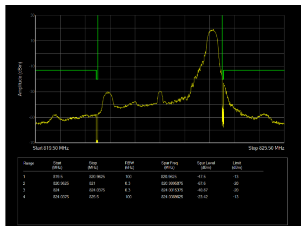
H/LTE Band26 (814-824) QAM64 BW=3MHz Channel=26775 RB Size=1 Position=#Max
