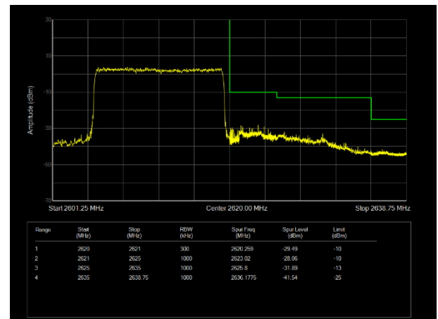
H\LTE Band38 QPSK BW=15MHz Channel=38175 RB Size=75 Position=#0
