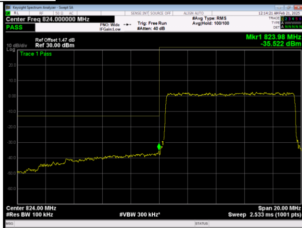
LLTE Band26 (824-849) QAM16 BW=10MHz Channel=26840 RB Size=50 Position=#0
