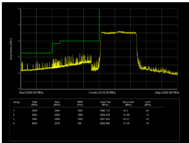
L\LTE Band38 QAM16 BW=5MHz Channel=37775 RB Size=25 Position=#0
