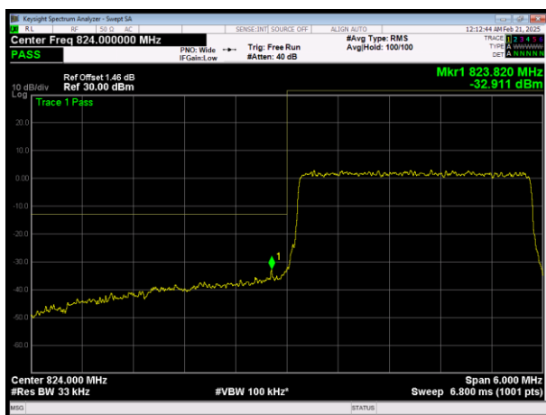
L\LTE Band26 (824-849) QAM16 BW=3MHz Channel=26805 RB Size=15 Position=#0
