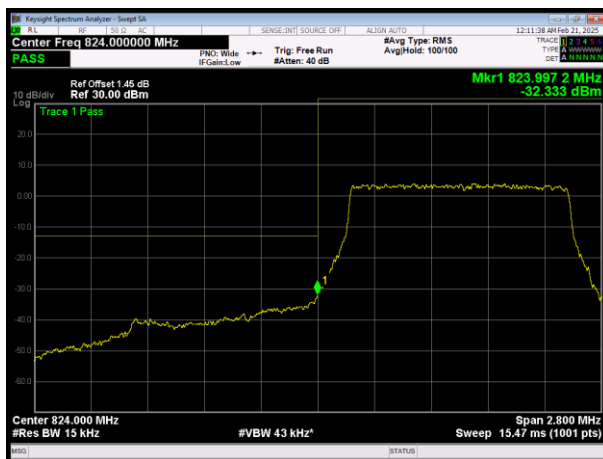
L\LTE Band26 (824-849) QPSK BW=1.4MHz Channel=26797 RB Size=6 Position=#0
