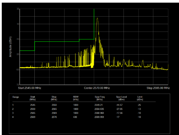
L\LTE Band38 QAM16 BW=20MHz Channel=37850 RB Size=1 Position=#0
