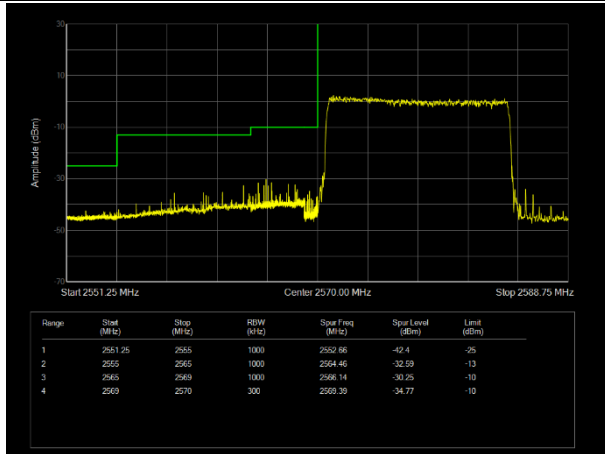
L\LTE Band38 QAM16 BW=15MHz Channel=37825 RB Size=75 Position=#0
