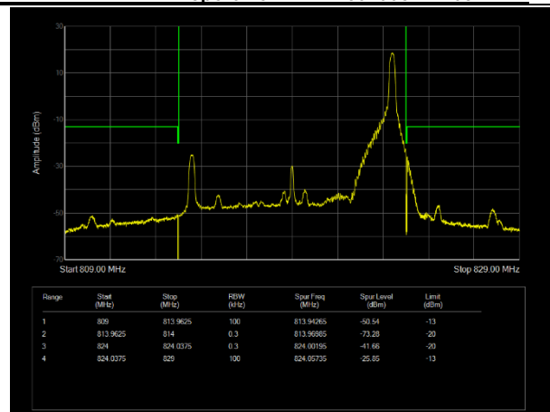
H/LTE Band26 (814-824) QAM64 BW=10MHz Channel=26740 RB Size=1 Position=#Max
