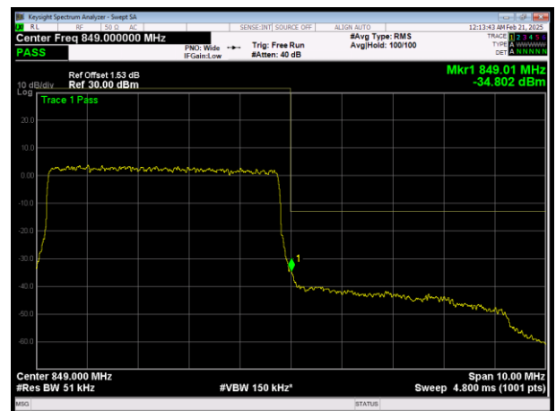
H\LTE Band26 (824-849) QPSK BW=5MHz Channel=27015 RB Size=25 Position=#0
