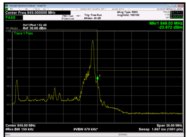
HLLTE Band26 (824-849) QAM16 BW=15MHz Channel=26965 RB Size=1 Position=#Max
