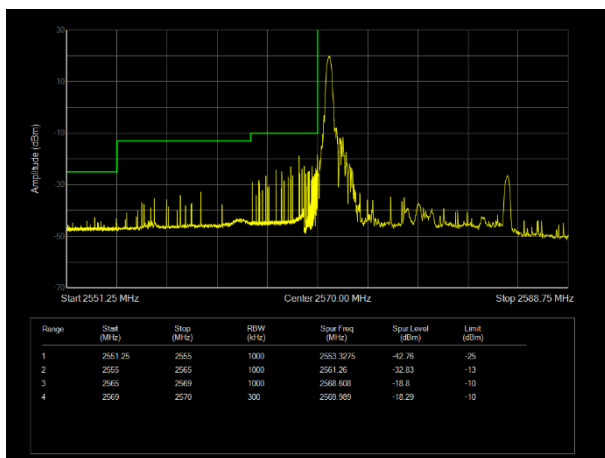
L\LTE Band38 QPSK BW=15MHz Channel=37825 RB Size=1 Position=#0
