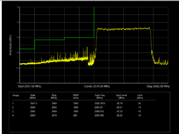
L\LTE Band38 QPSK BW=10MHz Channel=37800 RB Size=50 Position=#0
