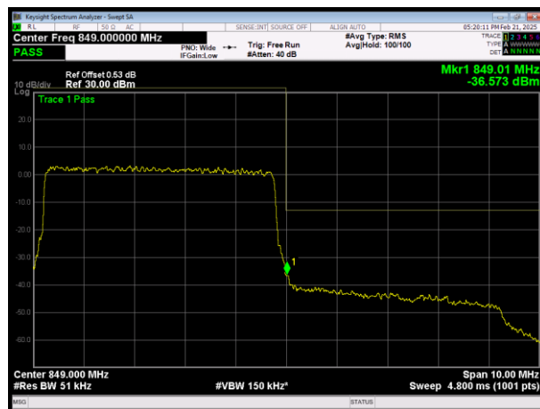
H\LTE Band26 (824-849) QAM64 BW=5MHz Channel=27015 RB Size=25 Position=#0
