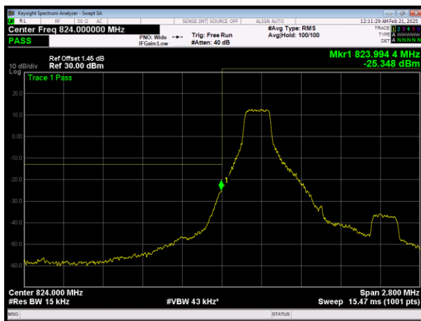
L\LTE Band26 (824-849) QPSK BW=1.4MHz Channel=26797 RB Size=1 Position=#0
