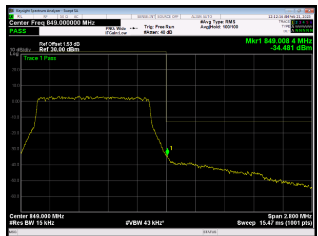
H\LTE Band26 (824-849) QAM16 BW=1.4MHz Channel=27033 RB Size=6 Position=#0
