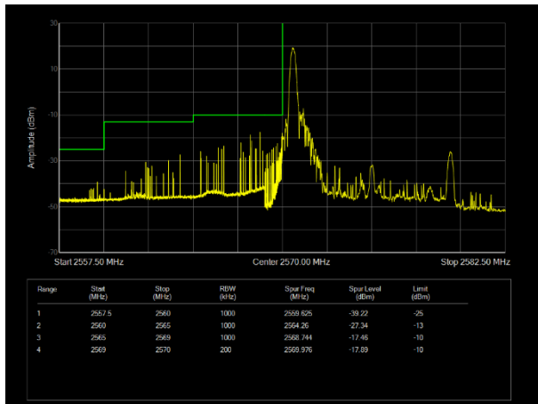
L\LTE Band38 QPSK BW=10MHz Channel=37800 RB Size=1 Position=#0
