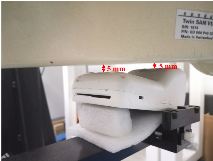
Body Back (WLAN 2.4G/5G) Setup Photo(5mm)
