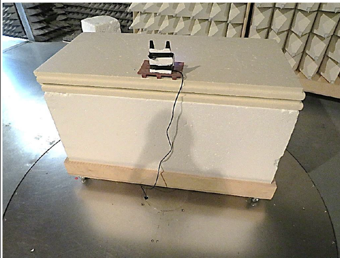
Test setup above 30 MHz - view 2
