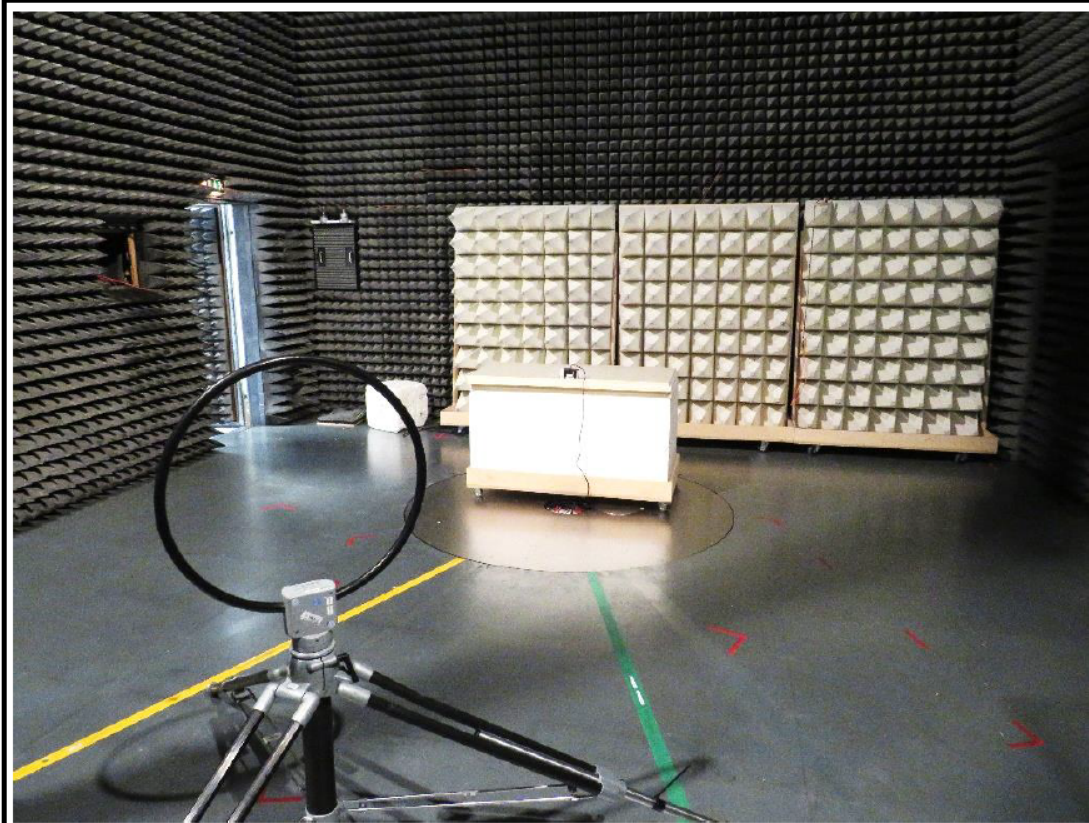
Test setup below 30 MHz - view 2
