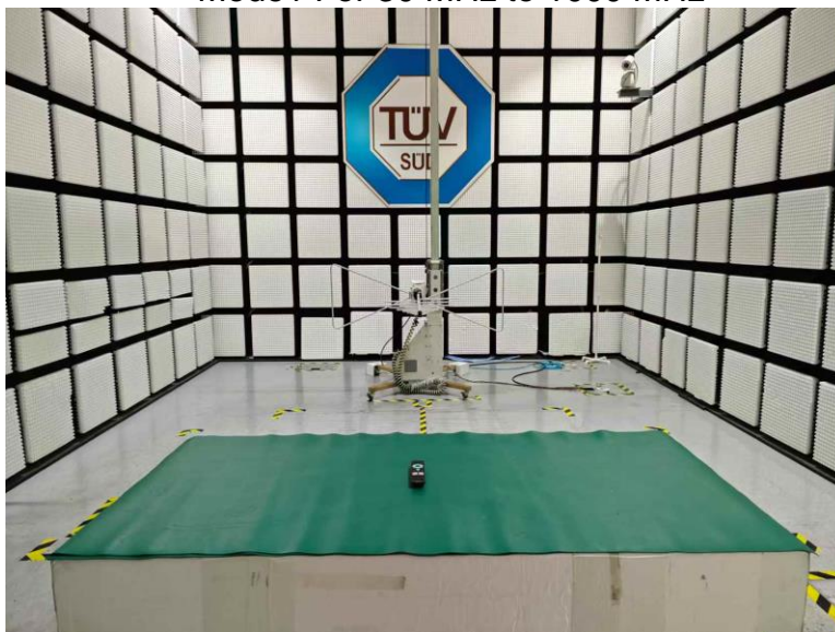
Radiated Emission Setup Mode1 For 30 MHz to 1000 MHz
