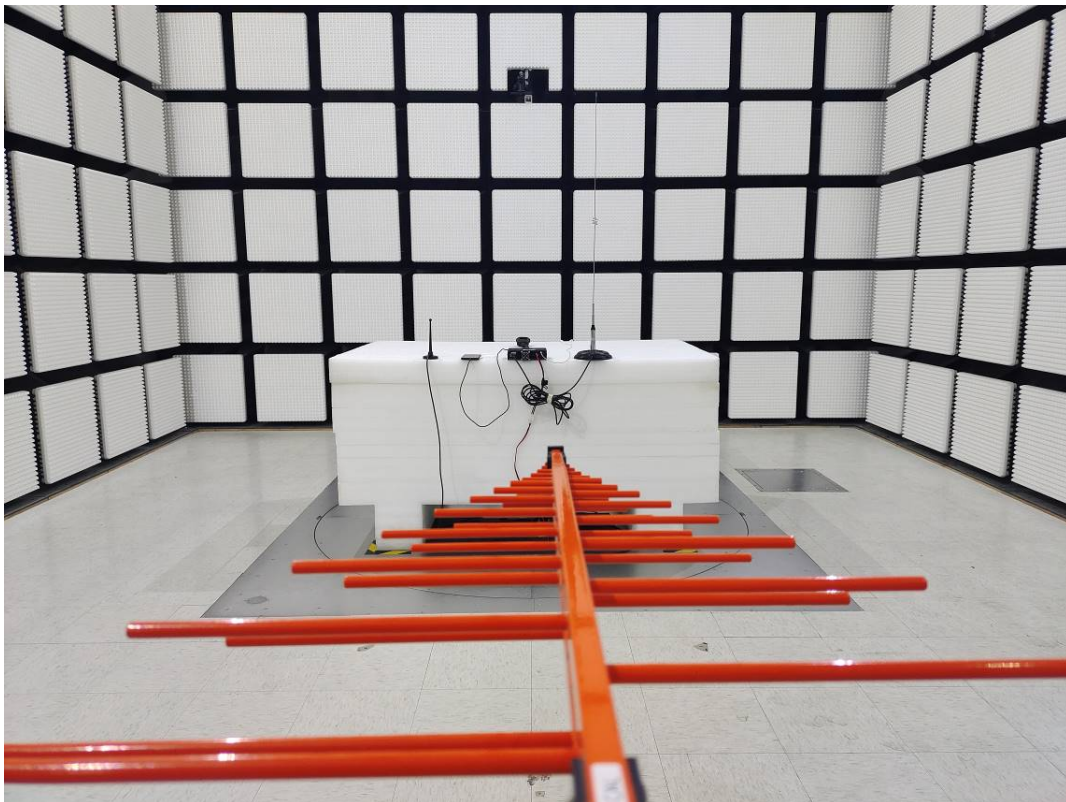
Radiated Emission 30M-1GHz Rear View M1
