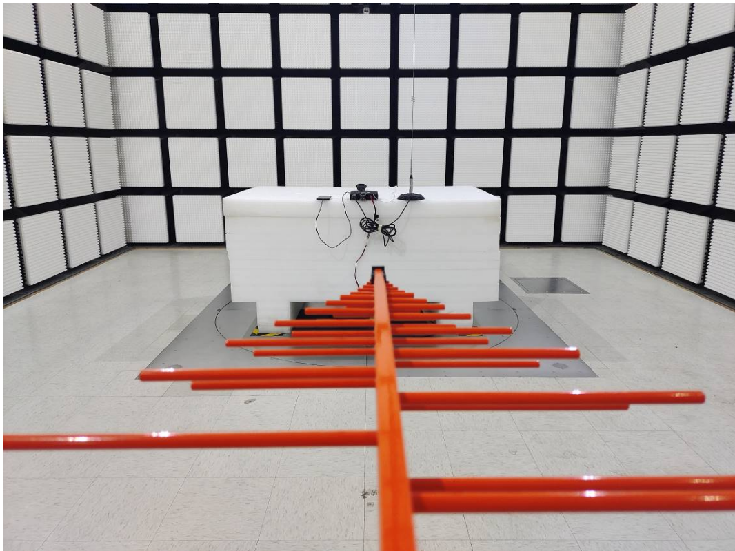
Radiated Emission 30M-1GHz Rear View M2
