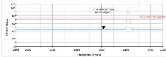
BLE Channel 0 Peak
