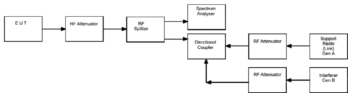
Figure i Test Setup
