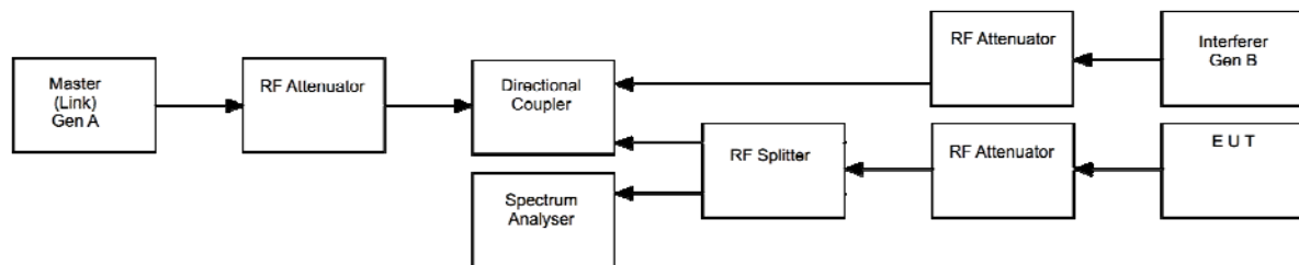
Figure ii Test Setup
