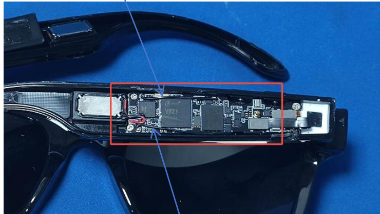
ANT 1 - WLAN Antenna
