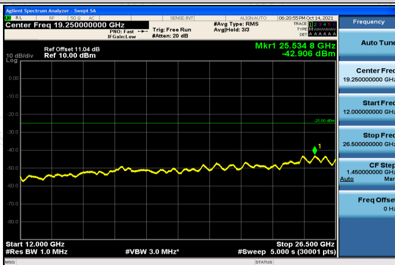
Band41-20MHz-16QAM-41140-1RB#0-Range6:12000~26500MHz
