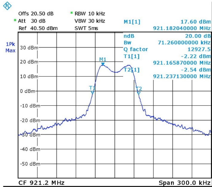
Figure 9. — 921.2 MHz
