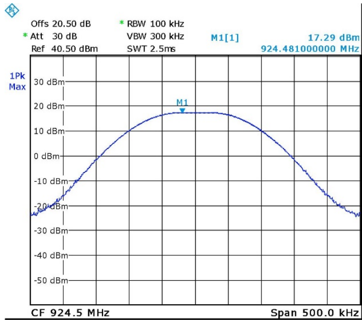
Figure 27 — 924.5 MHz
