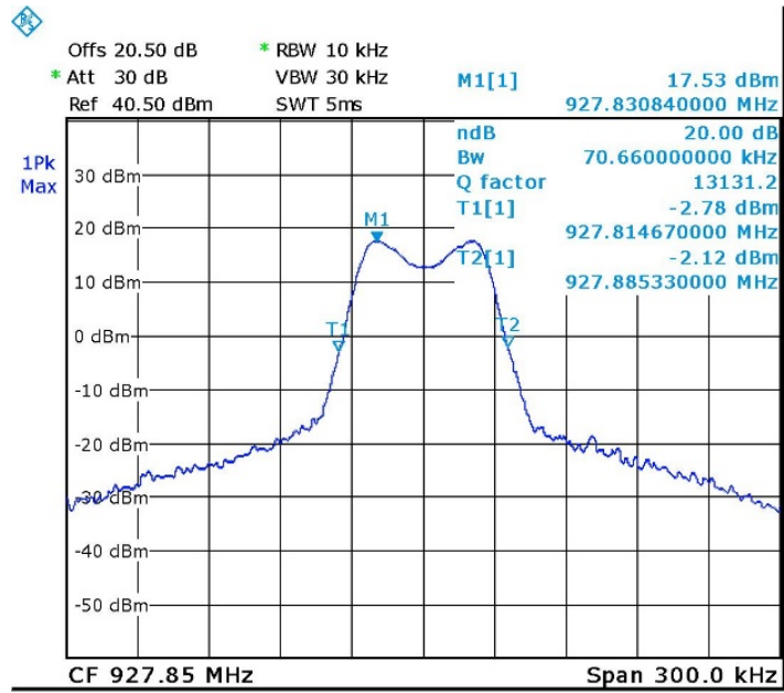
Figure 11. — 927.8 MHz
