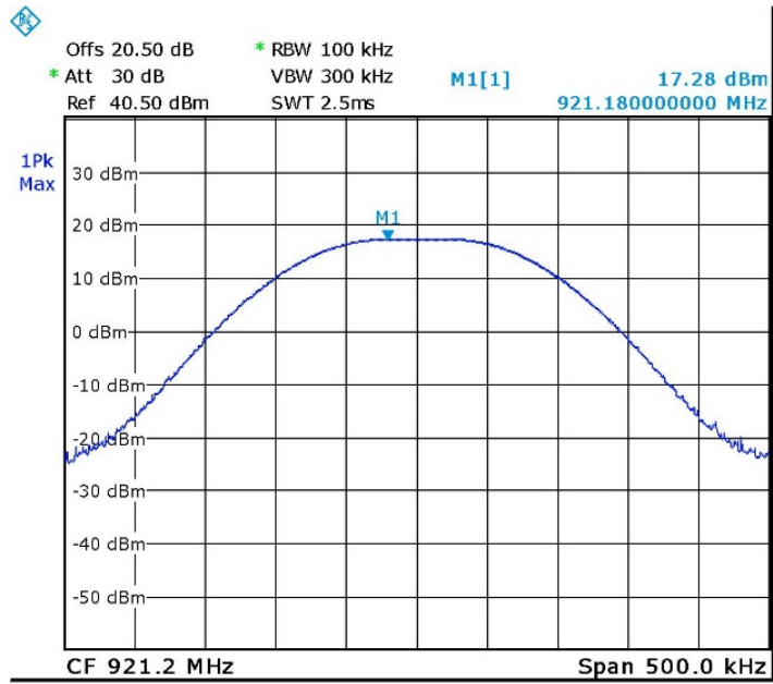
Figure 26 — 921.2 MHz
