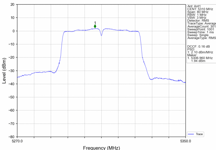
802.11ac(VHT40)_HCH_5310MHz_Ant1_NTNV
