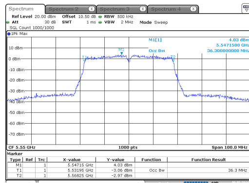
n40_5550MHz_Chain 0
