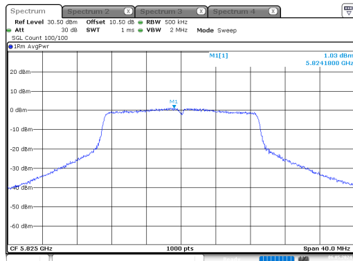
n20_5825MHz_Chain 0
