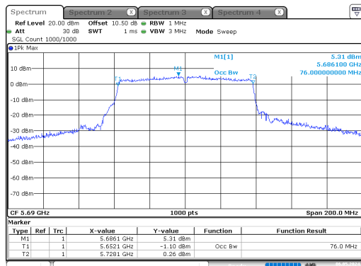
ac80_5690MHz_Chain 0
