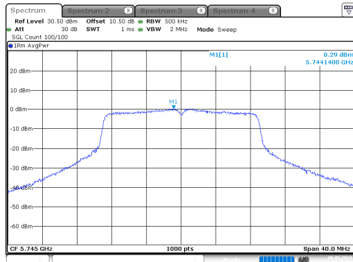
n20_5745MHz_Chain 0
