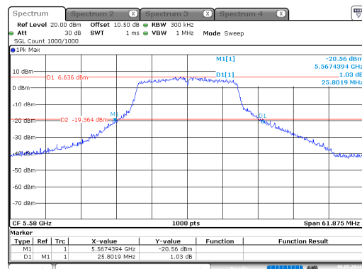
n20_5580MHz_Chain 0
