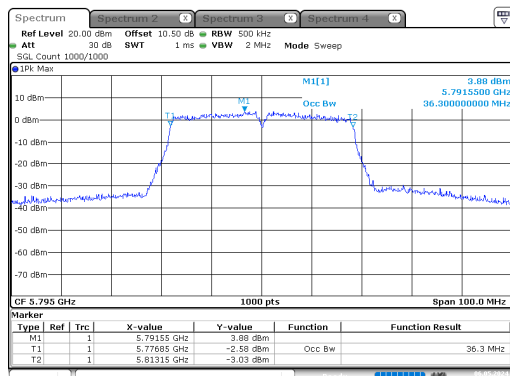
n40_5795MHz_Chain 0
