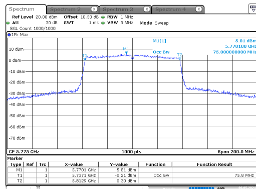
ac80_5775MHz_Chain 0
