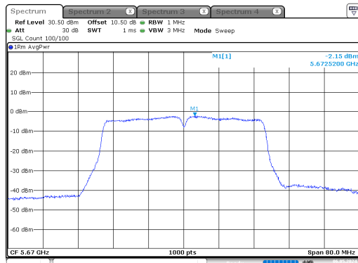
n40_5670MHz_Chain 0
