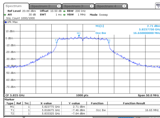
a_5825MHz_Chain 0
