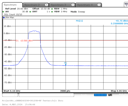
n20_5200MHz_Chain 0
