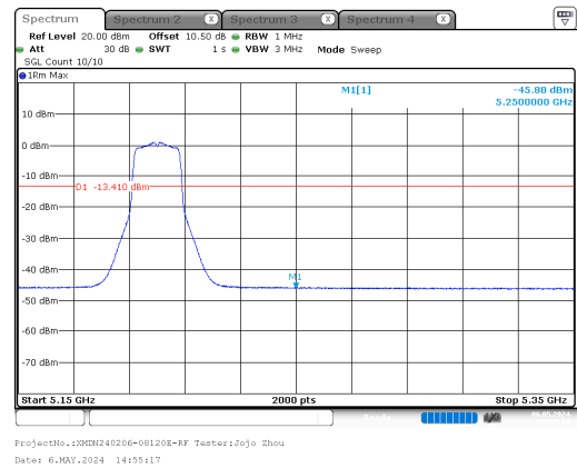
n20_5180MHz_Chain 0
