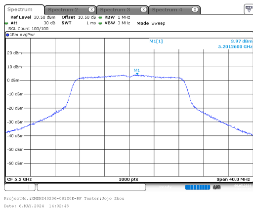
n20_5200MHz_Chain 0
