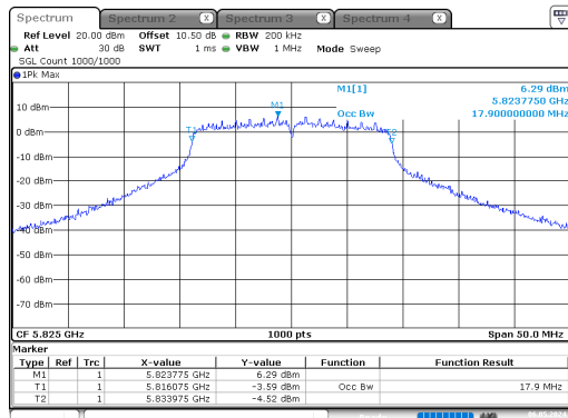
n20_5825MHz_Chain 0
