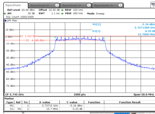
a_5745MHz_Chain 0
