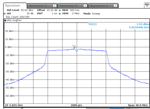
a_5825MHz_Chain 0
