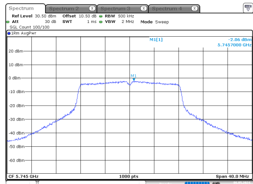
a_5745MHz_Chain 0
