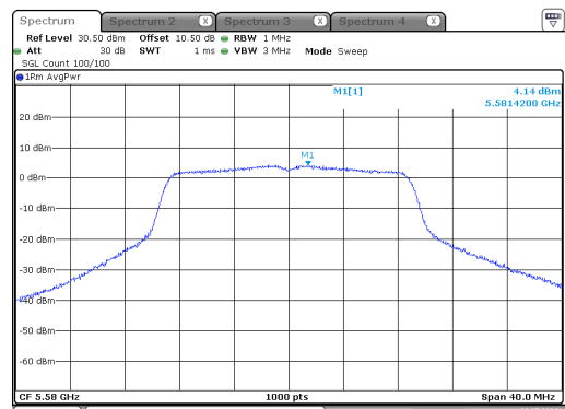
n20_5580MHz_Chain 0
