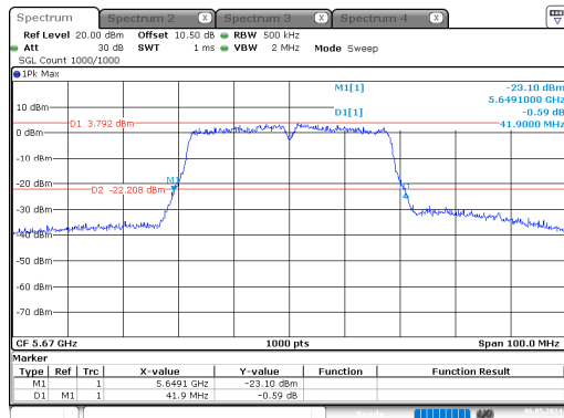
n40_5670MHz_Chain 0
