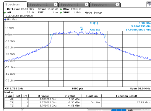
n20_5785MHz_Chain 0
