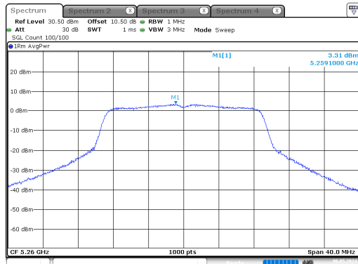
n20_5260MHz_Chain 0
