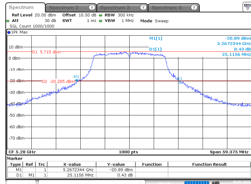
n20_5280MHz_Chain 0
