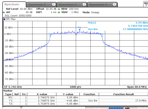
n20_5745MHz_Chain 0
