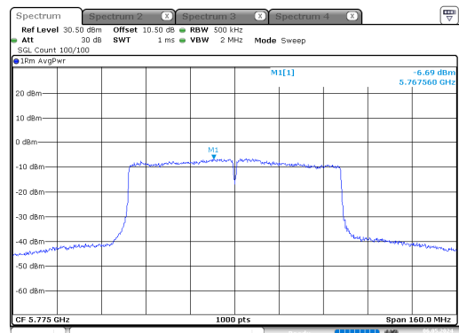
ac80_5775MHz_Chain 0
