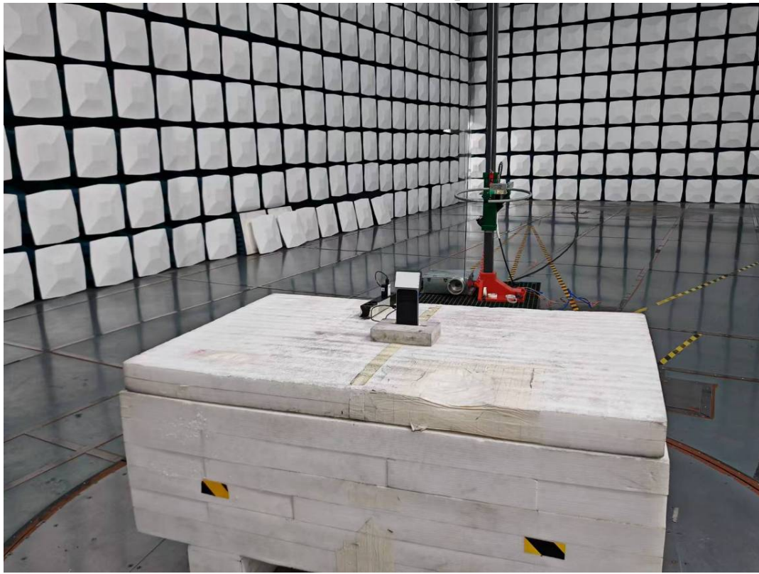
Radiated Emission 30M-1GHz front View M3
