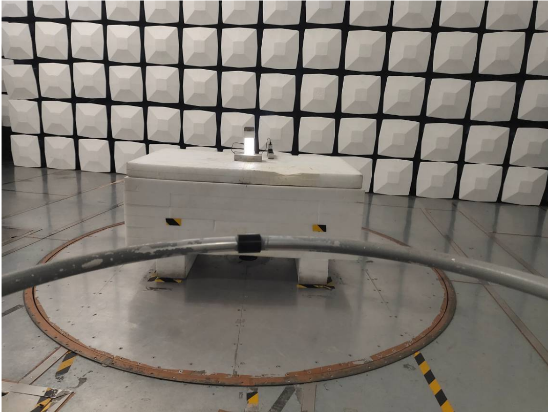
Radiated Emission 30M-1GHz front View M1
