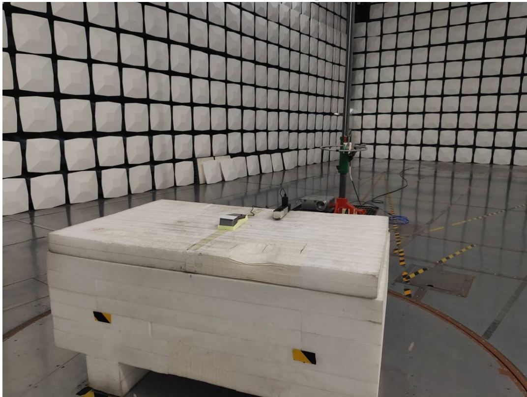
Radiated Emission 30M-1GHz front View M7
