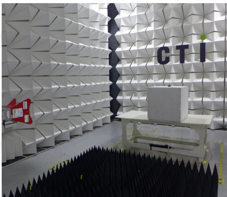
Radiated spurious emission Test Setup-2 (Above 1GHz)
