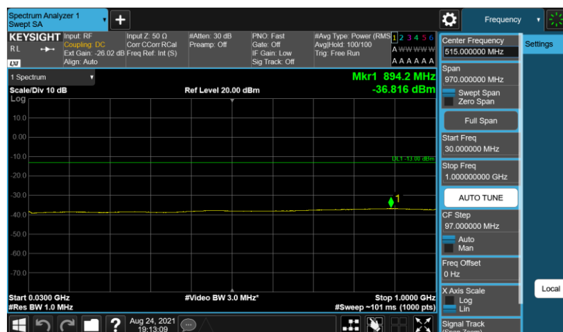
Band41-10MHz-256QAM-40620-E-TM3.1A-30~1000
