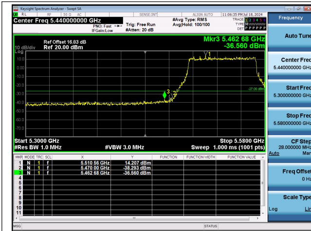
11AX80MIMO-Ant0-5530-PASS
