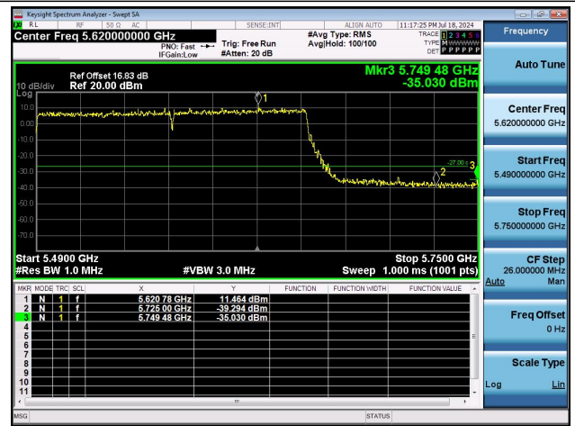
11AX160MIMO-Ant0-5570-PASS
