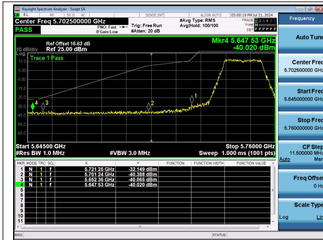
11AC20MIMO-Ant0-5745-PASS
