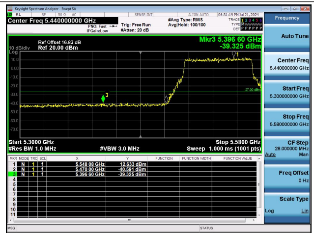
11AX80MIMO-Ant1-5530-PASS
