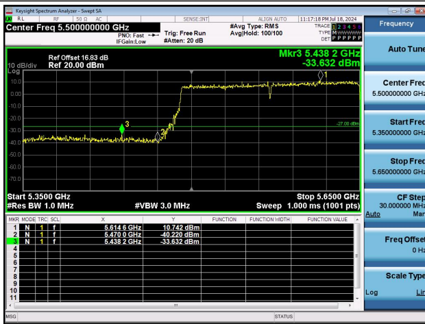
11AX160MIMO-Ant0-5570-PASS
