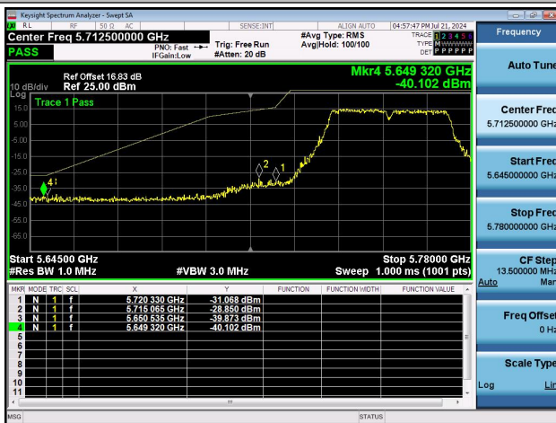
11N40MIMO-Ant0-5755-PASS
