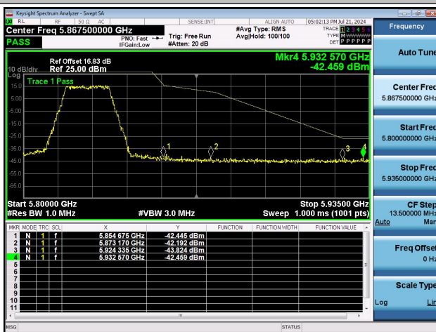
11AC20MIMO-Ant0-5825-PASS
