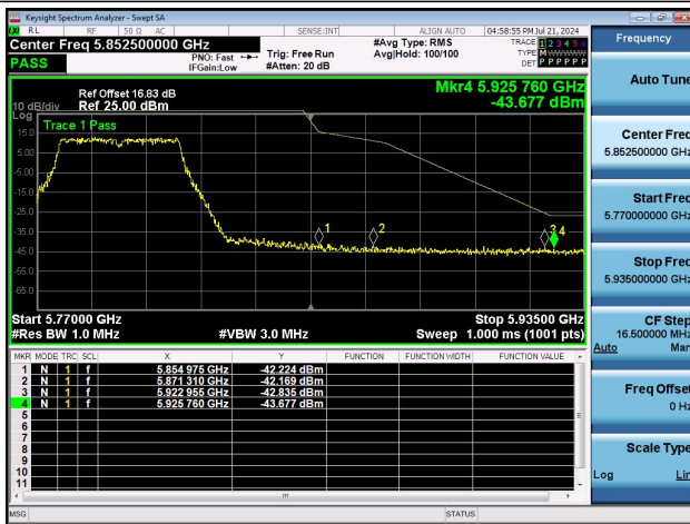
11N40MIMO-Ant0-5795-PASS
