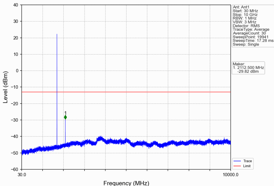
Band4_5MHz_16QAM_LCH_1712.5MHz_RB_1_0_NTNV
