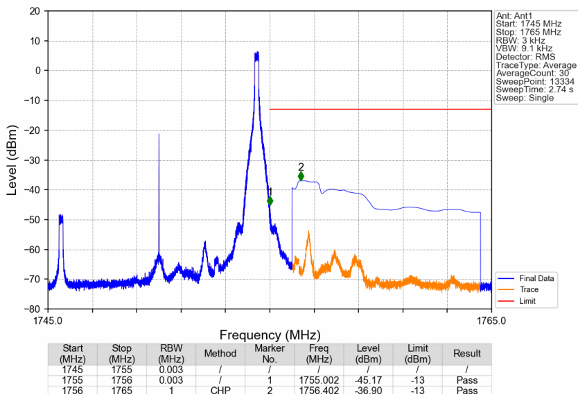
Band4_10MHz_16QAM_HCH_1750MHz_RB_1_49_NTNV
