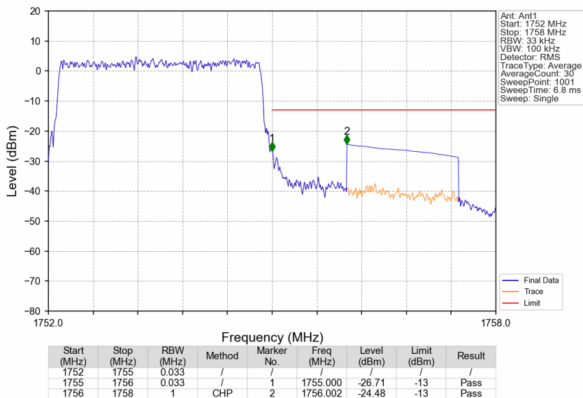
Band4_3MHz_16QAM_HCH_1753.5MHz_RB_15_0_NTNV
