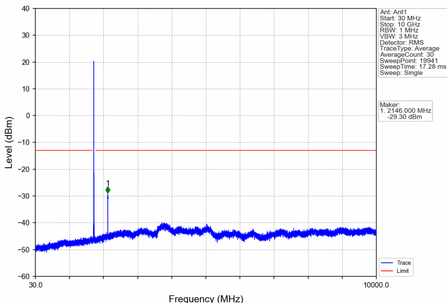
Band4_20MHz_16QAM_HCH_1745MHz_RB_1_0_NTNV
