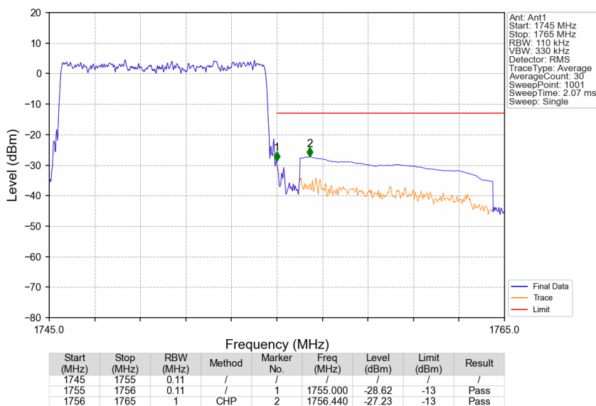
Band4_10MHz_16QAM_HCH_1750MHz_RB_50_0_NTNV
