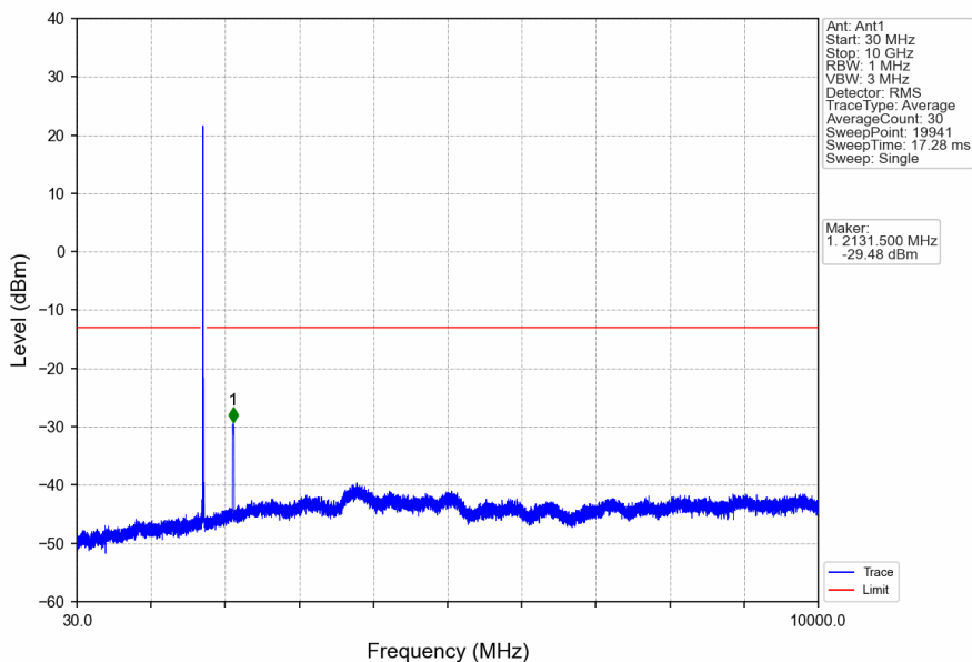
Band4_20MHz_16QAM_MCH_1732.5MHz_RB_1_0_NTNV
