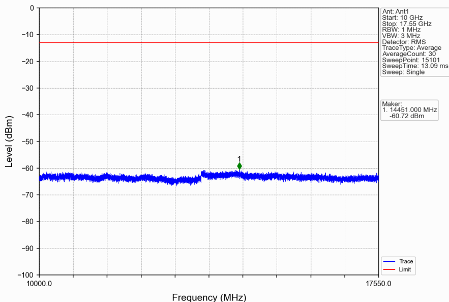
Band4_15MHz_QPSK_MCH_1732.5MHz_RB_1_0_NTNV
