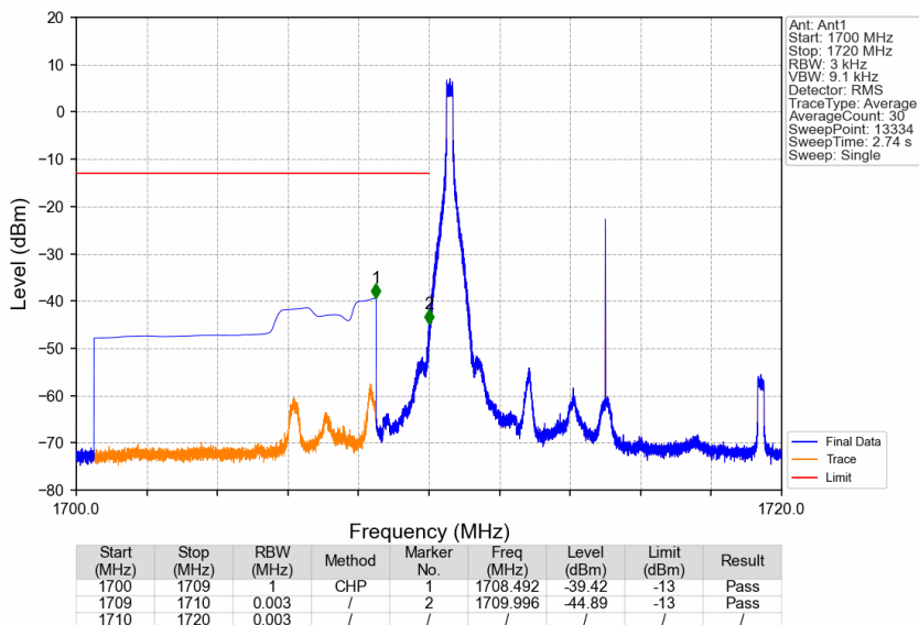
Band4_10MHz_16QAM_LCH_1715MHz_RB_1_0_NTNV
