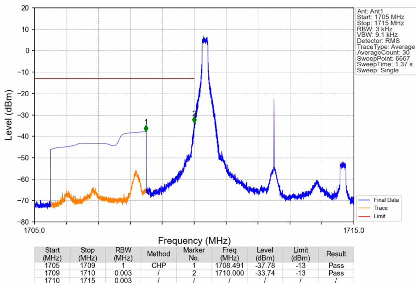
Band4_5MHz_16QAM_LCH_1712.5MHz_RB_1_0_NTNV
