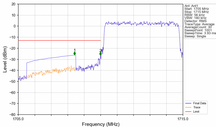
Band4_5MHz_16QAM_LCH_1712.5MHz_RB_25_0_NTNV
