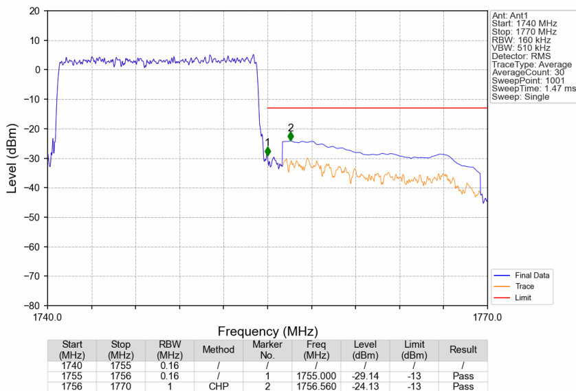
Band4_15MHz_QPSK_HCH_1747.5MHz_RB_75_0_NTNV
