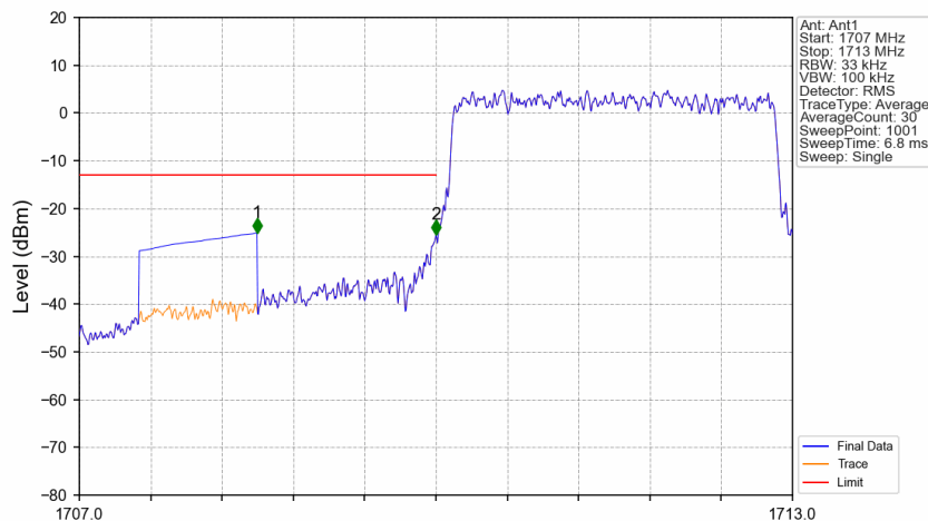
Band4_3MHz_16QAM_LCH_1711.5MHz_RB_15_0_NTNV
