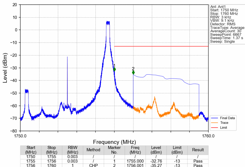
Band4_5MHz_QPSK_HCH_1752.5MHz_RB_1_24_NTNV
