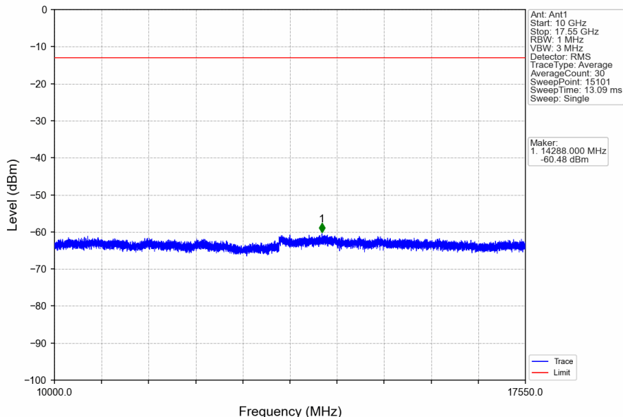
Band4_5MHz_16QAM_LCH_1712.5MHz_RB_25_0_NTNV
