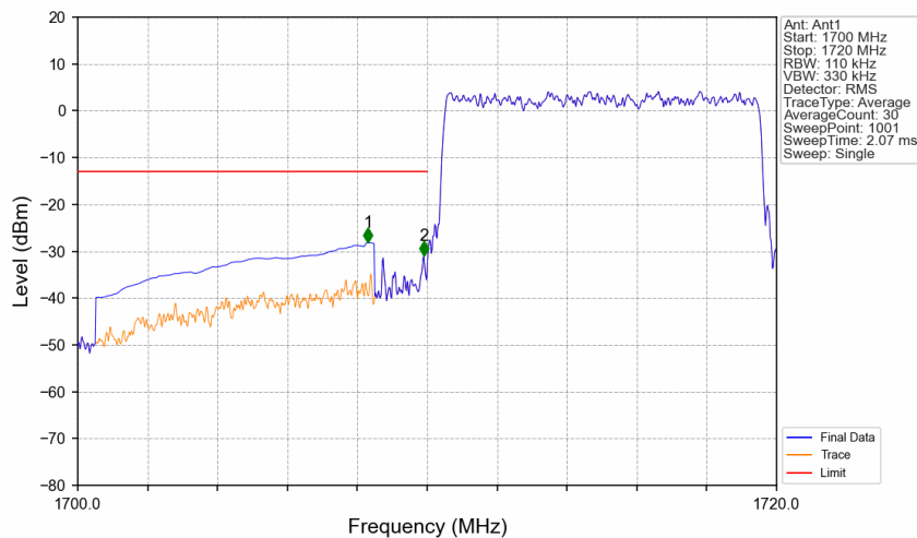
Band4_10MHz_16QAM_LCH_1715MHz_RB_50_0_NTNV
