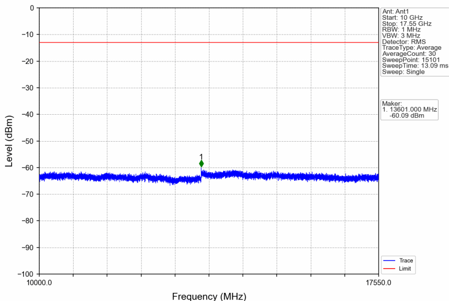
Band4_10MHz_16QAM_MCH_1732.5MHz_RB_1_0_NTNV
