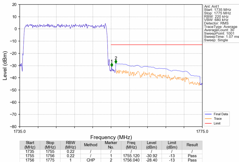
Band4_20MHz_16QAM_HCH_1745MHz_RB_100_0_NTNV
