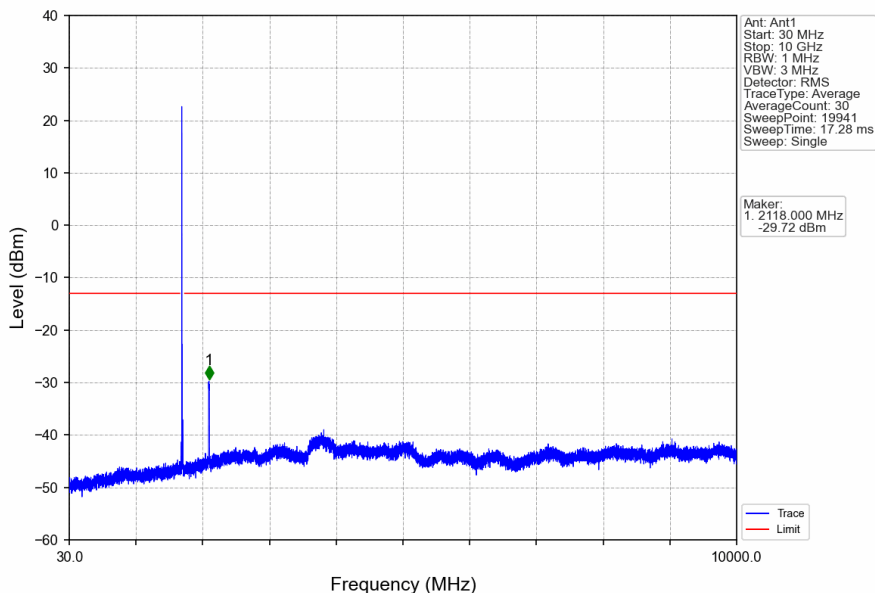
Band4_15MHz_16QAM_LCH_1717.5MHz_RB_1_0_NTNV
