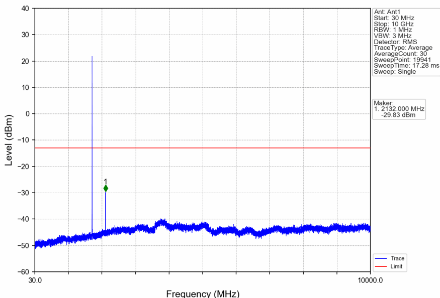
Band4_5MHz_16QAM_MCH_1732.5MHz_RB_1_0_NTNV
