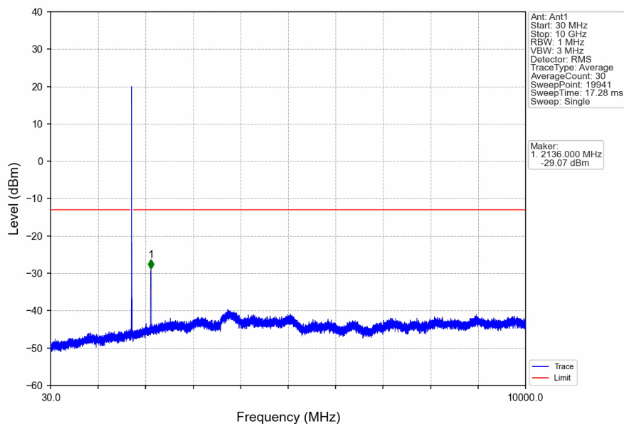
Band4_15MHz_16QAM_MCH_1732.5MHz_RB_1_0_NTNV
