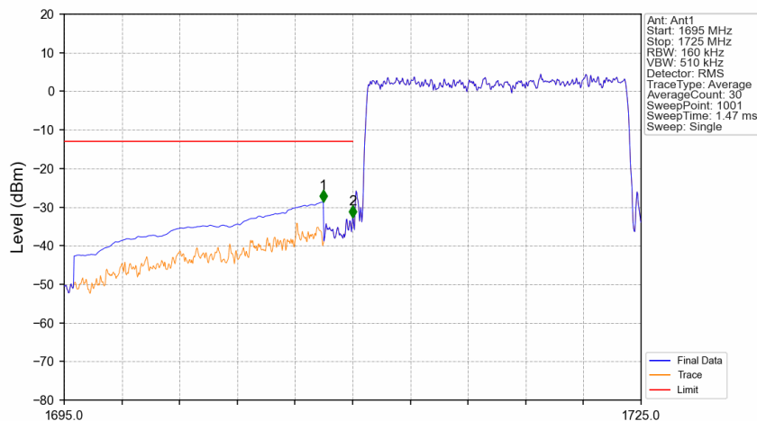
Band4_15MHz_16QAM_LCH_1717.5MHz_RB_75_0_NTNV
