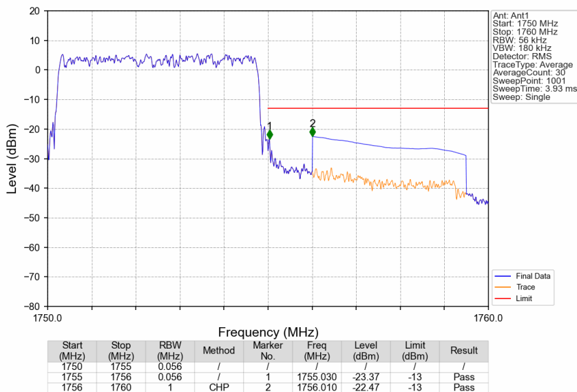
Band4_5MHz_QPSK_HCH_1752.5MHz_RB_25_0_NTNV
