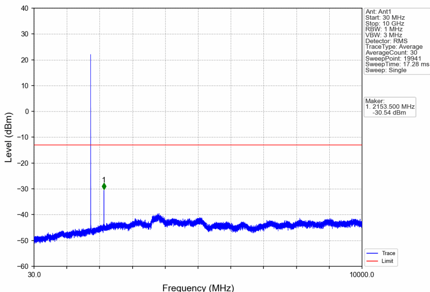
Band4_3MHz_16QAM_HCH_1753.5MHz_RB_1_0_NTNV
