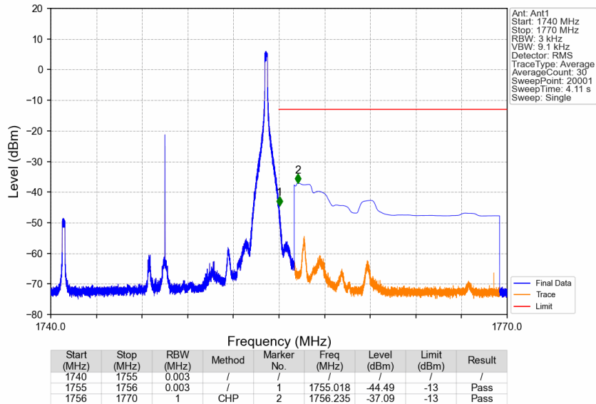
Band4_15MHz_16QAM_HCH_1747.5MHz_RB_1_74_NTNV
