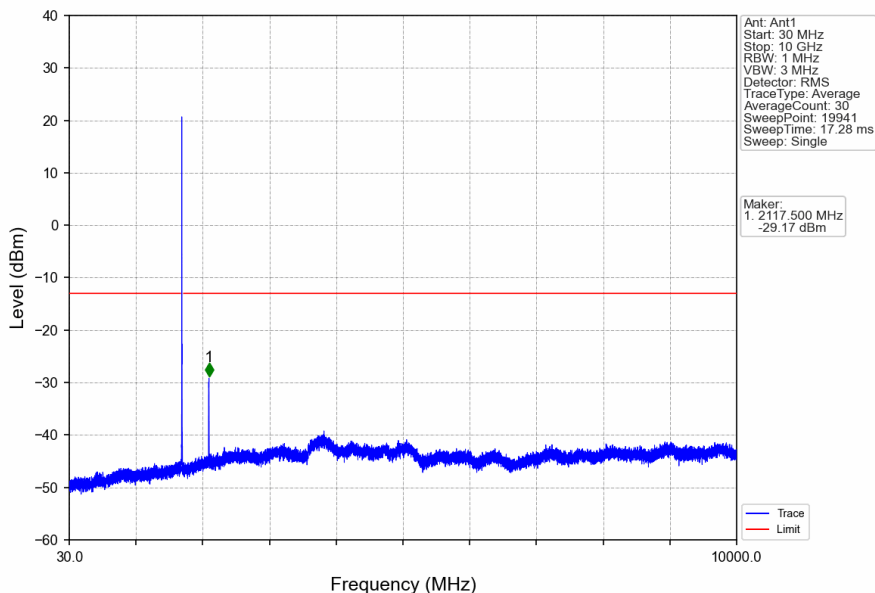
Band4_10MHz_16QAM_LCH_1715MHz_RB_1_0_NTNV
