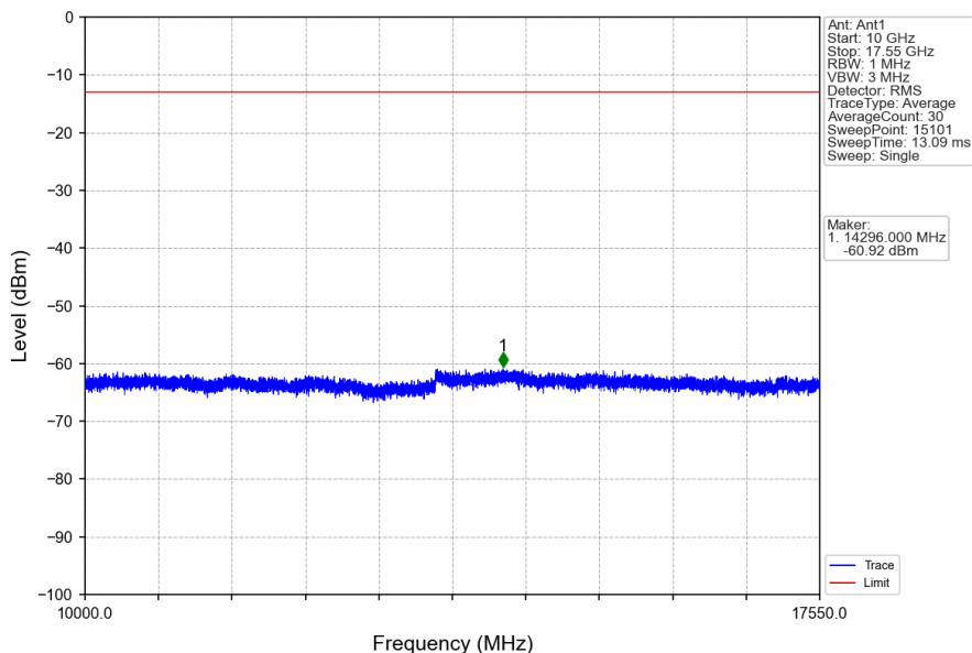
Band4_5MHz_QPSK_MCH_1732.5MHz_RB_1_0_NTNV
