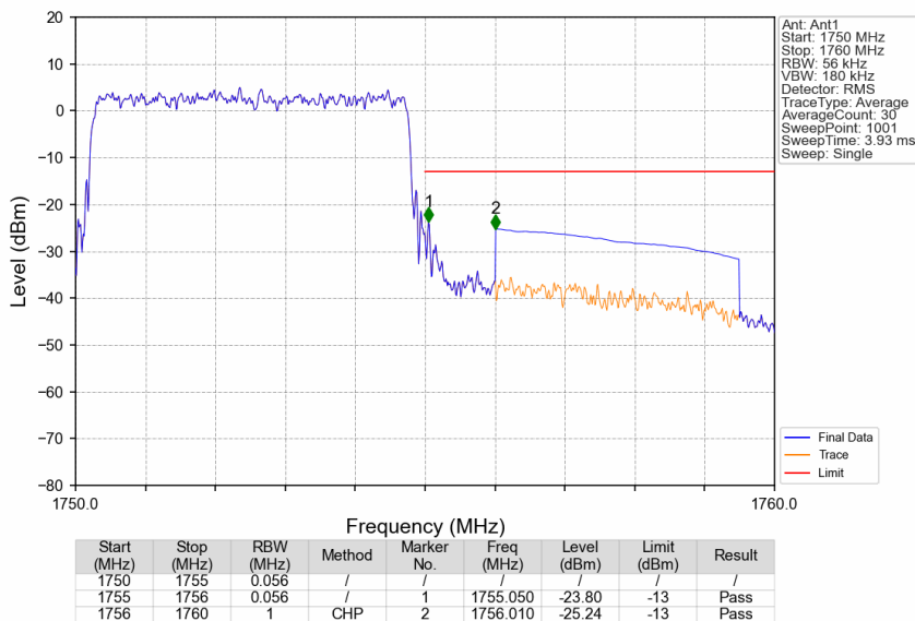
Band4_5MHz_16QAM_HCH_1752.5MHz_RB_25_0_NTNV
