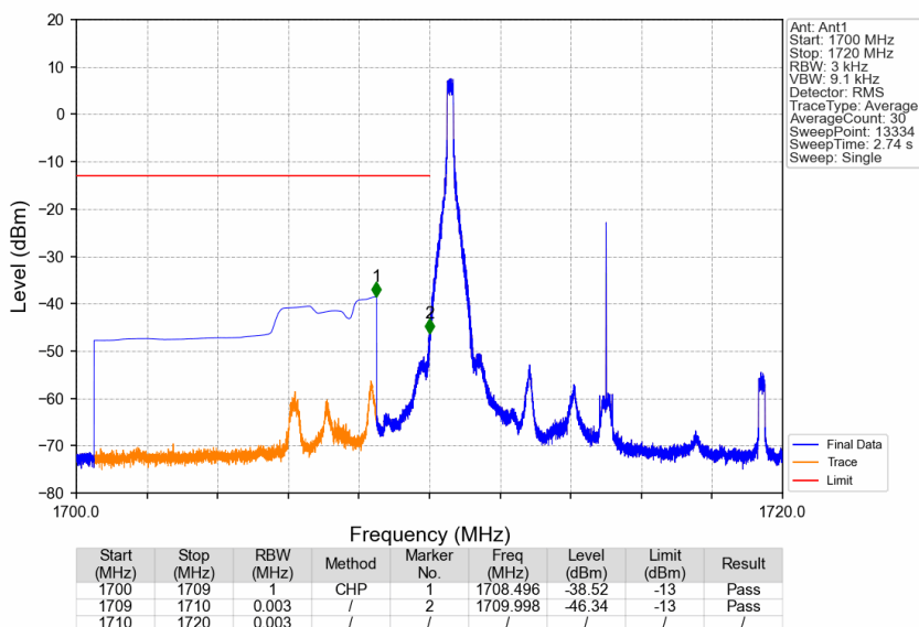
Band4_10MHz_QPSK_LCH_1715MHz_RB_1_0_NTNV
