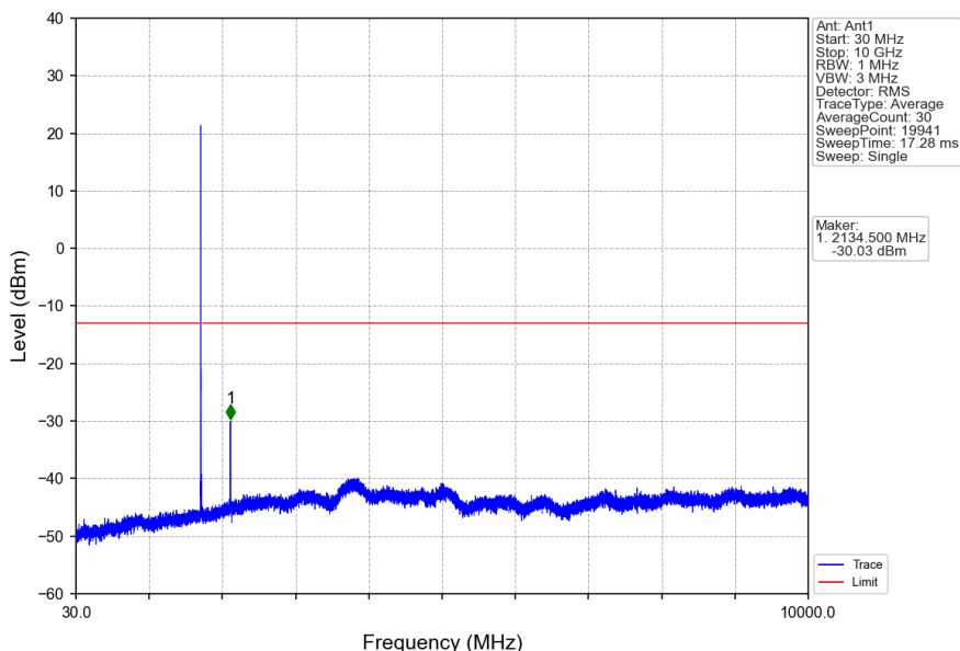
Band4_10MHz_16QAM_MCH_1732.5MHz_RB_1_0_NTNV
