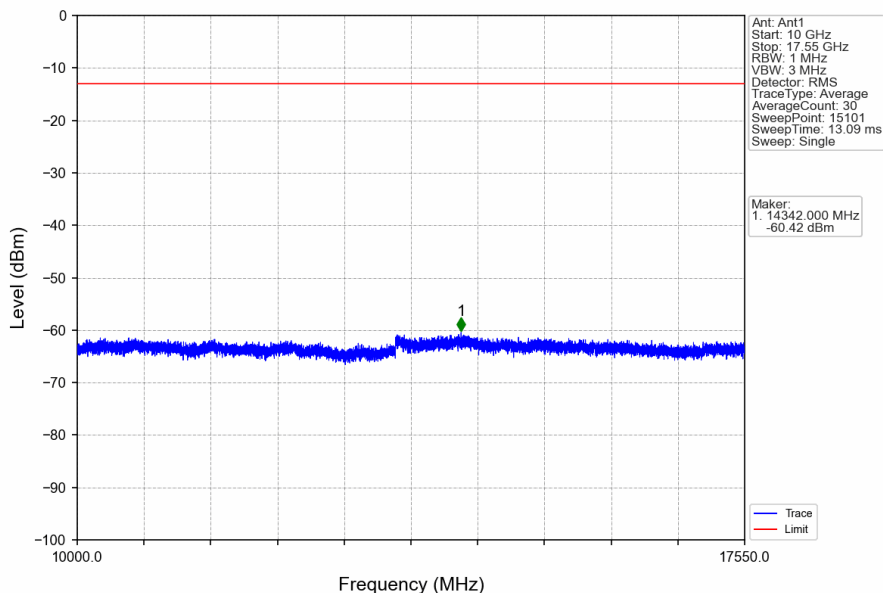
Band4_5MHz_16QAM_HCH_1752.5MHz_RB_1_0_NTNV
