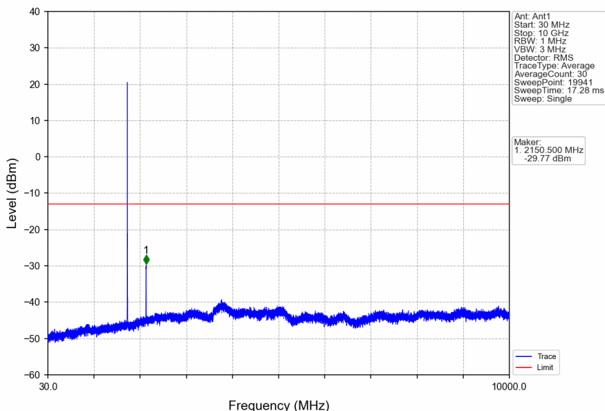
Band4_10MHz_16QAM_HCH_1750MHz_RB_1_0_NTNV
