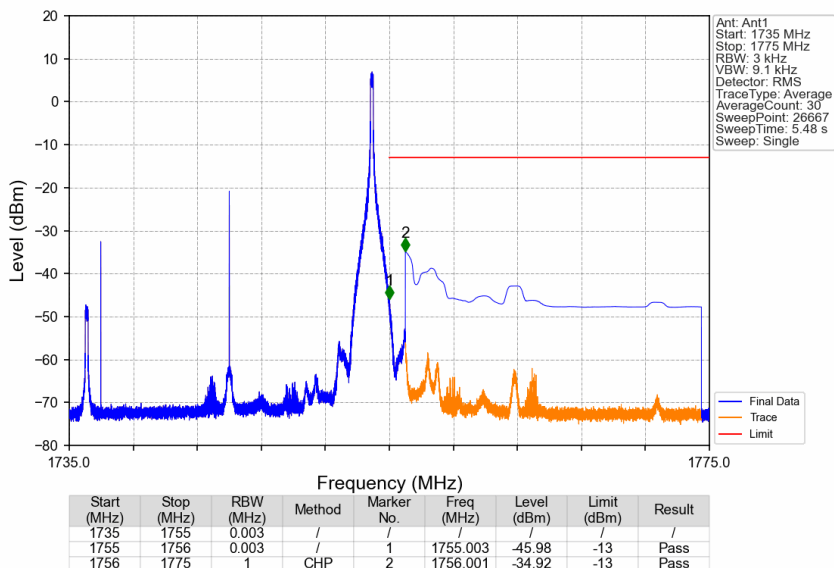
Band4_20MHz_16QAM_HCH_1745MHz_RB_1_99_NTNV
