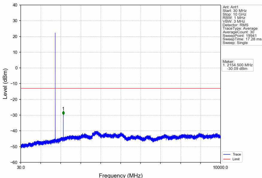
Band4_5MHz_16QAM_HCH_1752.5MHz_RB_1_0_NTNV
