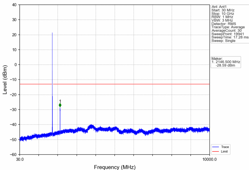
Band4_15MHz_16QAM_HCH_1747.5MHz_RB_1_0_NTNV
