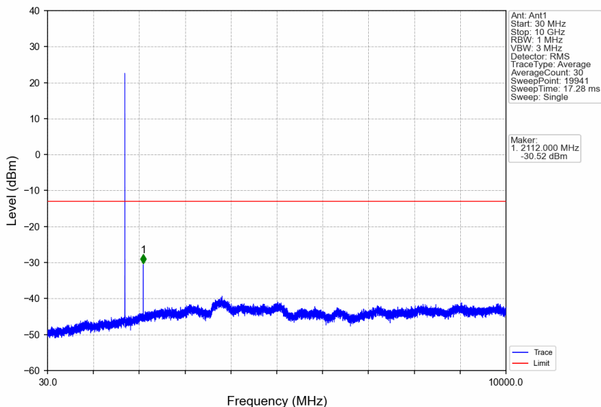
Band4_3MHz_16QAM_LCH_1711.5MHz_RB_1_0_NTNV
