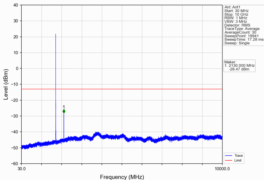
Band4_10MHz_QPSK_MCH_1732.5MHz_RB_1_0_NTNV
