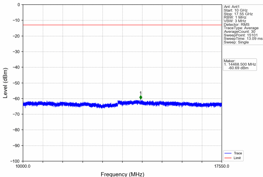
Band4_3MHz_16QAM_HCH_1753.5MHz_RB_1_0_NTNV
