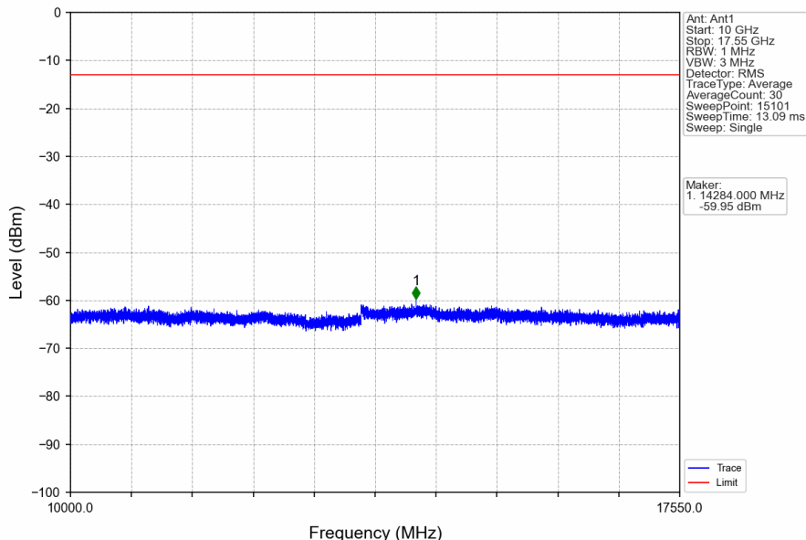
Band4_10MHz_QPSK_LCH_1715MHz_RB_50_0_NTNV
