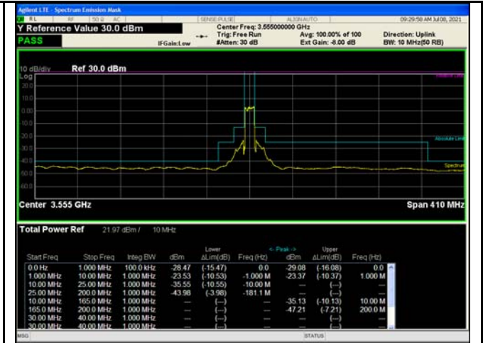
10MHz - Low CH QPSK - Chain 1
