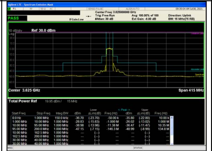
15MHz - Middle CH QPSK - Chain 1
