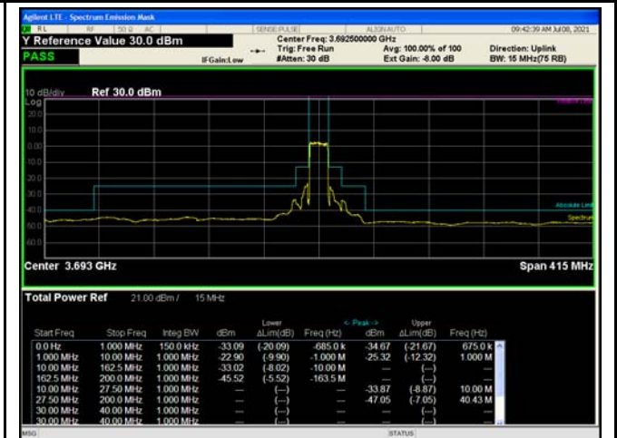
15MHz - High CH QPSK - Chain 1
