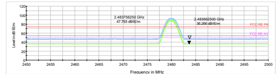
Bluetooth LE (1M) Channel 39 Peak+Average
