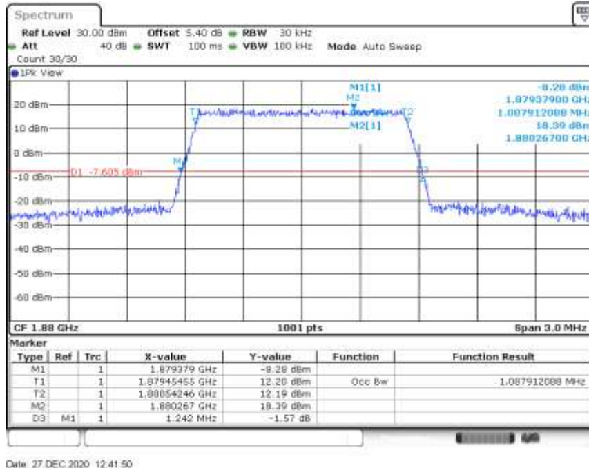
Band2-1.4MHz-QPSK-18900-6RB#0-1.088
