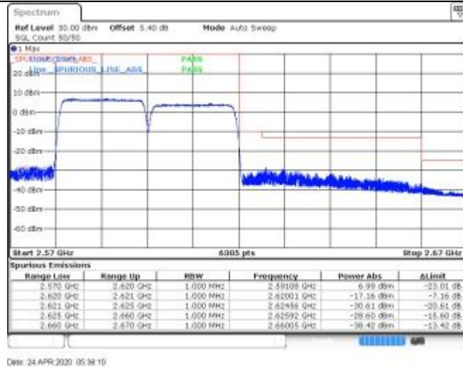
CA_38C_100RB+100RB_QPSK_37952+38150_100RB#0+100RB#0
