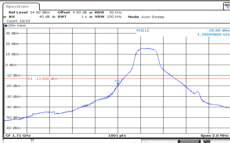
Band4-1.4MHz-QPSK-19957-1RB#0
