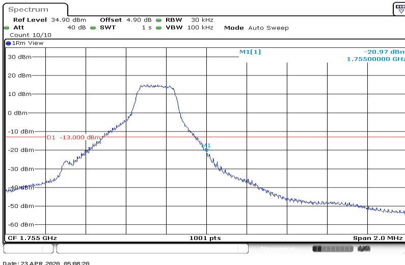
Band4-1.4MHz-16QAM-20393-6RB#0
