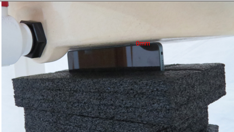
Picture 15: Left Edge, the distance from EUT to the bottom of the Phantom is 0mm
