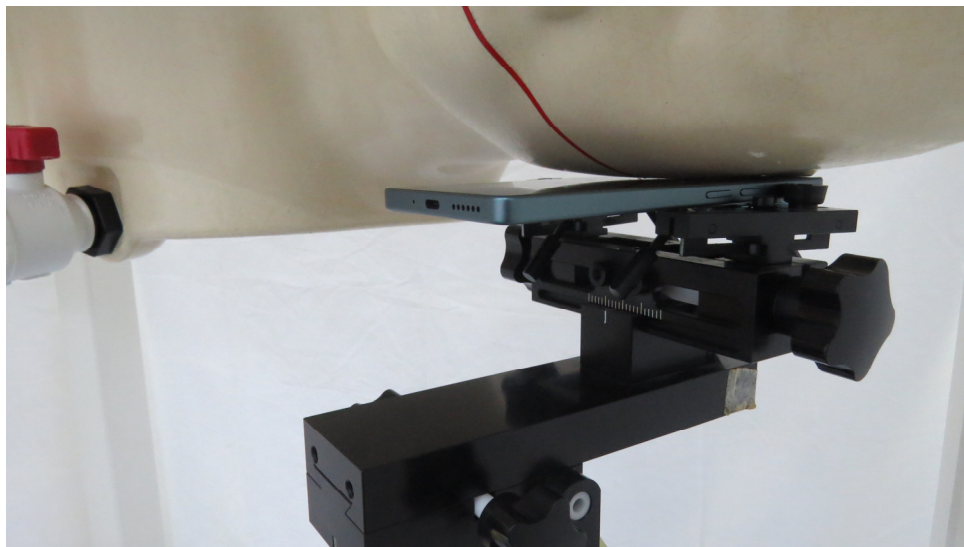
Picture 1: Left Hand Touch Cheek Position
