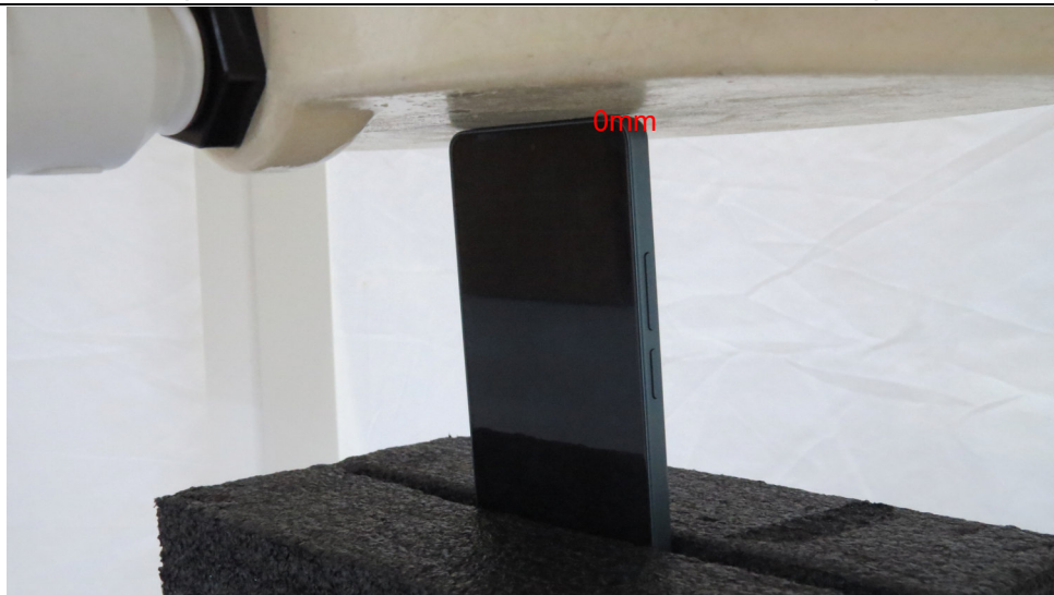
Picture 17: Top Edge, the distance from EUT to the bottom of the Phantom is 0mm
