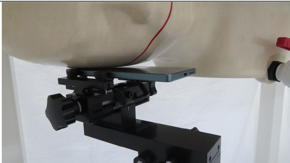
Picture 3: Right Hand Touch Cheek Position
