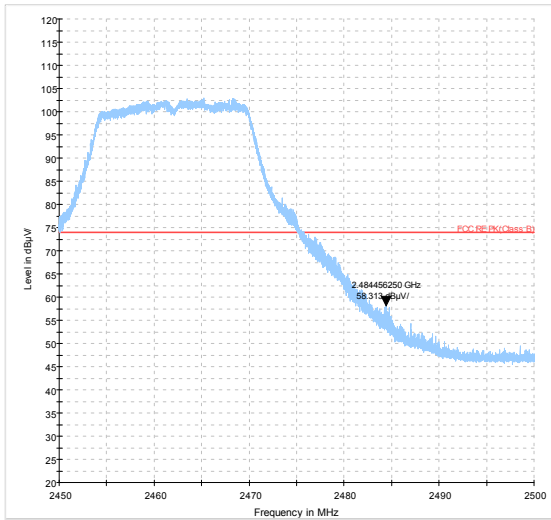
802.11g-Channel 11 Peak
