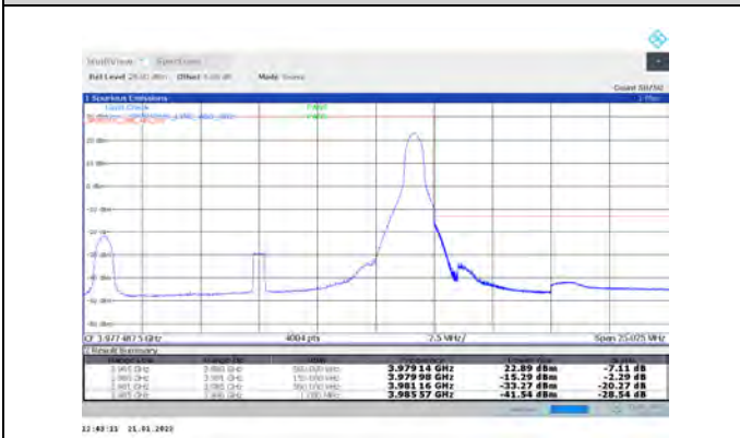
1-N77-3700-3980-PC3-30-15-H-2-DFT-PI2BPSK-Edge_1RB_Right-1@37-Ant1-PASS-see graph
