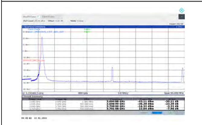
1-N77-3700-3980-PC3-30-80-L-4-CP-QPSK-Edge_1RB_Left-1@0-Ant1-PASS-see graph
