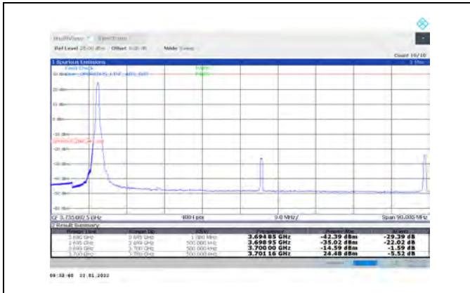
1-N77-3700-3980-PC3-30-80-L-1-DFT-PI2BPSK-Edge_1RB_Left-1@0-Ant1-PASS-see graph
