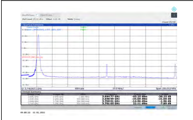
1-N77-3700-3980-PC3-30-90-L-4-CP-QPSK-Edge_1R B_Left-1@0-Ant1-PASS-see graph
