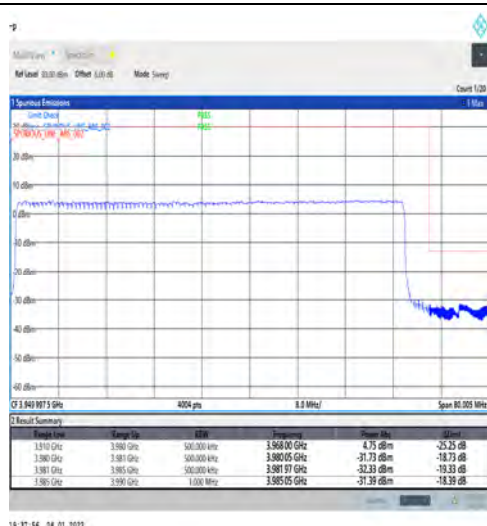
1-N77-3700-3980-PC3-30-70-H-3-DFT-PI2BPSK-Outer_Full-180@0-Ant1-PASS-see graph
