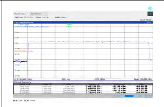
1-N77-3700-3980-PC3-30-90-L-3-DFT-PI2BPSK-Outer_Full-240@0-Ant1-PASS-see graph
