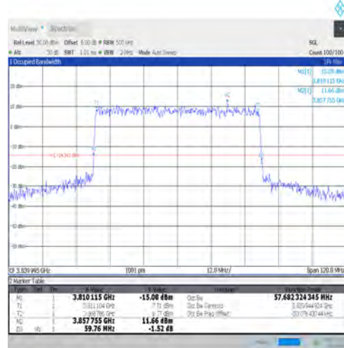
1-N77-3700-3980-PC3-30-60-M-8-CP-64QAM-Outer_Full-162@0-Ant1-57.682-59.760-≤60-PASS
