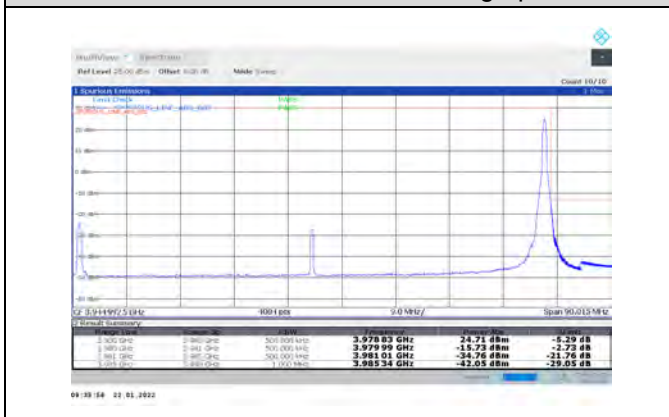
1-N77-3700-3980-PC3-30-80-H-2-DFT-PI2BPSK-Edge_1RB_Right-1@216-Ant1-PASS-see graph
