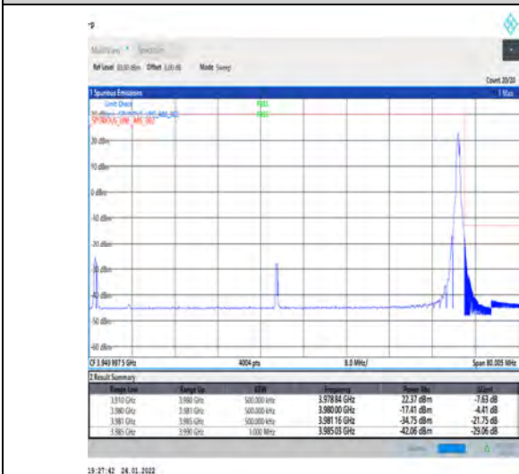
1-N77-3700-3980-PC3-30-70-H-5-CP-QPSK-Edge_1RB_Right-1@188-Ant1-PASS-see graph
