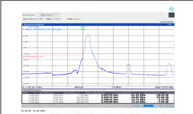
1-N77-3700-3980-PC3-30-15-L-4-CP-QPSK-Edge_1R_B_Left-1@0-Ant1-PASS-see graph
