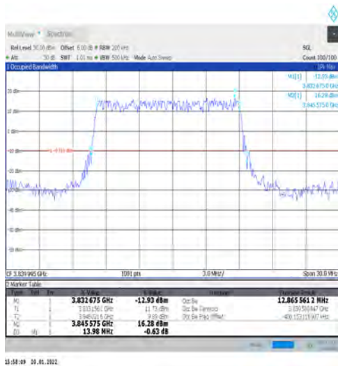
1-N77-3700-3980-PC3-30-15-M-2-DFT-PI2BPSK-Outer_Full-36@0-Ant1-12.866-13.980-≤15-PASS
