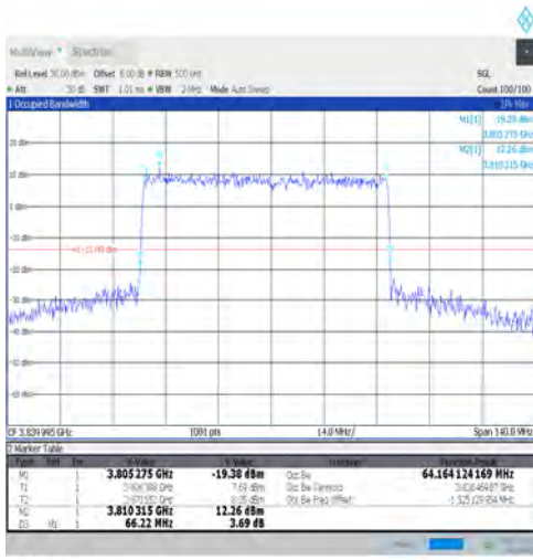
1-N77-3700-3980-PC3-30-70-M-4-DFT-64QAM-Outer_Full-Outer_Full@N/A-Ant1-64.164-66.220-≤70-PA SS
