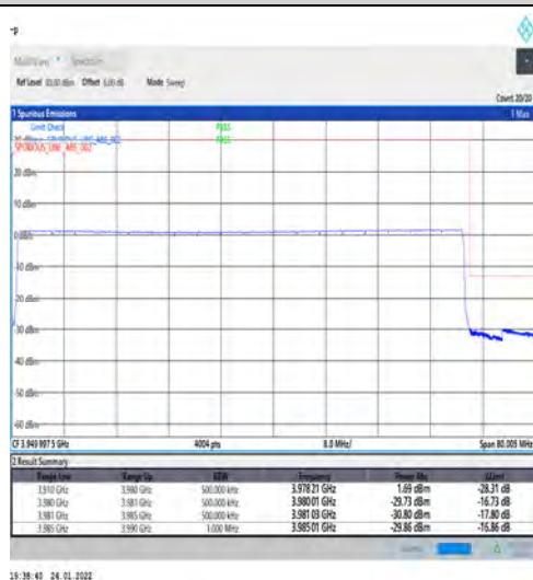
1-N77-3700-3980-PC3-30-70-H-6-CP-QPSK-Outer_Full-189@0-Ant1-PASS-see graph
