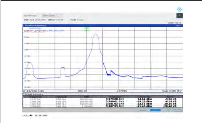
1-N77-3700-3980-PC3-30-10-H-2-DFT-PI2BPSK-Edge_1RB_Right-1@23-Ant1-PASS-see graph
