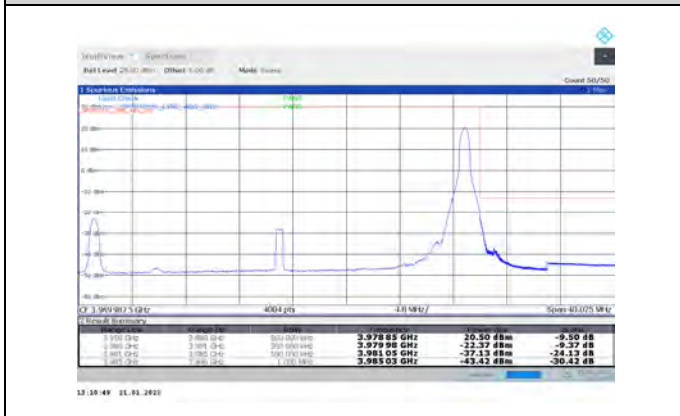
1-N77-3700-3980-PC3-30-30-H-5-CP-QPSK-Edge_1RB_Right-1@77-Ant1-PASS-see graph
