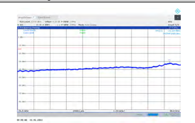
1-N77-3700-3980-PC3-30-100-H-1-DFT-PI2BPSK-E dge_1RB_Left-1@0-26500-40000
