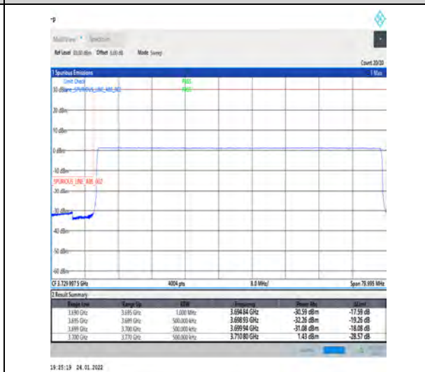
1-N77-3700-3980-PC3-30-70-L-6-CP-QPSK-Outer_Full-189@0-Ant1-PASS-see graph
