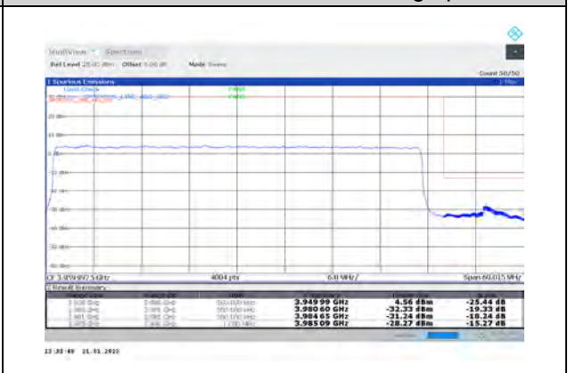
1-N77-3700-3980-PC3-30-50-H-3-DFT-PI2BPSK-Outer_Full-128@0-Ant1-PASS-see graph
