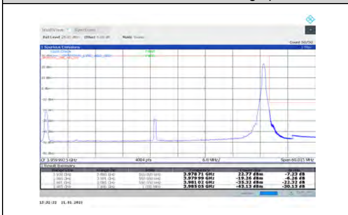
1-N77-3700-3980-PC3-30-50-H-2-DFT-PI2BPSK-Edge_1RB_Right-1@132-Ant1-PASS-see graph
