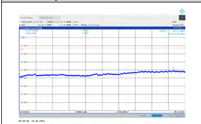
1-N77-3700-3980-PC3-30-100-H-1-DFT-PI2BPSK-E dge_1RB_Left-1@0-6000-26500
