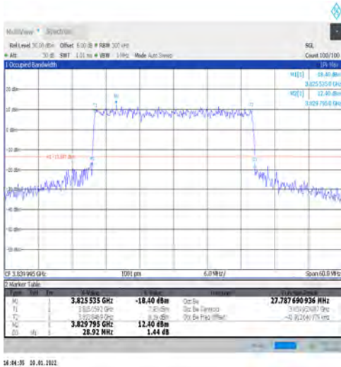
1-N77-3700-3980-PC3-30-30-M-8-CP-64QAM-Outer_Full-78@0-Ant1-27.788-28.920-≤30-PASS
