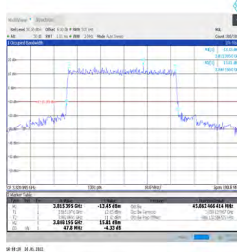
1-N77-3700-3980-PC3-30-50-M-1-DFT-QPSK-Outer_Full-128@0-Ant1-45.862-47.800-≤50-PASS
