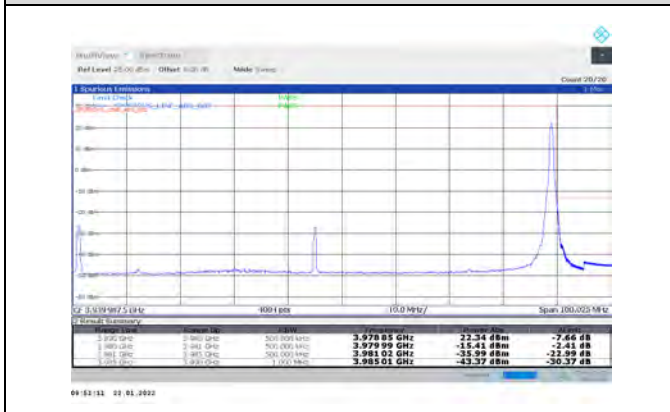
1-N77-3700-3980-PC3-30-90-H-5-CP-QPSK-Edge_1RB_Right-1@244-Ant1-PASS-see graph
