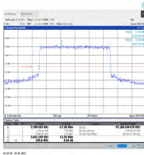
1-N77-3700-3980-PC3-30-100-M-6-CP-QPSK-Outer _Full-273@0-Ant1-97.266-100.800-≤100-PASS
