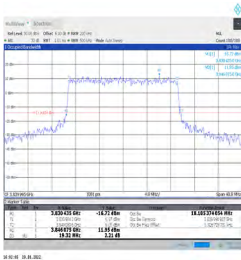
1-N77-3700-3980-PC3-30-20-M-7-CP-16QAM-Outer_Full-51@0-Ant1-18.185-19.320-≤20-PASS
