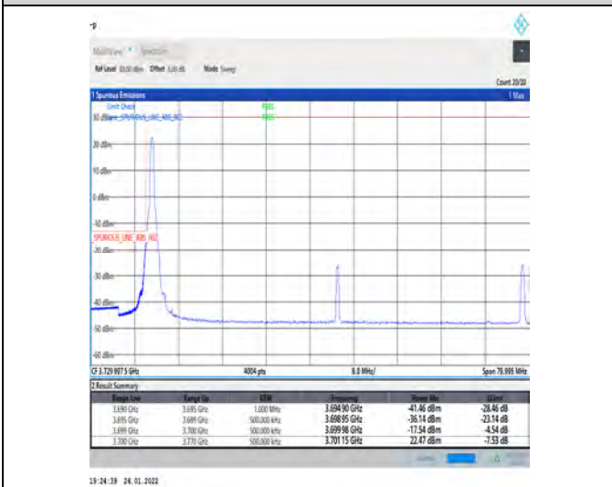
1-N77-3700-3980-PC3-30-70-L-4-CP-QPSK-Edge_1RB_Left-1@0-Ant1-PASS-see graph
