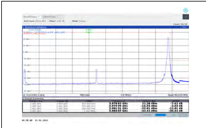
1-N77-3700-3980-PC3-30-80-H-5-CP-QPSK-Edge_1 RB_Right-1@216-Ant1-PASS-see graph
