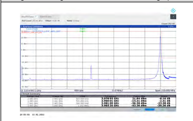
1-N77-3700-3980-PC3-30-100-H-5-CP-QPSK-Edge_1 RB_Right-1@272-Ant1-PASS-see graph
