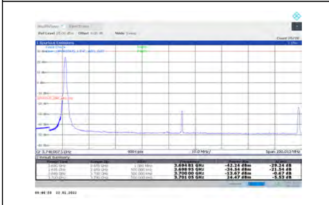
1-N77-3700-3980-PC3-30-90-L-1-DFT-PI2BPSK-Edge_1RB_Left-1@0-Ant1-PASS-see graph
