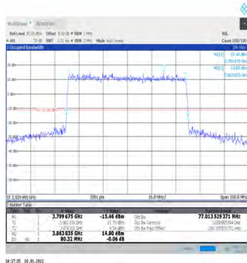
1-N77-3700-3980-PC3-30-80-M-4-DFT-64QAM-Outer_Full-216@0-Ant1-77.014-80.320-≤80-PASS
