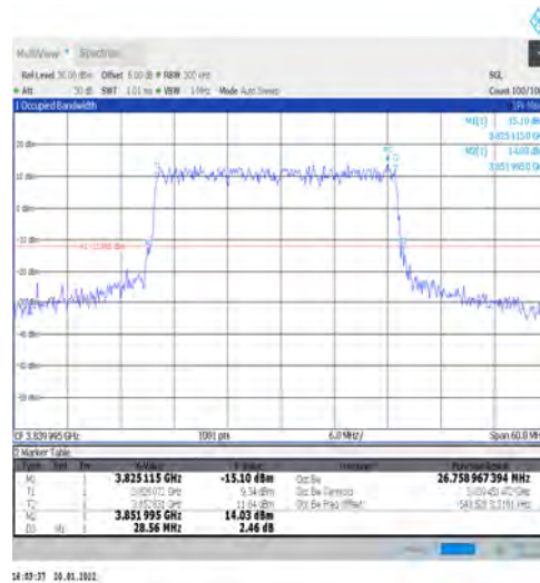
1-N77-3700-3980-PC3-30-30-M-3-DFT-16QAM-Outer_Full-75@0-Ant1-26.761-28.560-≤30-PASS
