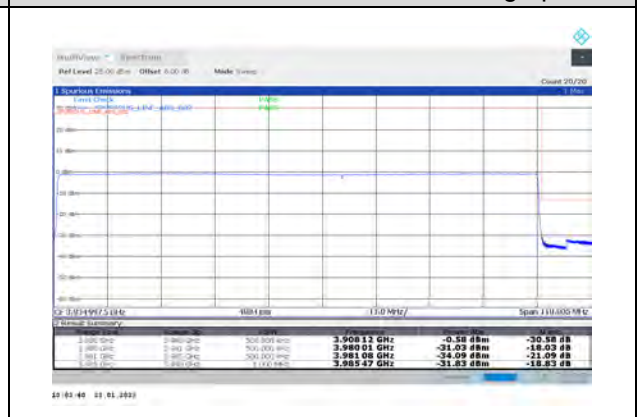
1-N77-3700-3980-PC3-30-100-H-6-CP-QPSK-Outer_Full-273@0-Ant1-PASS-see graph
