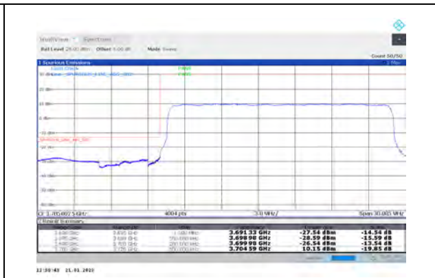
1-N77-3700-3980-PC3-30-20-L-3-DFT-PI2BPSK-Outer_Full-50@0-Ant1-PASS-see graph
