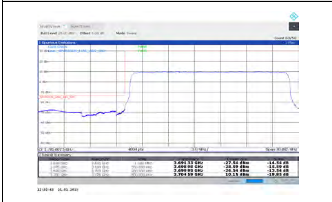
1-N77-3700-3980-PC3-30-20-L-4-CP-QPSK-Edge_1RB_Left-1@0-Ant1-PASS-see graph
