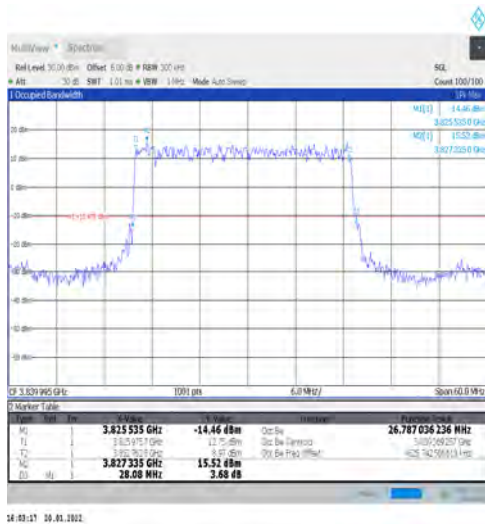
1-N77-3700-3980-PC3-30-30-M-2-DFT-PI2BPSK-Outer_Full-75@0-Ant1-26.79-28.080-≤30-PASS
