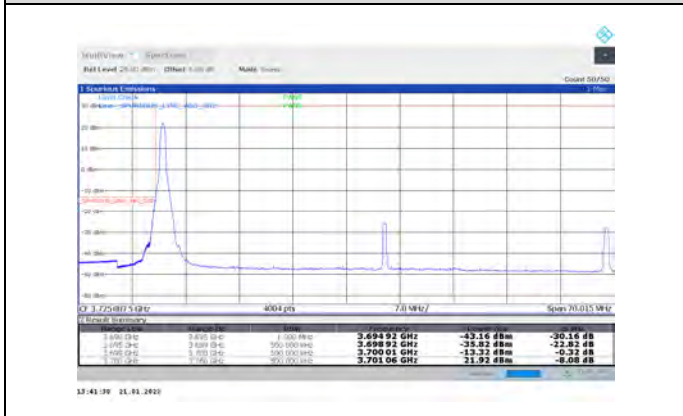
1-N77-3700-3980-PC3-30-60-L-4-CP-QPSK-Edge_1R_B_Left-1@0-Ant1-PASS-see graph
