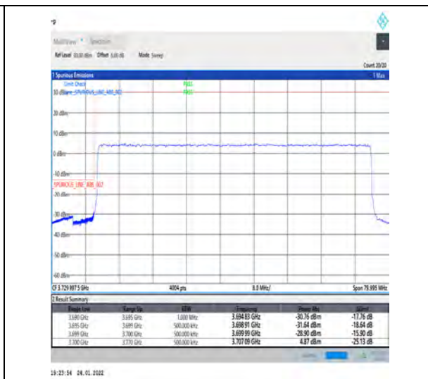
1-N77-3700-3980-PC3-30-70-L-3-DFT-PI2BPSK-Outer_Full-180@0-Ant1-PASS-see graph
