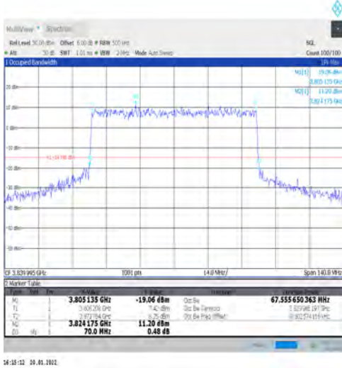
1-N77-3700-3980-PC3-30-70-M-6-CP-QPSK-Outer_Full-Outer_Full@N/A-Ant1-67.556-70.000-≤70-PASS
