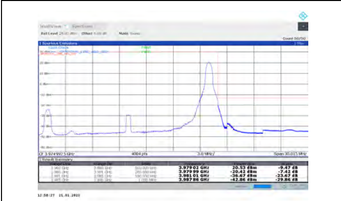
1-N77-3700-3980-PC3-30-20-H-5-CP-QPSK-Edge_1R_B_Right-1@50-Ant1-PASS-see graph
