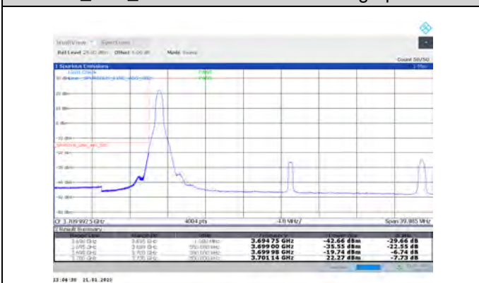
1-N77-3700-3980-PC3-30-30-L-4-CP-QPSK-Edge_1R_B_Left-1@0-Ant1-PASS-see graph
