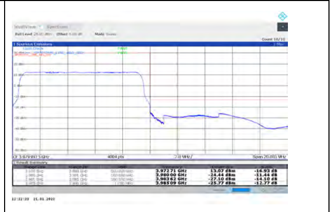
1-N77-3700-3980-PC3-30-10-H-3-DFT-PI2BPSK-Outer_Full-24@0-Ant1-PASS-see graph
