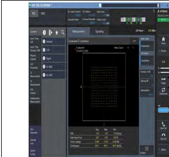
1-N77-3700-3980-PC3-30-100-M-5-DFT-256QAM-Outer_Full-270@0-Ant1-see graph-PASS
