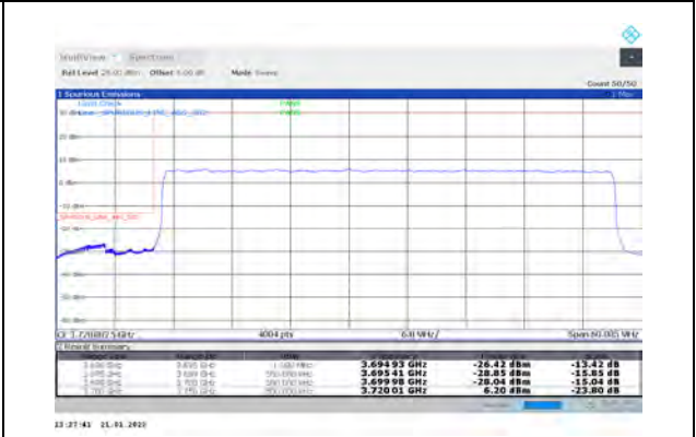
1-N77-3700-3980-PC3-30-50-L-3-DFT-PI2BPSK-Outer_Full-128@0-Ant1-PASS-see graph
