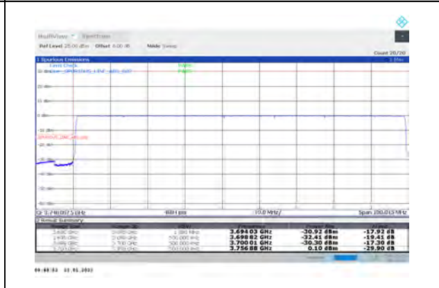
1-N77-3700-3980-PC3-30-90-L-6-CP-QPSK-Outer_Full-245@0-Ant1-PASS-see graph
