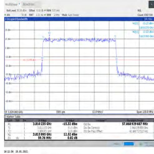
1-N77-3700-3980-PC3-30-60-M-4-DFT-64QAM-Outer_Full-162@0-Ant1-57.869-59.760-≤60-PASS
