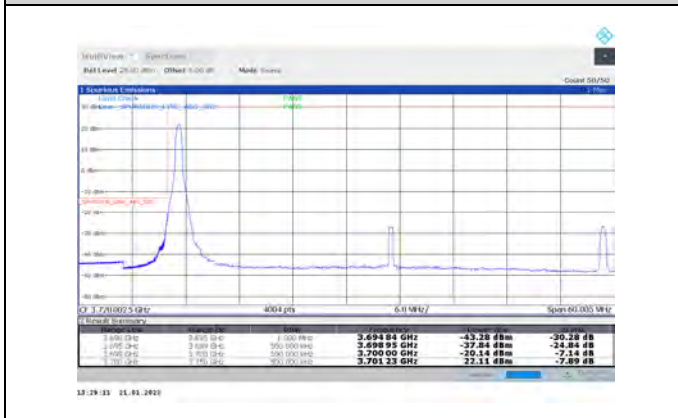
1-N77-3700-3980-PC3-30-50-L-4-CP-QPSK-Edge_1RB_Left-1@0-Ant1-PASS-see graph
