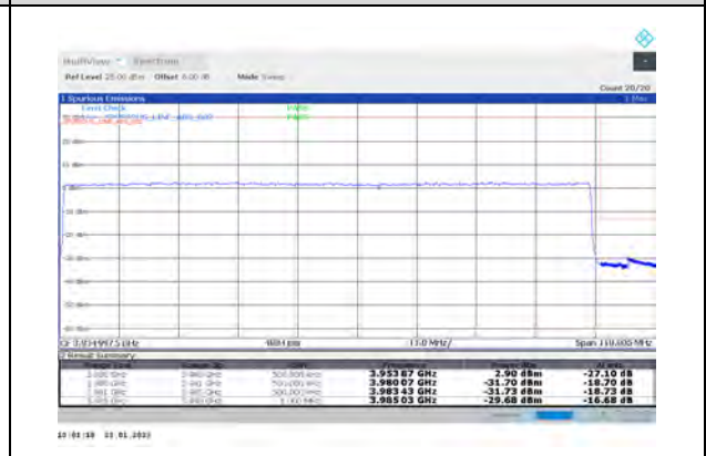
1-N77-3700-3980-PC3-30-100-H-3-DFT-PI2BPSK-Outer_Full-270@0-Ant1-PASS-see graph
