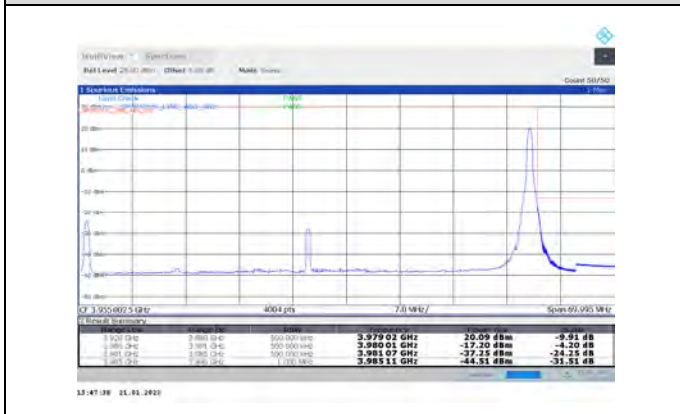
1-N77-3700-3980-PC3-30-60-H-5-CP-QPSK-Edge_1RB_Right-1@161-Ant1-PASS-see graph
