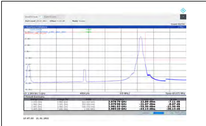
1-N77-3700-3980-PC3-30-30-H-2-DFT-PI2BPSK-Edge_1RB_Right-1@77-Ant1-PASS-see graph
