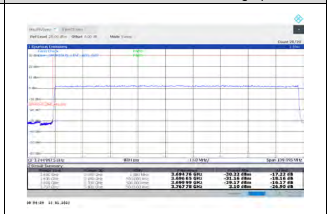
1-N77-3700-3980-PC3-30-100-L-3-DFT-PI2BPSK-Outer_Full-270@0-Ant1-PASS-see graph
