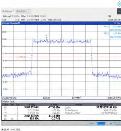
1-N77-3700-3980-PC3-30-60-M-5-DFT-256QAM-Outer_Full-162@0-Ant1-57.776-60.000-≤60-PASS
