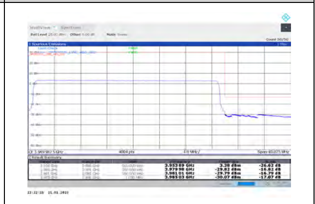
1-N77-3700-3980-PC3-30-30-H-6-CP-QPSK-Outer_Full-78@0-Ant1-PASS-see graph
