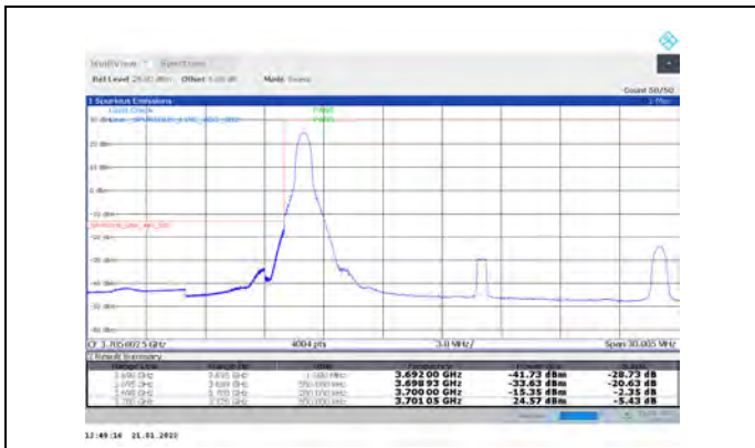
1-N77-3700-3980-PC3-30-20-L-1-DFT-PI2BPSK-Edge_1RB_Left-1@0-Ant1-PASS-see graph
