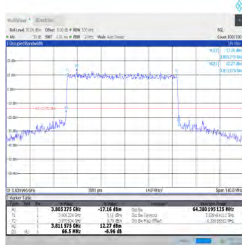
1-N77-3700-3980-PC3-30-70-M-3-DFT-16QAM-Outer_Full-Outer_Full@N/A-Ant1-64.38-66.500-≤70-PA SS
