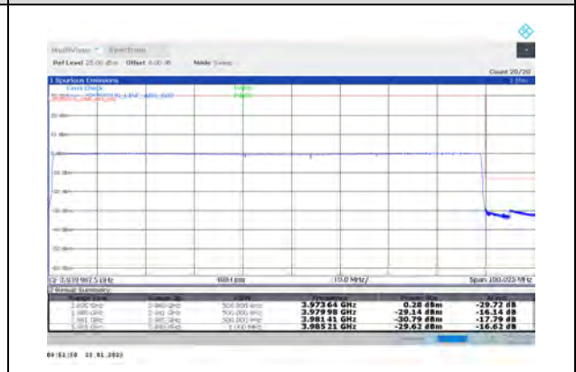
1-N77-3700-3980-PC3-30-90-H-6-CP-QPSK-Outer_Full-245@0-Ant1-PASS-see graph
