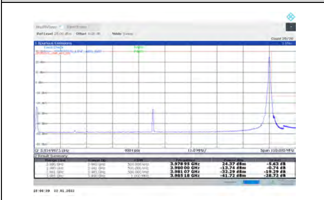
1-N77-3700-3980-PC3-30-100-H-2-DFT-PI2BPSK-Edge_1RB_Right-1@272-Ant1-PASS-see graph
