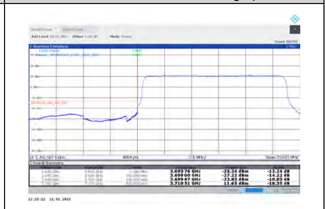
1-N77-3700-3980-PC3-30-15-L-3-DFT-PI2BPSK-Outer_Full-36@0-Ant1-PASS-see graph
