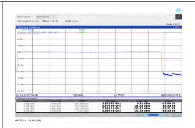
1-N77-3700-3980-PC3-30-80-H-6-CP-QPSK-Outer_Full-217@0-Ant1-PASS-see graph
