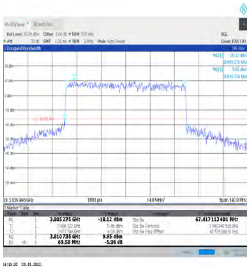
1-N77-3700-3980-PC3-30-70-M-8-CP-64QAM-Outer_Full-Outer_Full@N/A-Ant1-67.417-69.580-≤70-PAS
