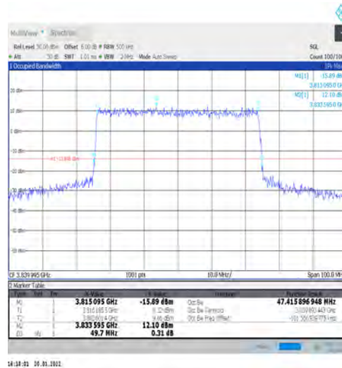
1-N77-3700-3980-PC3-30-50-M-7-CP-16QAM-Outer_Full-133@0-Ant1-47.416-49.700-≤50-PASS
