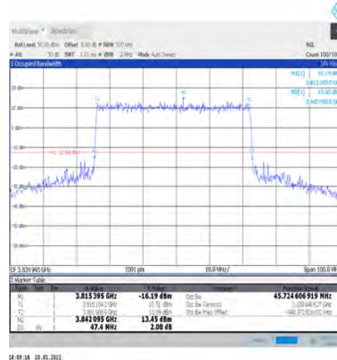
1-N77-3700-3980-PC3-30-50-M-3-DFT-16QAM-Outer_Full-128@0-Ant1-45.725-47.400-≤50-PASS
