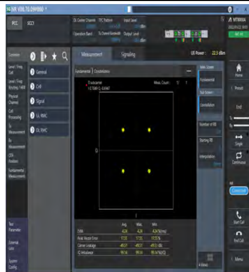
1-N77-3700-3980-PC3-30-100-M-6-CP-QPSK-Outer_Full-273@0-Ant1-see graph-PASS
