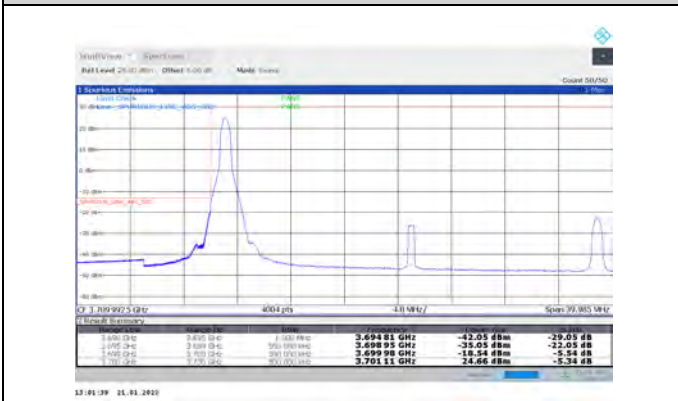
1-N77-3700-3980-PC3-30-30-L-1-DFT-PI2BPSK-Edge_1RB_Left-1@0-Ant1-PASS-see graph
