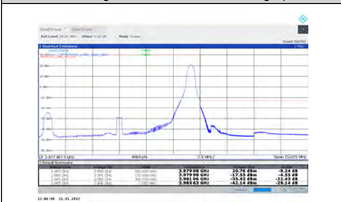
1-N77-3700-3980-PC3-30-15-H-5-CP-QPSK-Edge_1R_B_Right-1@37-Ant1-PASS-see graph
