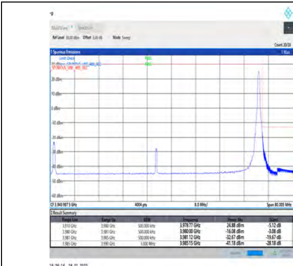
1-N77-3700-3980-PC3-30-70-H-2-DFT-PI2BPSK-Edge_e_1RB_Right-1@188-Ant1-PASS-see graph
