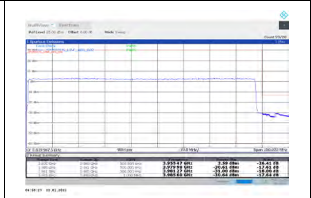
1-N77-3700-3980-PC3-30-90-H-3-DFT-PI2BPSK-Outer_Full-240@0-Ant1-PASS-see graph
