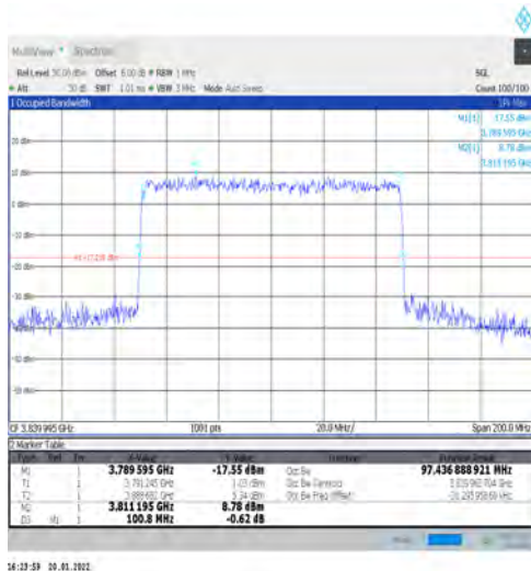
1-N77-3700-3980-PC3-30-100-M-9-CP-256QAM-Outer_Full-273@0-Ant1-97.437-100.800-≤100-PASS
