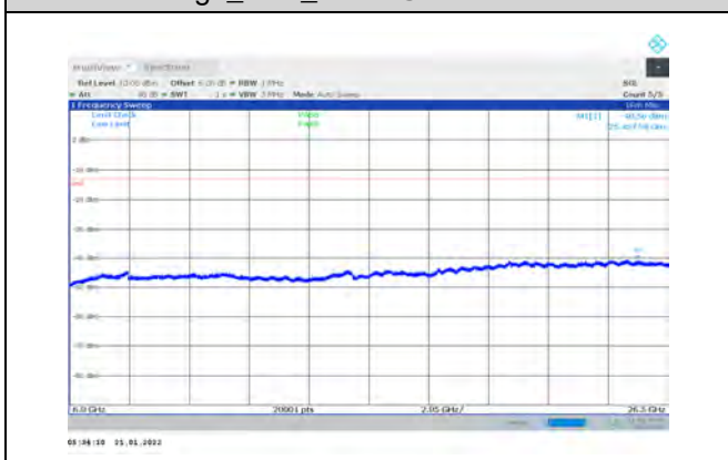
1-N77-3700-3980-PC3-30-100-M-1-DFT-PI2BPSK-E dge_1RB_Left-1@0-6000-26500
