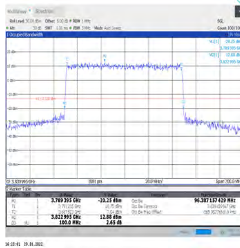
1-N77-3700-3980-PC3-30-100-M-4-DFT-64QAM-Ou ter_Full-270@0-Ant1-96.387-100.000-≤100-PASS
