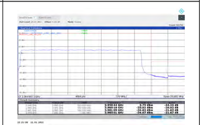
1-N77-3700-3980-PC3-30-40-H-3-DFT-PI2BPSK-Outer_Full-100@0-Ant1-PASS-see graph
