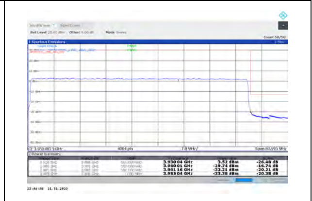
1-N77-3700-3980-PC3-30-60-H-3-DFT-PI2BPSK-Outer_Full-162@0-Ant1-PASS-see graph
