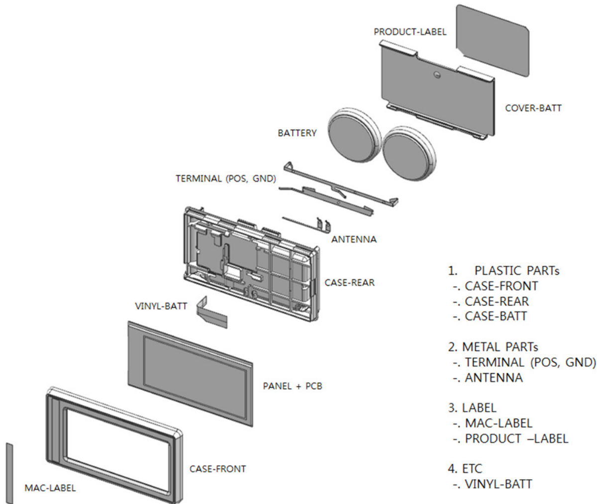
Figure 4 Exploded View
