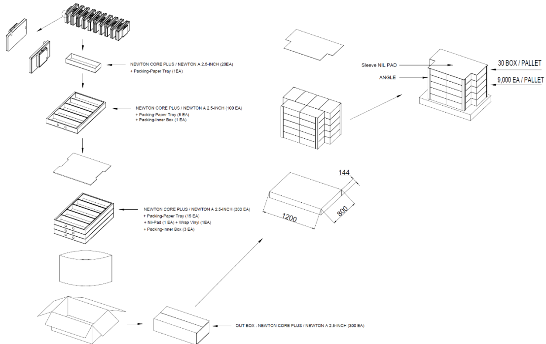
Figure 14. 2.5" PACKING-DIAGRAM (1,200 X 800)
