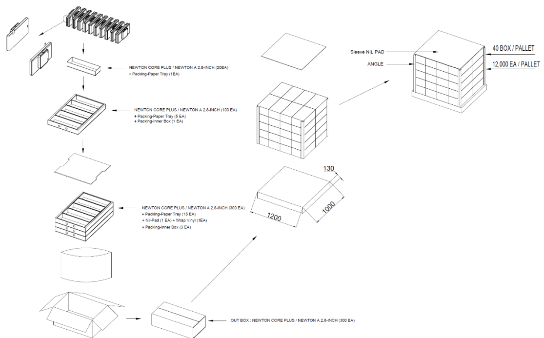
Figure 17. 2.8" PACKING-DIAGRAM (1,200 X 1,000)
