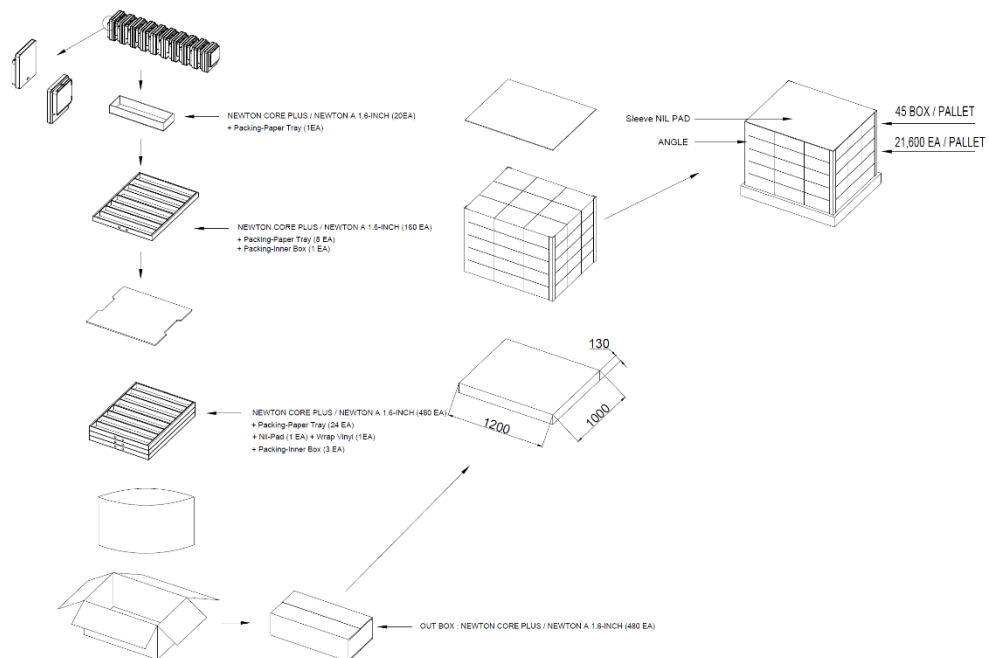
Figure 11. 1.6" PACKING-DIAGRAM (1,200 X 1,000)
