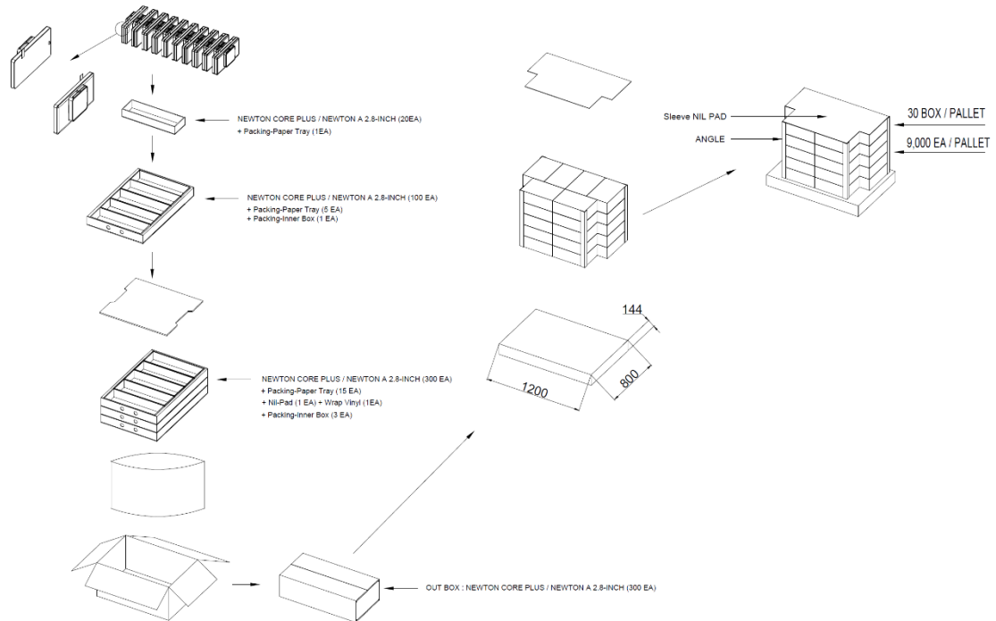
Figure 16. 2.8" PACKING-DIAGRAM (1,200 X 800)
