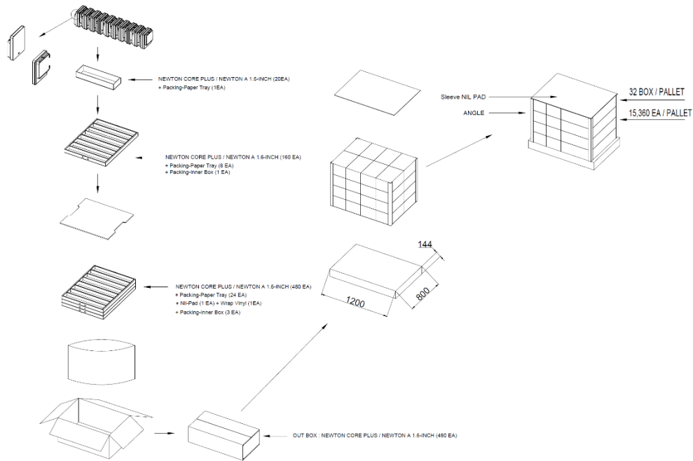
Figure 10. 1.6" PACKING-DIAGRAM (1,200 X 800)
