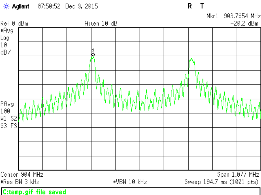
904 MHz – PSD
