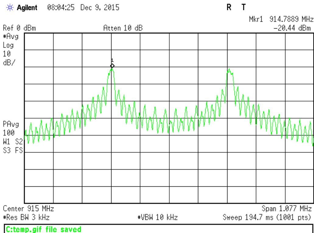
915 MHz – PSD
