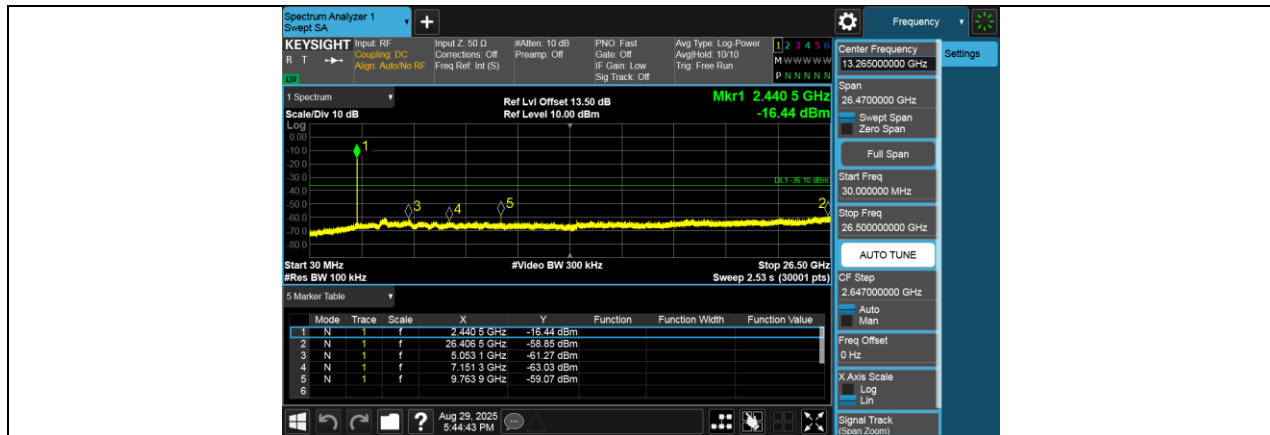
Tx. Spurious NVNT GFSK 2441MHz Ant1 Emission
