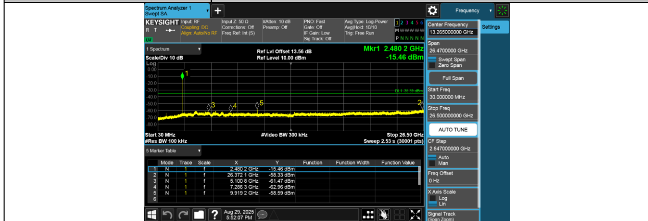
Tx. Spurious NVNT GFSK 2480MHz Ant1 Emission
