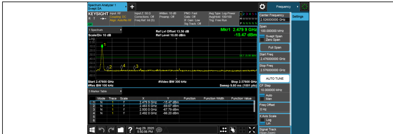
Band Edge NVNT GFSK 2480MHz Ant1 No-Hopping Emission
