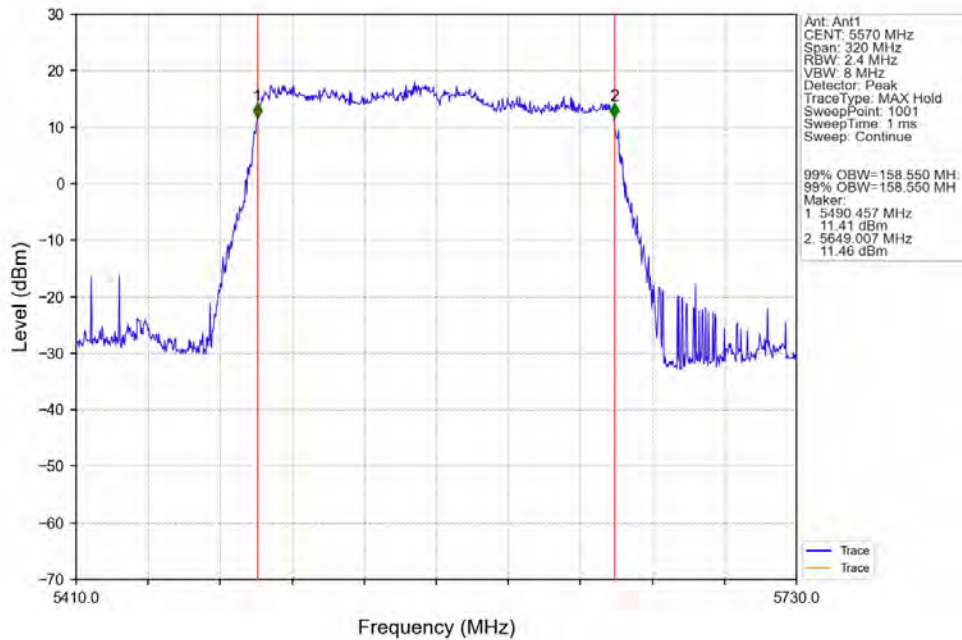
802.11ax(HEW160)_MCH_5570MHz_SU_ / _Ant1_NTNV
