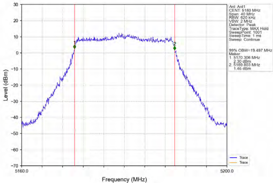
802.11ax(HEW20)_LCH_5180MHz_SU_ / _Ant1_NTNV
