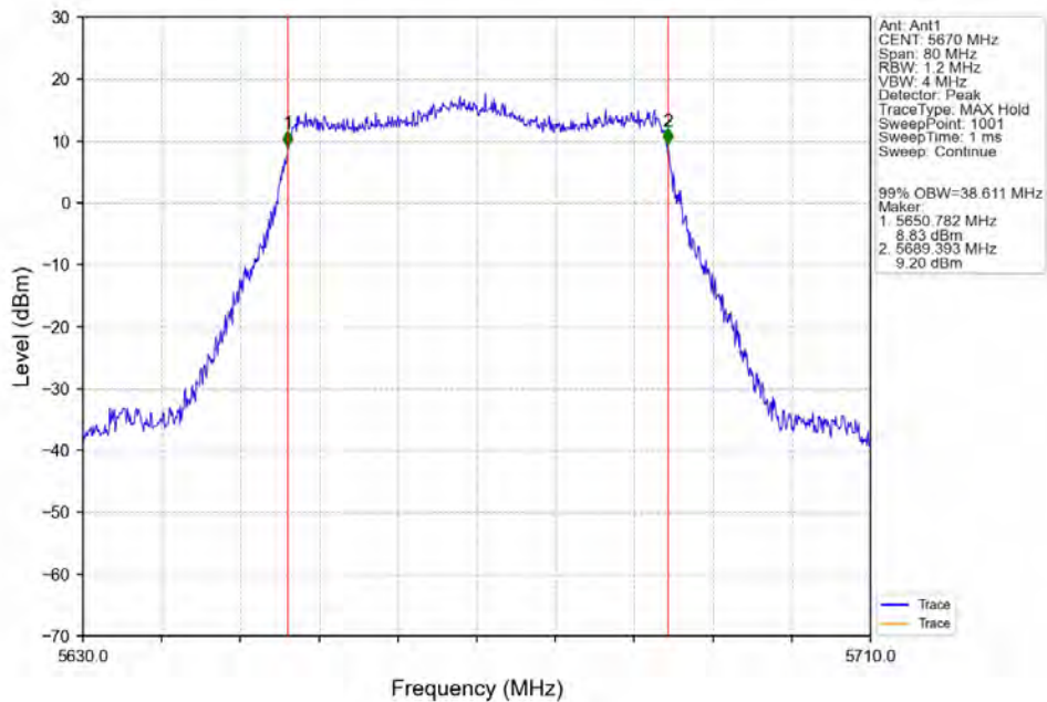
802.11ax(HEW40)_HCH_5670MHz_SU_ / _Ant1_NTNV
