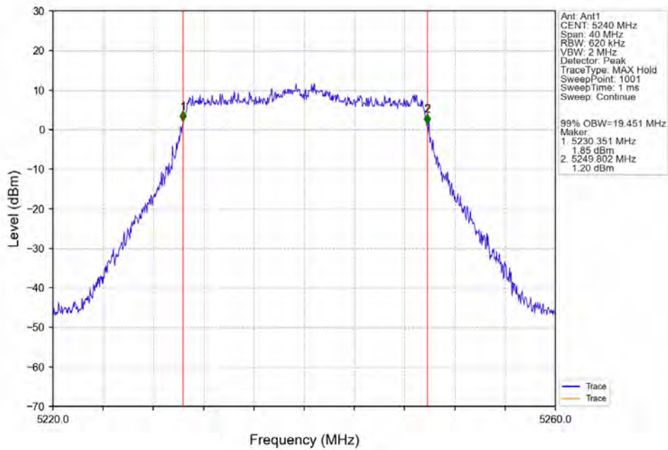
802.11ax(HEW20)_HCH_5240MHz_SU_ / _Ant1_NTNV
