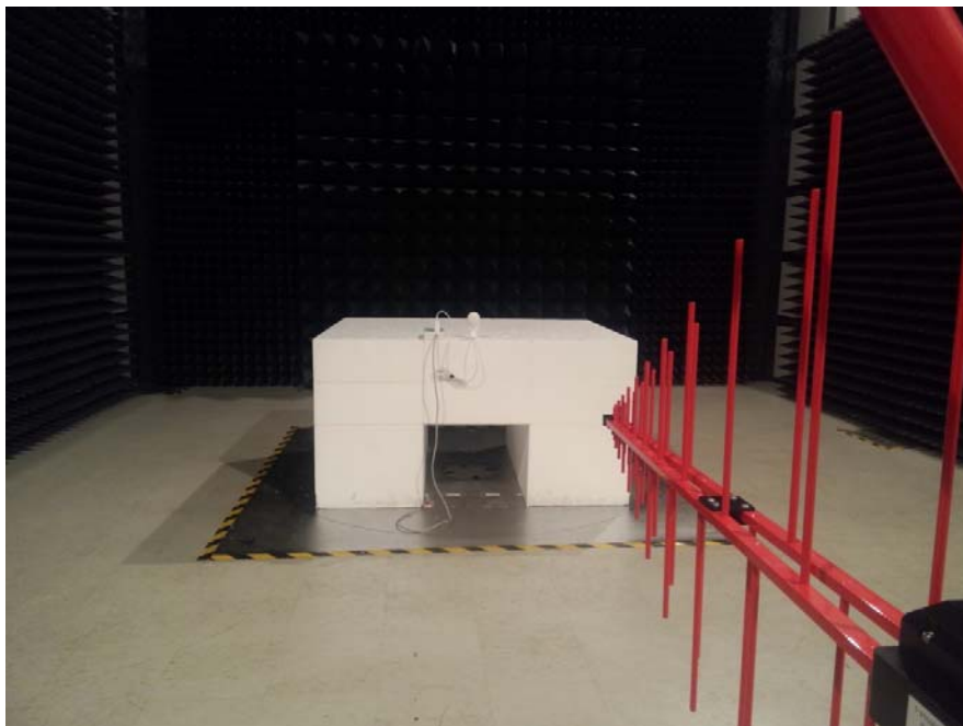
Radiated Spurious Emissions-Rear View (Below 1GHz)
