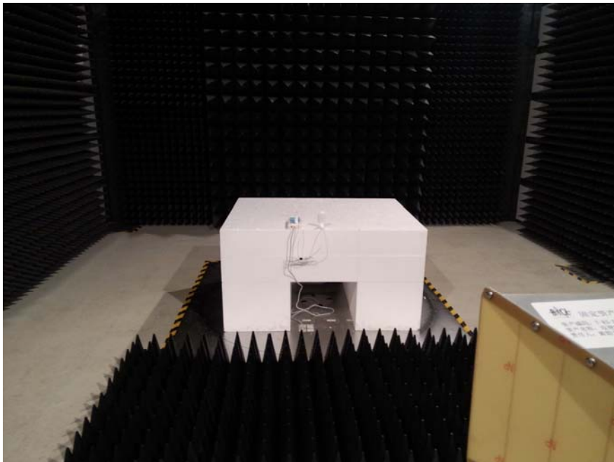
Radiated Spurious Emissions-Rear View (Above 1GHz)
