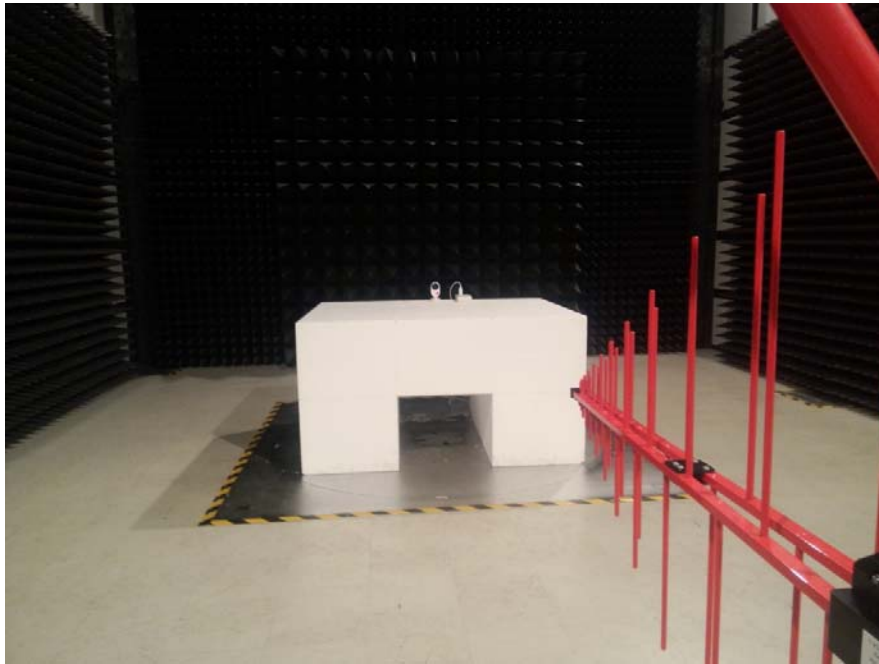
Radiated Spurious Emissions-Front View (Below 1GHz)
