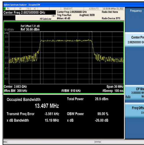
Band41-15MHz-QPSK-41515-75RB#0-13.497
