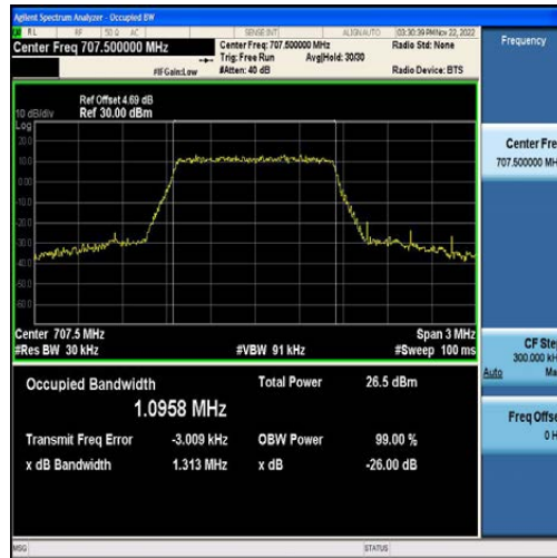
Band12-1.4MHz-16QAM-23095-6RB#0-1.0958
