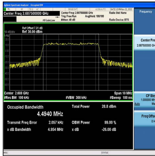
Band41-5MHz-QPSK-41565-25RB#0-4.4940
