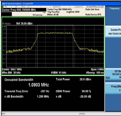
Band12-1.4MHz-QPSK-23017-6RB#0-1.0903
