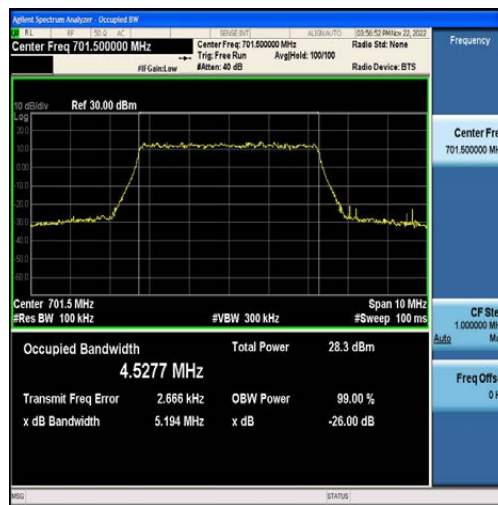
Band12-5MHz-QPSK-23035-25RB#0-4.5277
