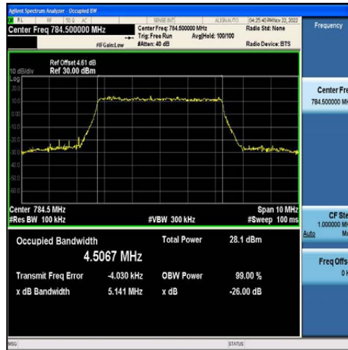
Band13-5MHz-QPSK-23255-25RB#0-4.5067
