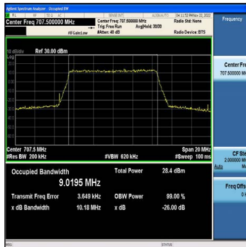
Band12-10MHz-QPSK-23095-50RB#0-9.0195
