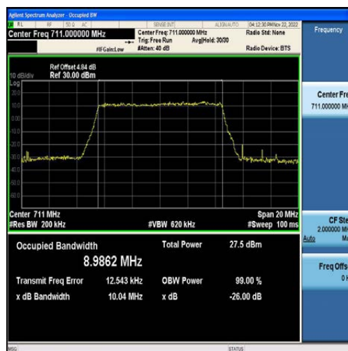
Band12-10MHz-16QAM-23130-50RB#0-8.9862
