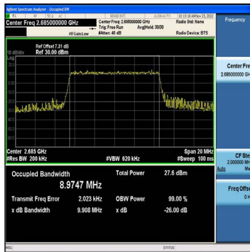
Band41-10MHz-16QAM-41540-50RB#0-8.9747
