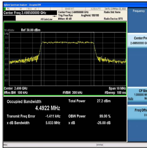
Band41-5MHz-16QAM-39675-25RB#0-4.4922
