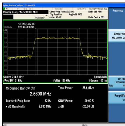
Band12-3MHz-16QAM-23165-15RB#0-2.6800
