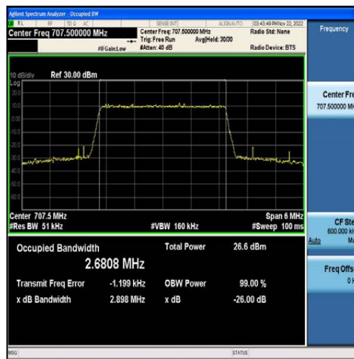
Band12-3MHz-16QAM-23095-15RB#0-2.6808
