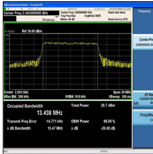
Band41-15MHz-QPSK-40620-75RB#0-13.438
