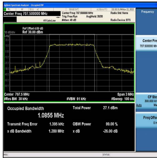
Band12-1.4MHz-QPSK-23095-6RB#0-1.0855
