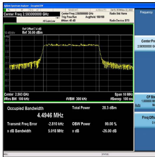
Band41-5MHz-QPSK-40620-25RB#0-4.4946
