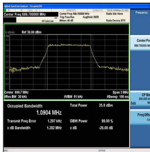
Band12-1.4MHz-16QAM-23017-6RB#0-1.0904
