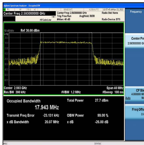
Band41-20MHz-16QAM-40620-100RB#0-17.943
