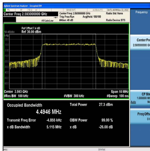
Band41-5MHz-16QAM-40620-25RB#0-4.4946
