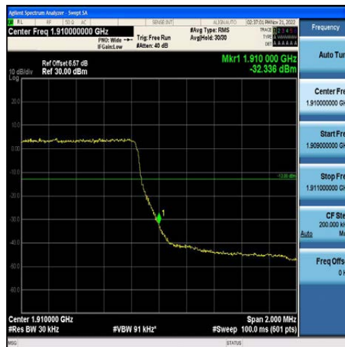
Band2-1.4MHz-QPSK-19193-6RB#0
