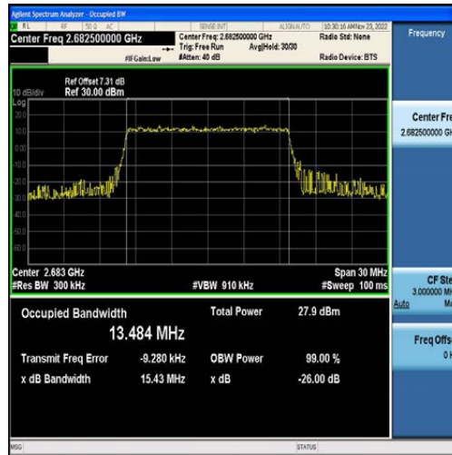
Band41-15MHz-16QAM-41515-75RB#0-13.484
