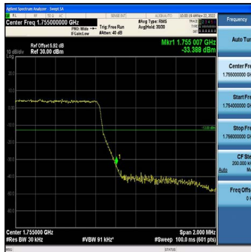
Band4-1.4MHz-QPSK-20393-6RB#0
