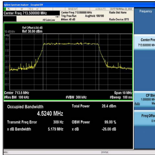
Band12-5MHz-QPSK-23155-25RB#0-4.5240
