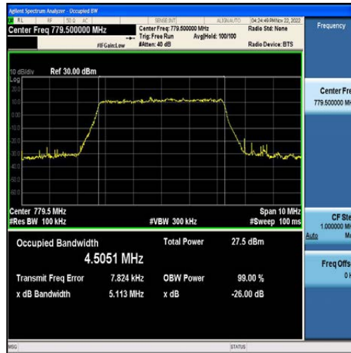
Band13-5MHz-16QAM-23205-25RB#0-4.5051
