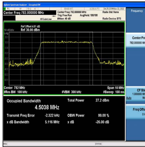
Band13-5MHz-16QAM-23230-25RB#0-4.5038
