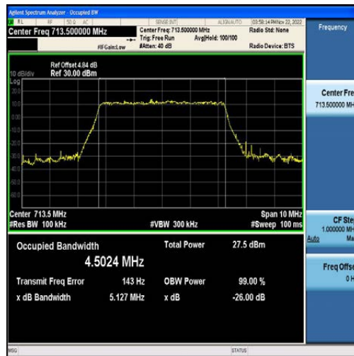
Band12-5MHz-16QAM-23155-25RB#0-4.5024
