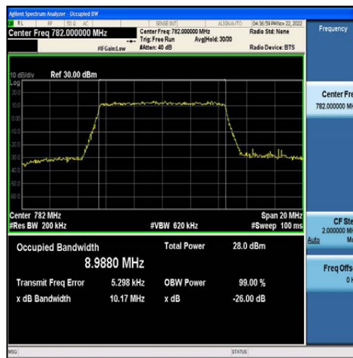
Band13-10MHz-QPSK-23230-50RB#0-8.9880
