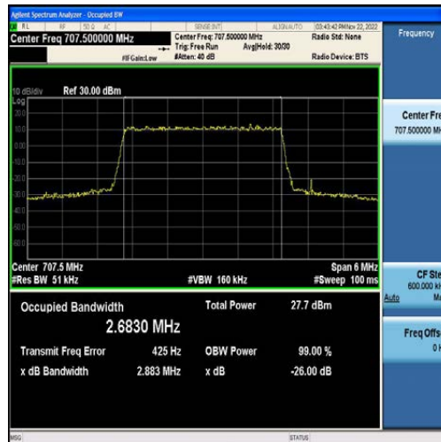
Band12-3MHz-QPSK-23095-15RB#0-2.6830
