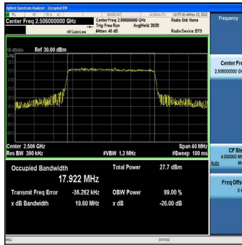
Band41-20MHz-16QAM-39750-100RB#0-17.922
