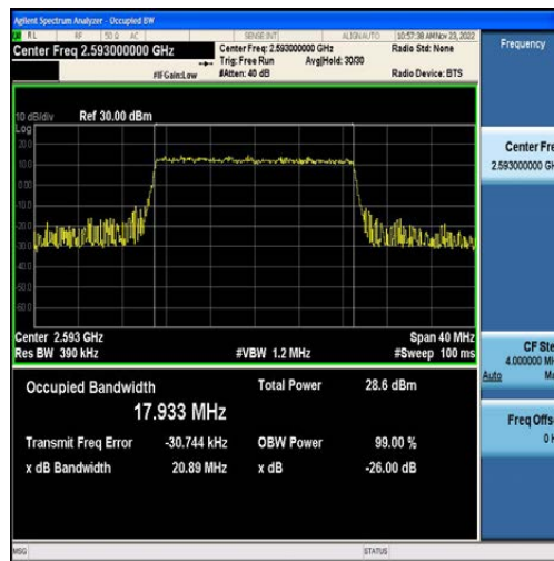
Band41-20MHz-QPSK-40620-100RB#0-17.933
