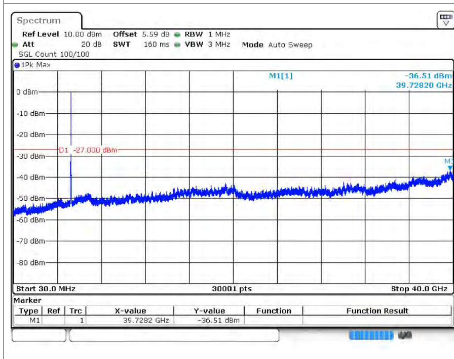
Tx. Spurious 5240MHz Ant1
