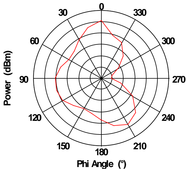
Fig. 3: 2402 MHz 3D Radiated pattern orientation of DUT compared to a phone.
