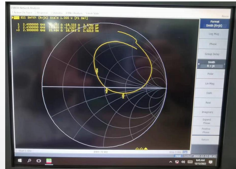
Smith-Chart
