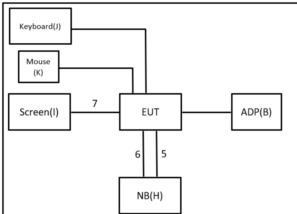
Radiated Emissions
