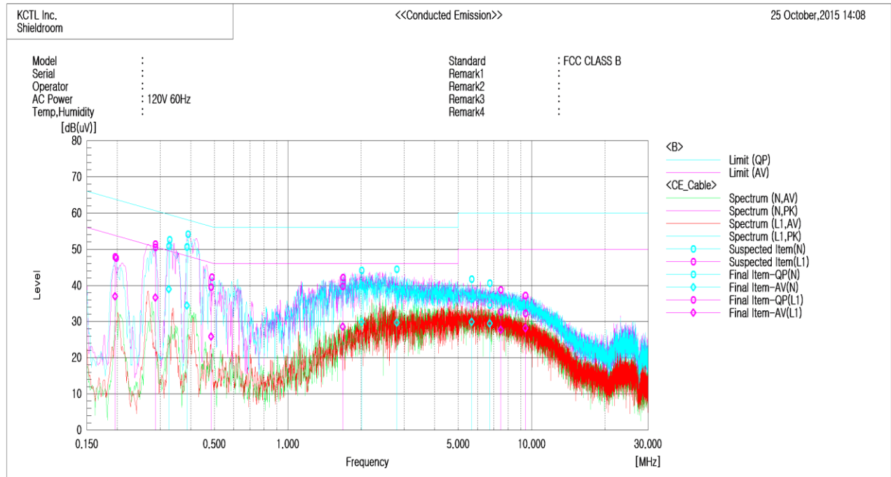
Figure 4. plot of Conducted Emission
