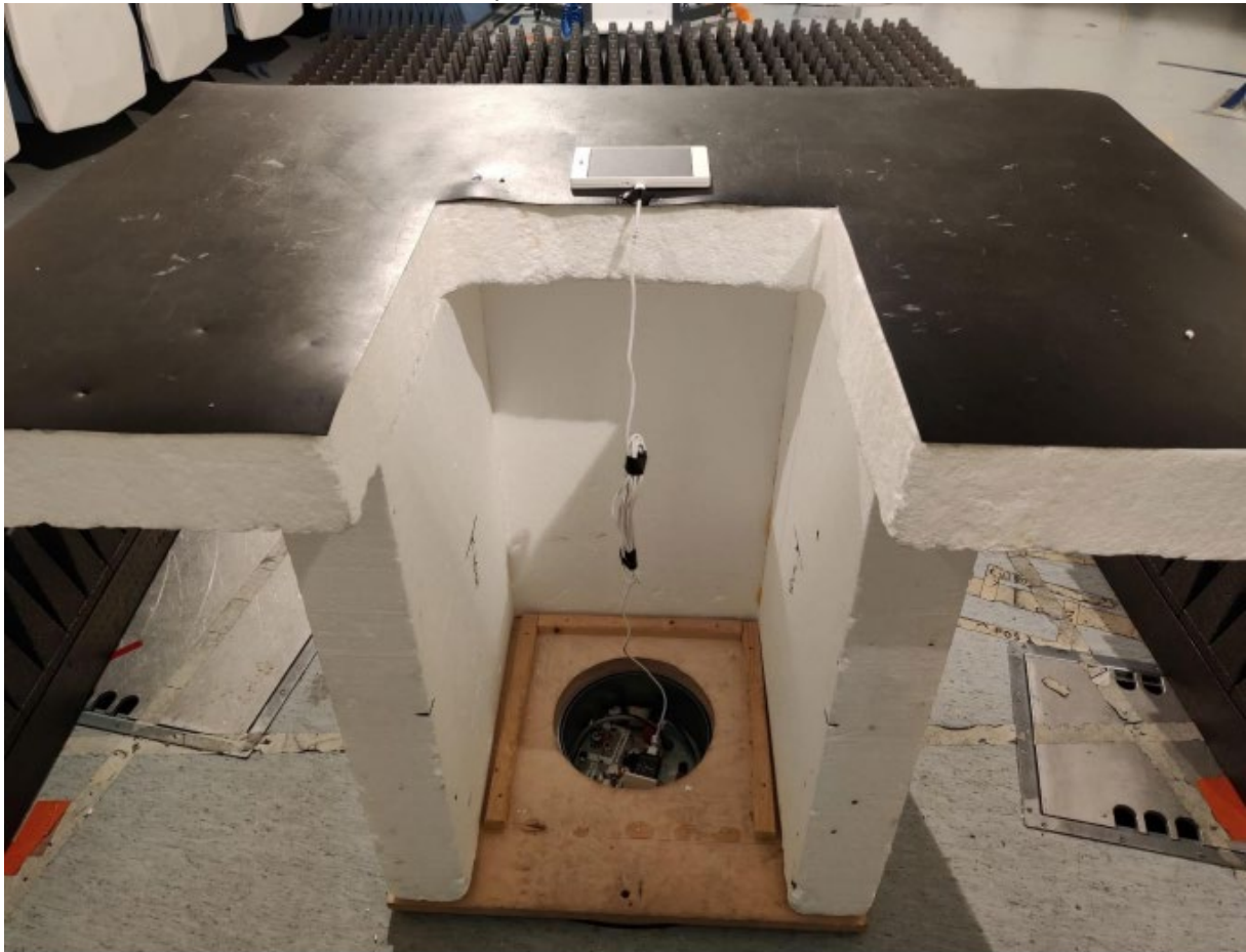
Radiated Spurious Emission, EUT setup, RX 1- 12,75 MHz
