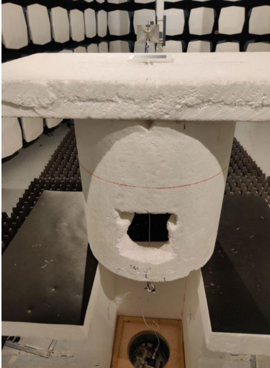
Radiated Spurious Emission, EUT setup, TX 1- 26 GHz
