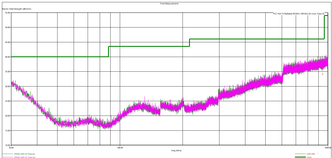
Figure 4 - Radiated Emissions Plot, Low Channel, Worst Case
