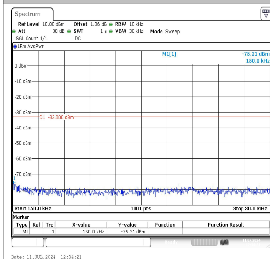
Band4_5MHz_16QAM_19975_1RB#0_0.15~30 0.15~30
