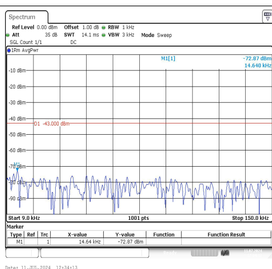
Band4_5MHz_16QAM_19975_1RB#0_0.009~0.15 _0.009~0.15
