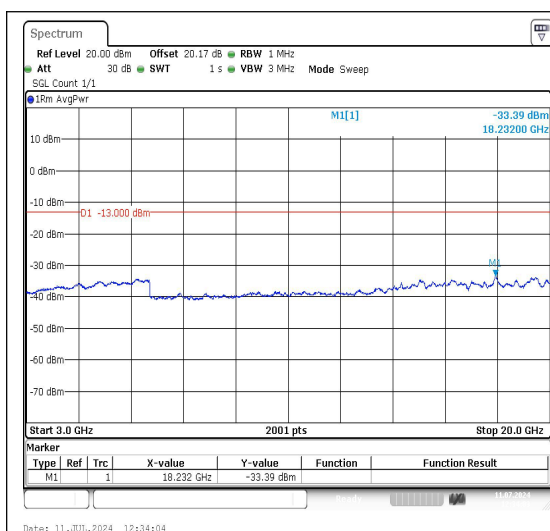
Band4_5MHz_QPSK_19975_1RB#0_3000~2000 0_3000~20000
