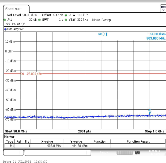
Band4_5MHz_16QAM_19975_1RB#0_30~1000_3 0~1000
