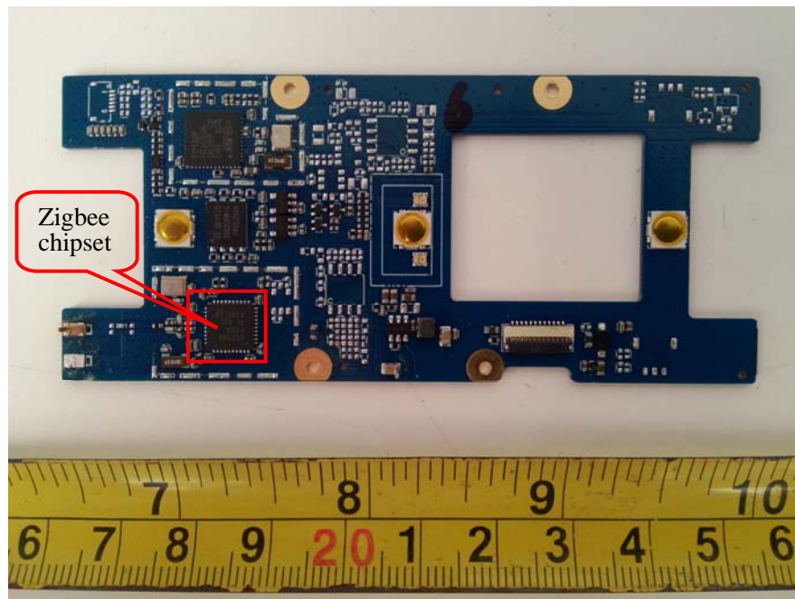
EUT – Main Board -2 Top shielding Cover off View
