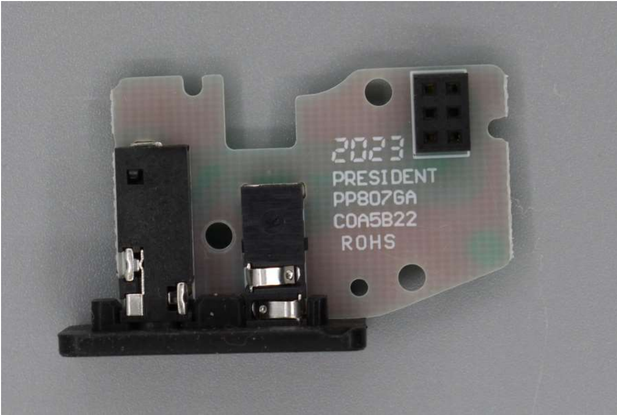
Figure E17.8 – Internal, Audio PCB, Top
