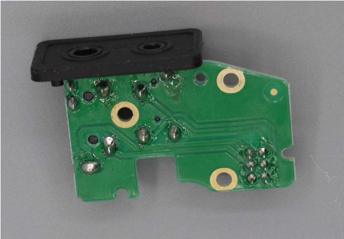
Figure E17.7 – Internal, Audio PCB, Bottom
