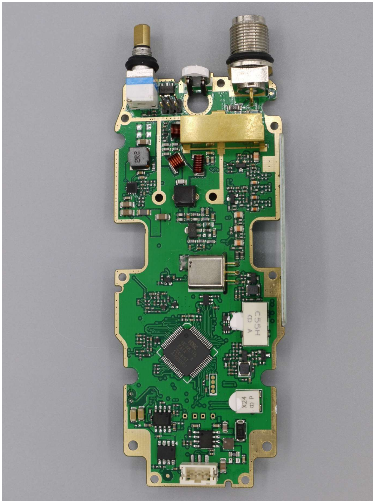
Figure E17.5 – Internal, Main PCB, Top
