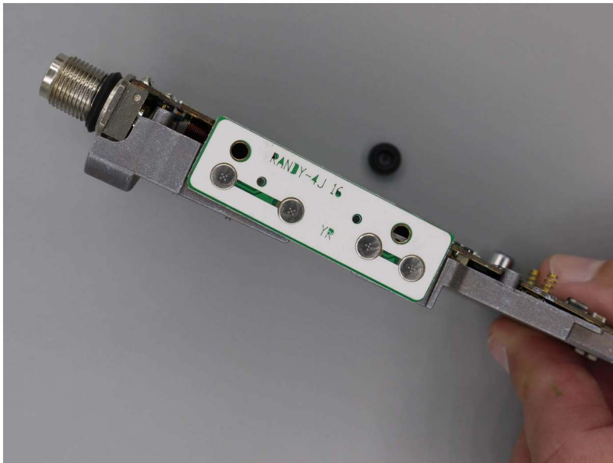
Figure E17.6 – Internal, Main PCB, Button Side
