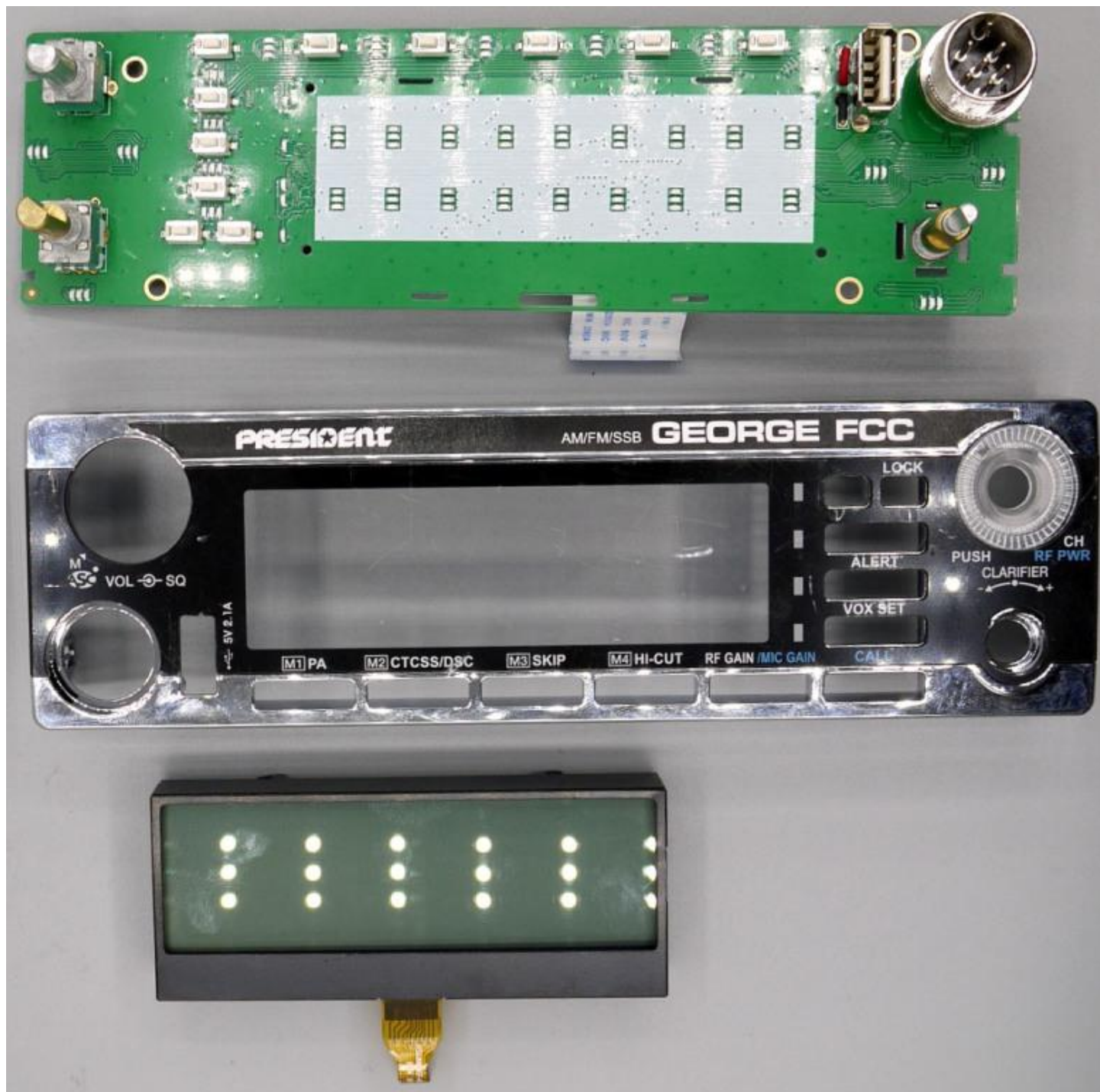
Figure E17.6 – Internal, Front Panel Components
