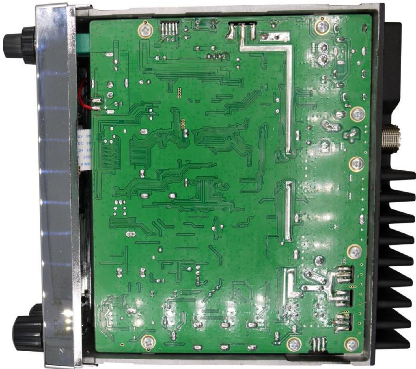
Figure E17.4 – Internal, Main PCB, Bottom Side
