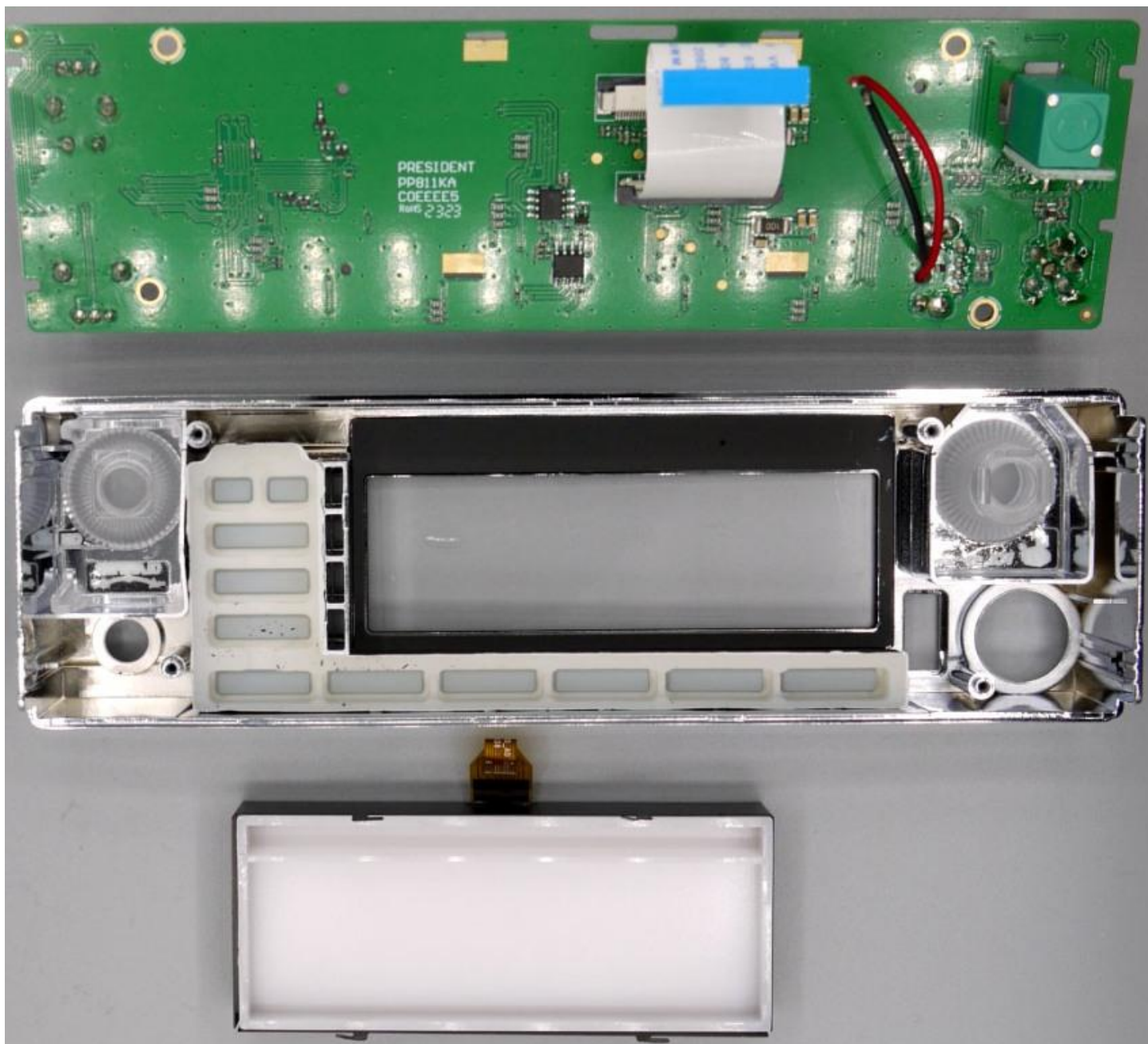
Figure E17.5 – Internal, Front Panel Components
