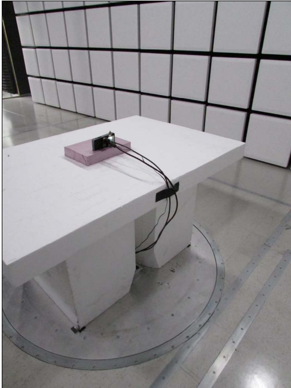
Figure 4: Back View – Below 1 GHz
