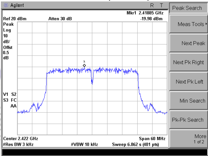
Channel 03 (2422MHz)
