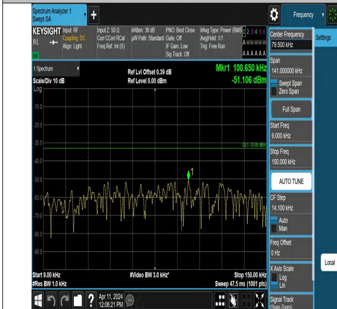
Band17_5MHz_QPSK_23825_1RB#0_0.009~0.15_0.009~0.15
