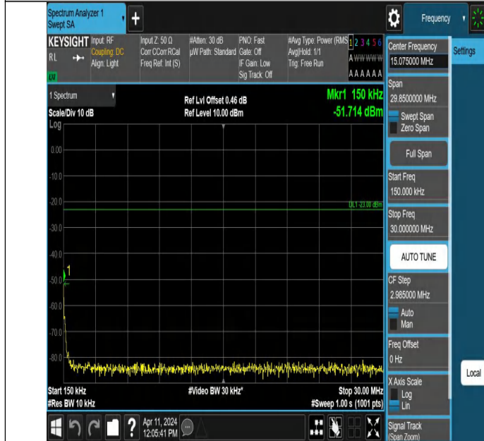
Band17_5MHz_QPSK_23790_1RB#0_0.15~30_0.15~30
