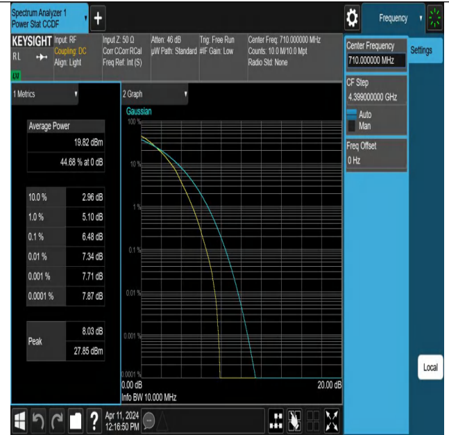
Band17-10MHz-64QAM-23790-50RB#0-PASS
