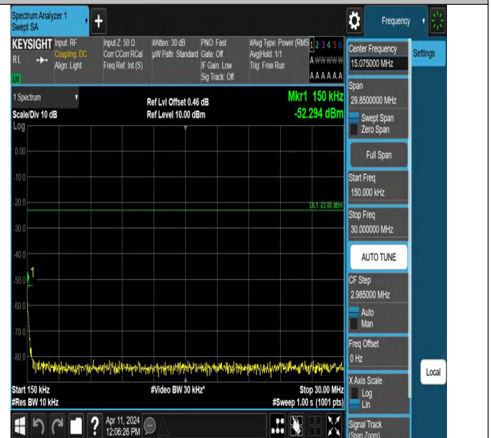
Band17_5MHz_QPSK_23825_1RB#0_0.15~30_0.15~30
